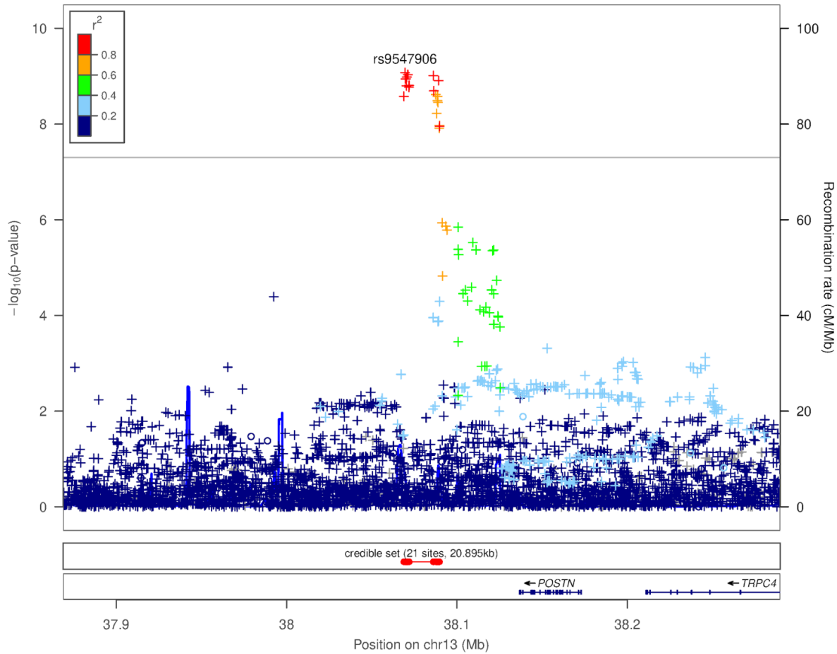
Figure 6: Locuszoom plot for spontaneous pneumothorax chromosome 13 association
