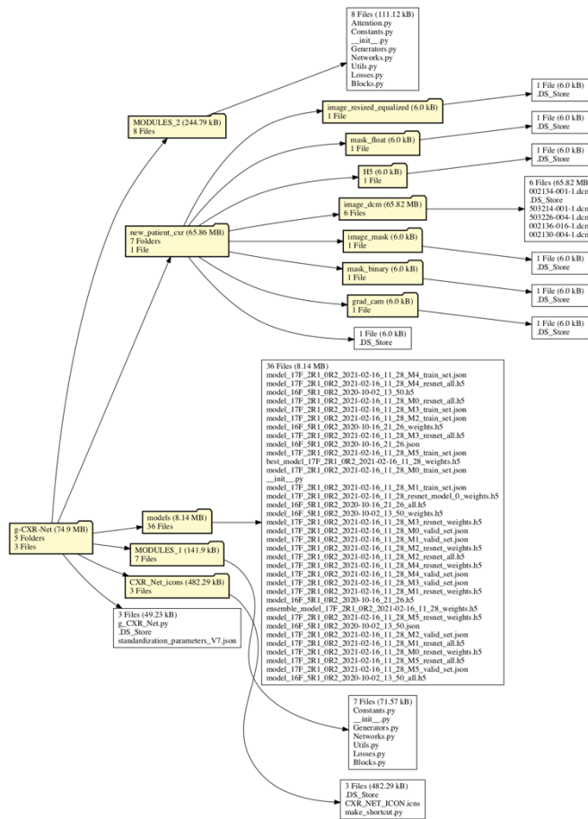
Fig. 1. g-CXR-Net tree. MODULES_I and MODULES_II folders contain all the modules necessary to build the underlying AI engine of CXR-Net. Trained CXR-Net models are in the models folder. The new_patient_cxr folder contains both the source directory for CXR images in DCM format, and the target directories where g-CXR-Net stores CXR images converted from DCM to PNG format, intermediate files in H5 format used for classification, the binary and floating point lung masks generated by CXR-Net Module I, and the heat maps, displaying the lung regions with potential SARS-CoV-2 lesions, generated by CXR-Net Module II. The folder CXR_Net_icons contains an example icon for the application, and a python script that can be used to generate an icon link to g_CXR_Net.py anywhere in the OS tree.
