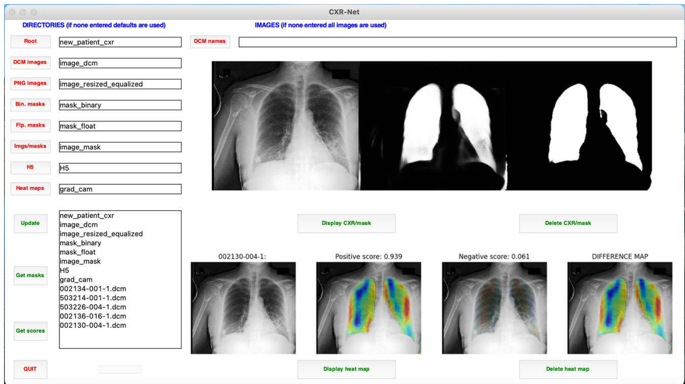
Fig. 2. g-CXR-Net GUI. Buttons are associated with different actions: a) select a directory tree for sources and targets different from the default one, b) select CXR images to be processed, c) update selections, d) calculate lung masks, e) calculate classification scores, f) calculate heat maps, g) display CXRs and corresponding floating point and binary lung masks, h) display heat maps, i) quit. Updates and task results are displayed in the text window at the lower left corner of the GUI.
