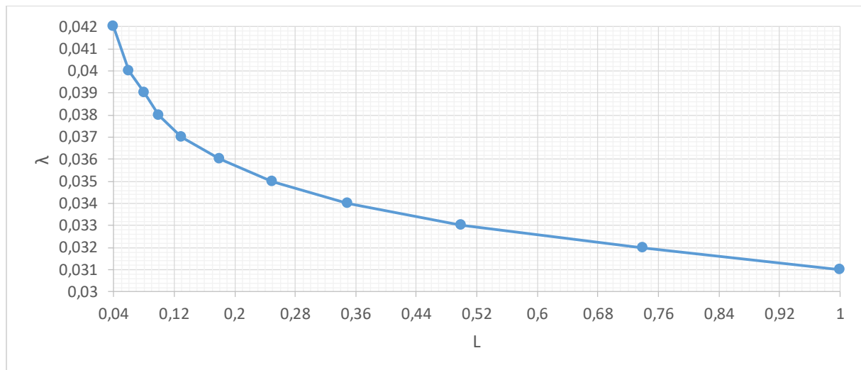
Figure 1 Dependence of the model coefficient \lambda on the lockdown efficiency L
