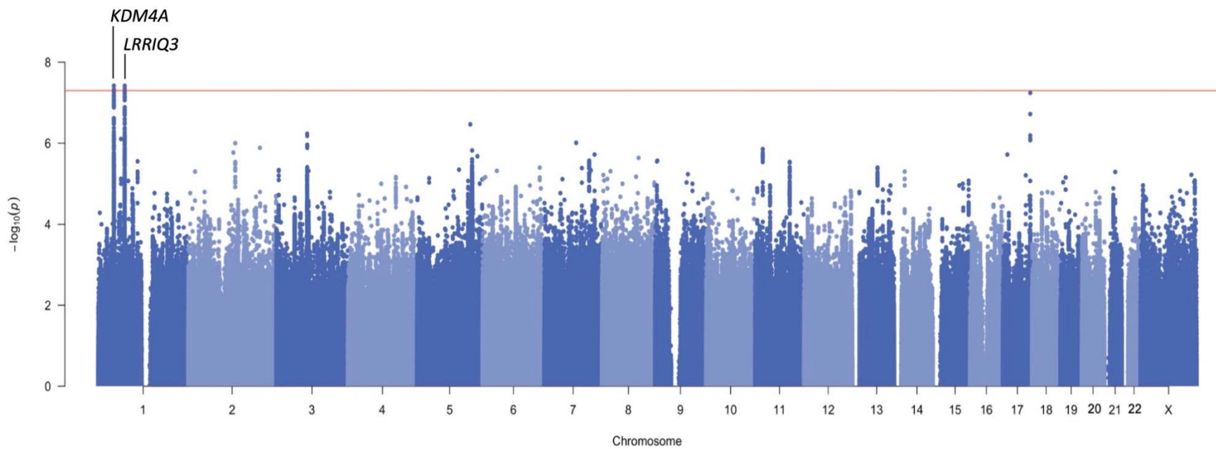
Figure 1. Genome-wide association analysis for problematic opioid use. The nearest genes are labeled for the 2 lead SNPs (rs3791033, rs640561). The x-axis shows chromosomal position and the y-axis shows significance on -\log_{10} scale. The horizontal red line denotes genome-wide significance ( p=5.00E-08 ).
