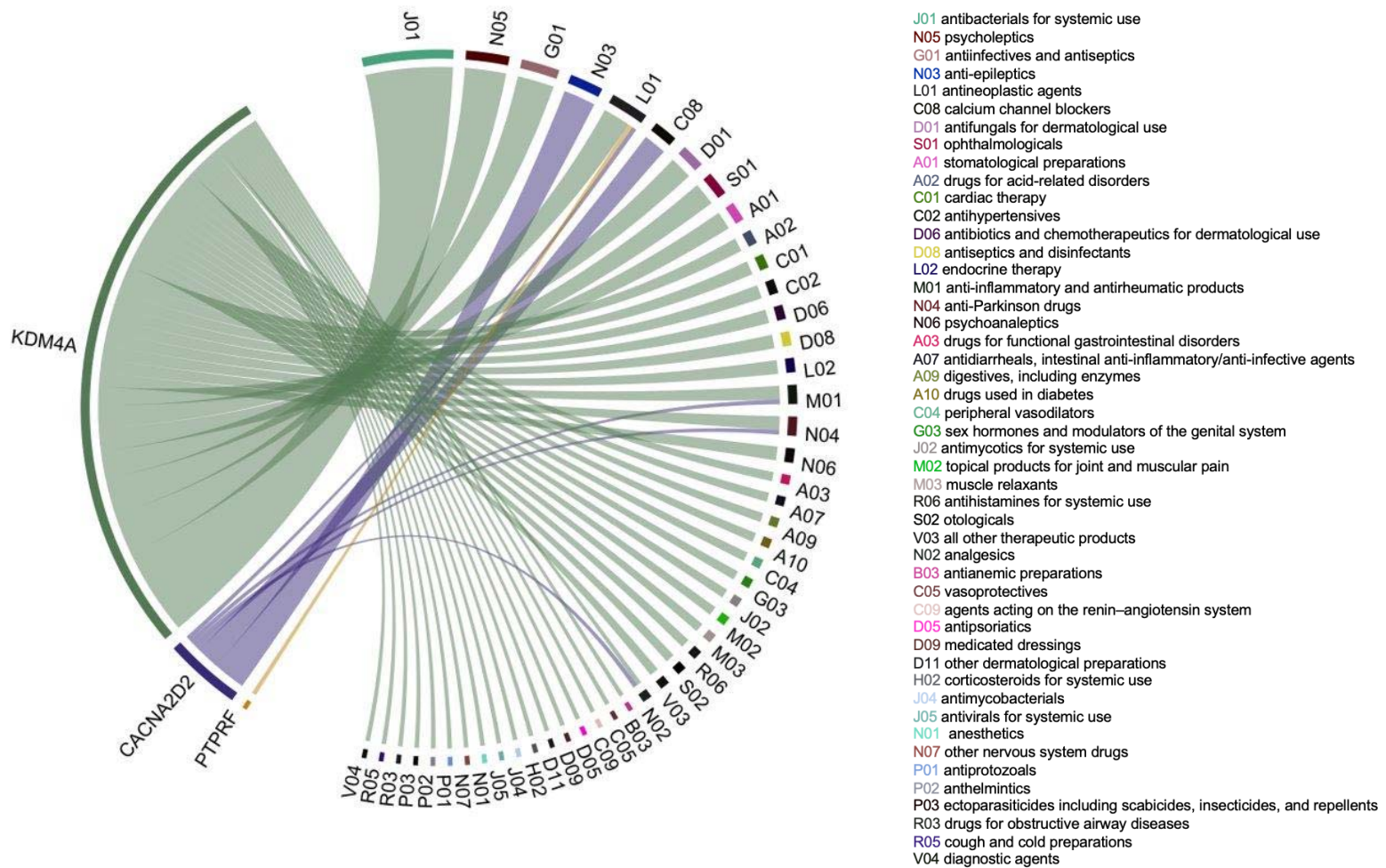
Figure 4. Chord diagram of genes significantly associated with POU at 10% FDR and the Anatomical Therapeutic Chemical classifications of drugs. The width of each line is determined by the number of drugs known to interact with each gene.
