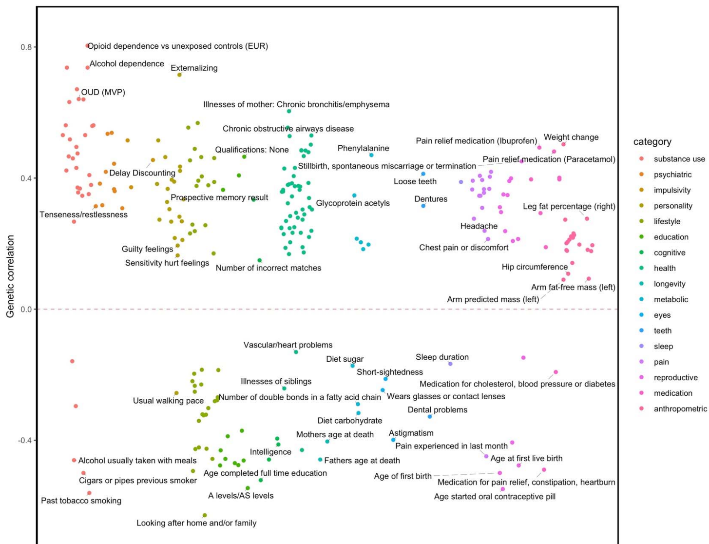
Figure 2. LDSC FDR-significant genetic correlations with POU. Traits with positive genetic correlation ( r_g ) values are plotted above the line; traits with negative r_g values are plotted below the line. All traits surpass 5% FDR correction for multiple testing.
