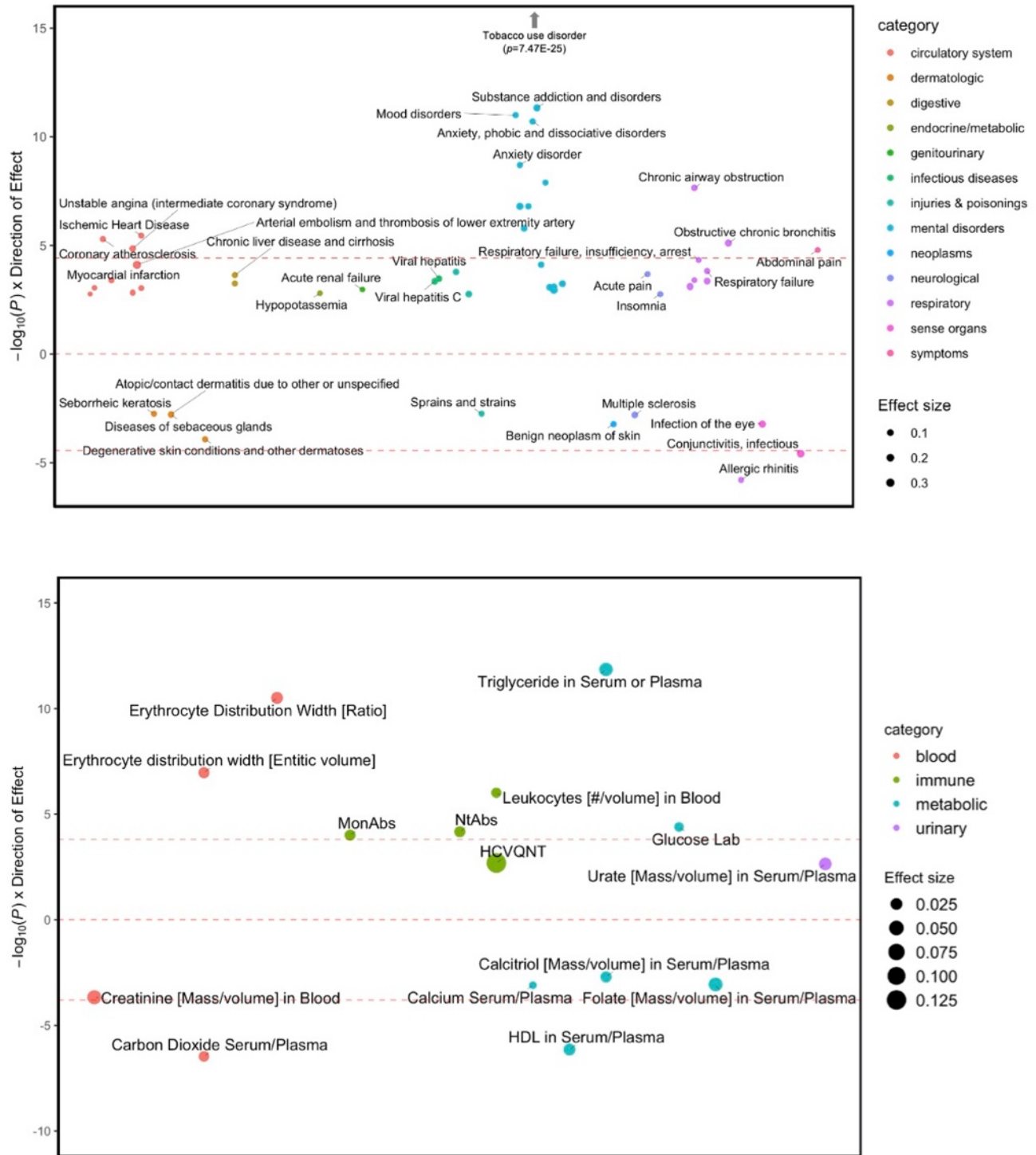
Figure 5. Phenome-wide (top) and lab-wide (bottom) association studies of polygenic risk scores for POU against 1,338 diseases and 315 biomarkers (respectively) available from BioVU. The top and bottom red dashed lines indicate the threshold for Bonferroni correction (PheWAS p=3.74E-05 ; LabWAS p=1.59E-04 ). Only FDR significant results are presented. The sizes of the dots correspond to the magnitude of the effect. Y axis represents the negative logarithm of the p-value for each trait multiplied by the sign of the effect.
