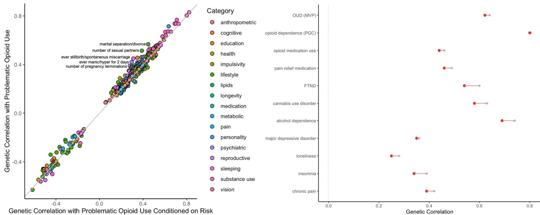
Figure 3. Genetic correlations ( r_g ) with POU before and after conditioning on risk-taking behavior. All FDR-significant results are plotted on the left panel, selected relevant traits are shown on the right panel (original r_g in grey; corrected r_g in red). The top 5 traits with biggest change in r_g value are labelled (left).
