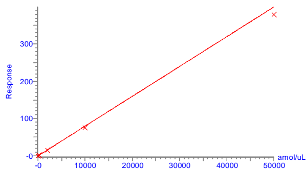
Supplementary Figure 2. Calibration curve for ADETQALPQR over the range 3-50,000 amol/ \mu L
