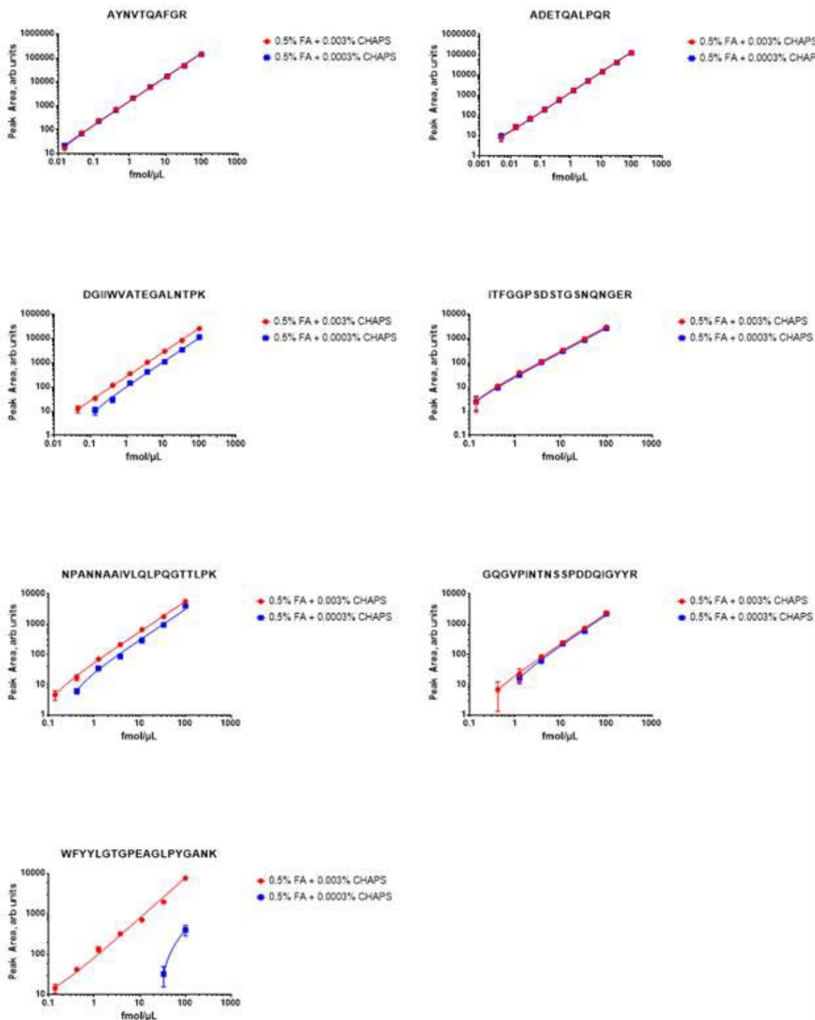
Supplementary Figure 1. Peak area (MRM sensitivity) SIL ( ^{13}\text{C}_6^{15}\text{N}_2 C-terminal K or ^{13}\text{C}_6^{15}\text{N}_4 C-terminal R labeled) NCAP peptides as function of peptide and detergent (CHAPS) concentration.
