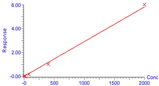
Supplementary Figure 4. Calibration curve for DGIWVATEGALNTPK over the range 3-2,000 amol/μL
