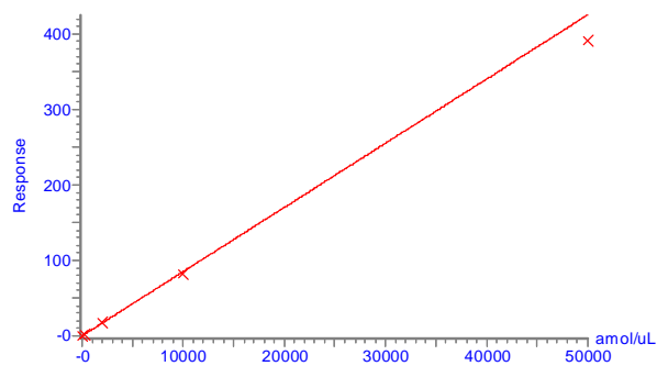
Supplementary Figure 3. Calibration curve for NPANNAIIVLQLPQGTTLPK over the range 3-50,000 amol/ \mu L
