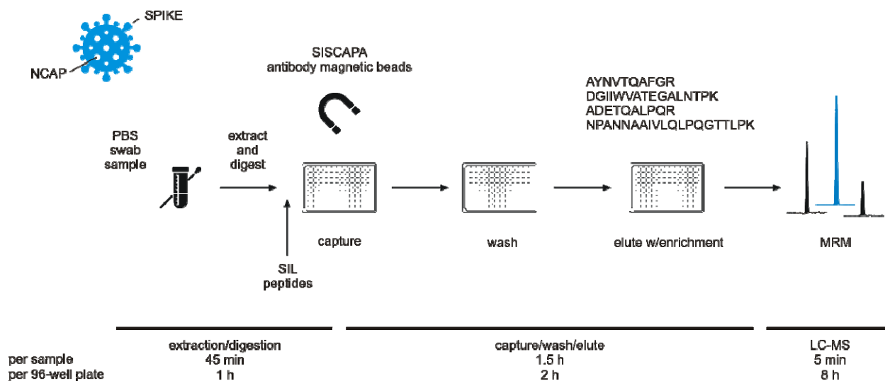
Figure 1. Experimental workflow for immuno-affinity peptide (SISCAPA) enrichment LC-MS of NCAP SARS-CoV-2 peptides. Swab sample extracts were subjected to tryptic digestion, SIL standards added to the tryptic digest solution, and magnetic beads coupled with specific anti-peptide antibodies incubated to allow binding of the peptides. Unbound peptides are removed and the target peptides eluted and measured using MRM analysis with LC-MS.
