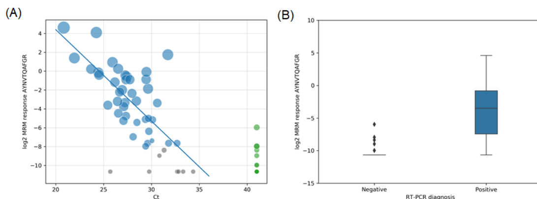
Figure 3. LC-MS ( \log_2 quantifier response) vs. RT-PCR (Ct) read-out correlation (A) and quartiles distribution of the LC-MS results (B) . Color labeling is based on RT-PCR diagnoses (green = negative SARS-Cov-2; blue = positive SARS-CoV-2); grey = not detected or inconclusively identified by LC-MS.
