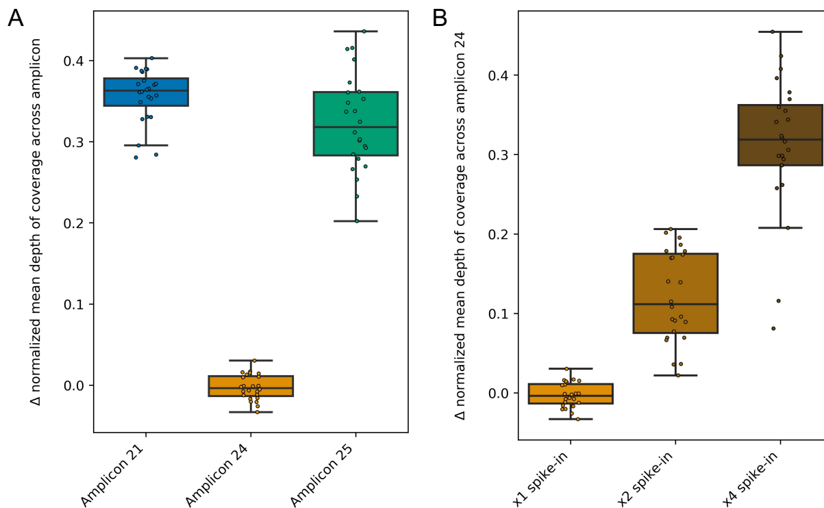
Figure 2: Amplicon drop-out is corrected by spiking updated primers into Freed et al. primer scheme. Updated primers were designed for problematic amplicons based on the primer site variant sequences identified by PCR_strainer in Table 1. Freed primer pools with and without these updated primers were used to sequence 24 P.1 lineage clinical specimens. Mean depths of coverage across each amplicon were calculated and normalized to each library's most deeply sequenced amplicon. These paired data were used to calculate changes in normalized mean depths of coverage across amplicons. A) Depth of coverage was significantly improved for amplicons 21 and 25 by spiking the updated primers into the Freed pool at one-times molarity (p-values < 0.00001, paired sample T-test). B) Depth of coverage across amplicon 24 was significantly improved when the updated primer was spiked into the Freed pool at two- and four-times molarity (p-values < 0.00001, paired sample T-test).
