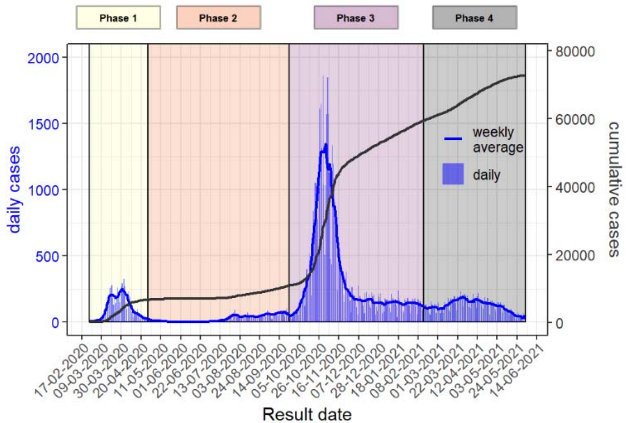
Figure 1 , Epidemic Curve of the cases of Coronavirus Disease 2019 (COVID-19) in Geneva state, February 26, 2020 – June 1st, 2021. Vertical bars represent the daily cases (based on the date of the test result), solid blue line represents the weekly moving average and the solid black line the cumulative cases.
