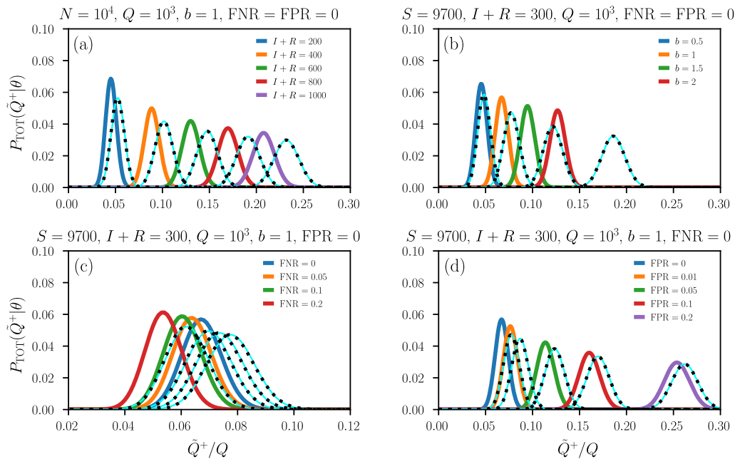
Figure 2. Distribution of apparently positive tests. Plots of P_{TOT}(\tilde{Q}^+ = q|Q, I, S, R, b) with N = S + I + R = 10^4 , Q = 10^3 , and different (a) values of I + R , (b) testing biases b , (c) FNRs, and (d) FPRs. The Gaussian approximation (solid light blue lines) of Eq. 2.22 provides an accurate approximation of P_{TOT} . Dashed black lines correspond to distributions with replacement and the remaining solid colored lines correspond to those without replacement.
