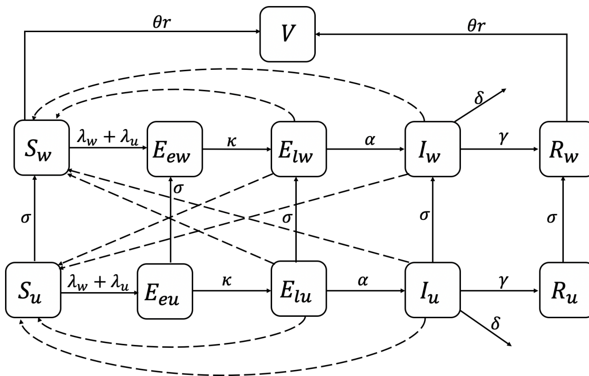
Figure 1: Schematic diagram of the COVID-19 model
