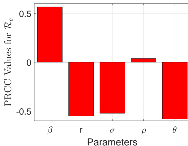
Figure 3: Partial rank correlation coefficients (PRCCs) showing the impact of model parameters on the reproduction number ( \mathcal{R}_c ) of the model. Parameter values used are as given in Table 3.
