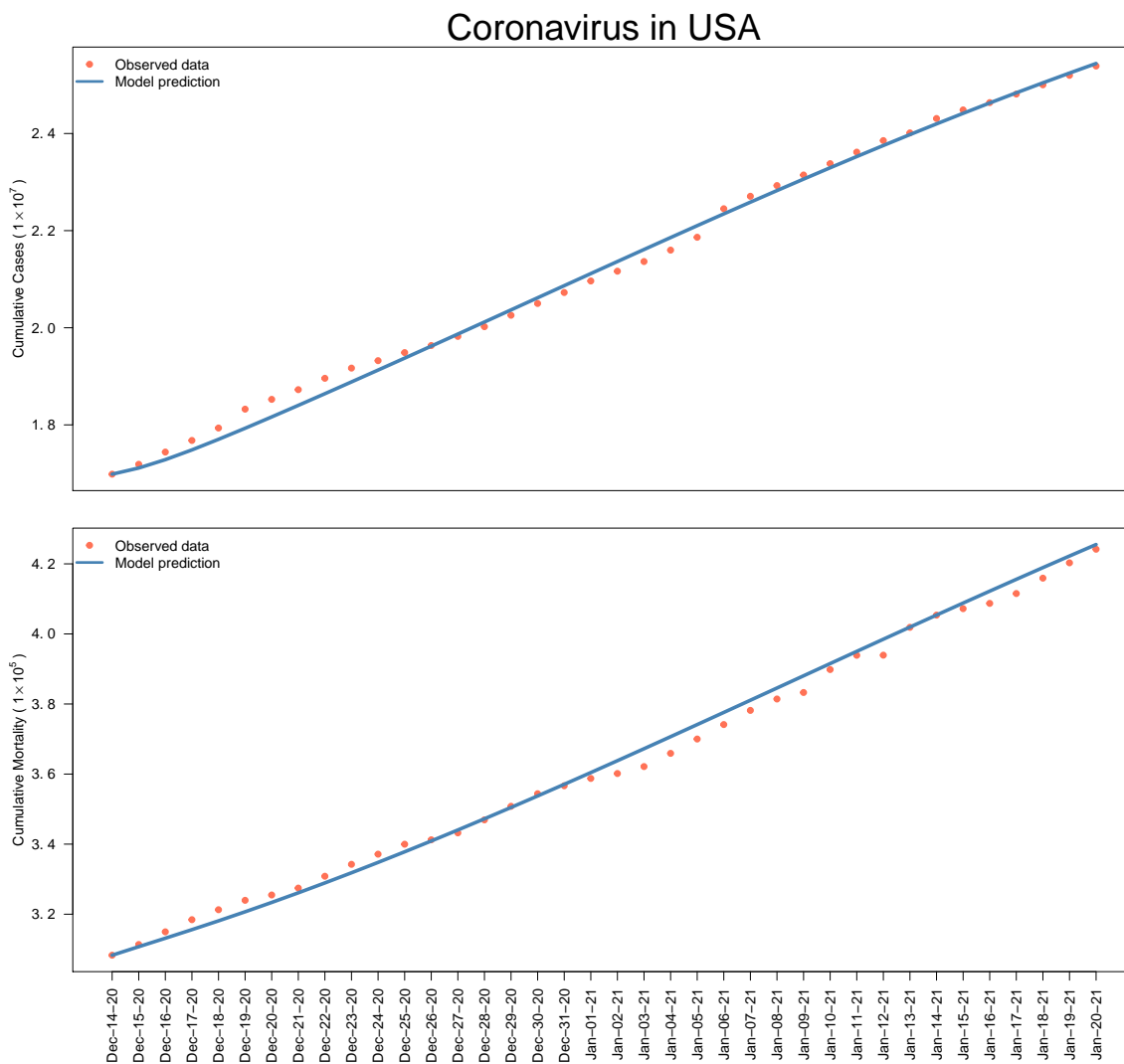
Figure 2: The fitted model and the observed COVID-19 cumulative cases and deaths in USA from December 14, 2020 to January 20, 2021
