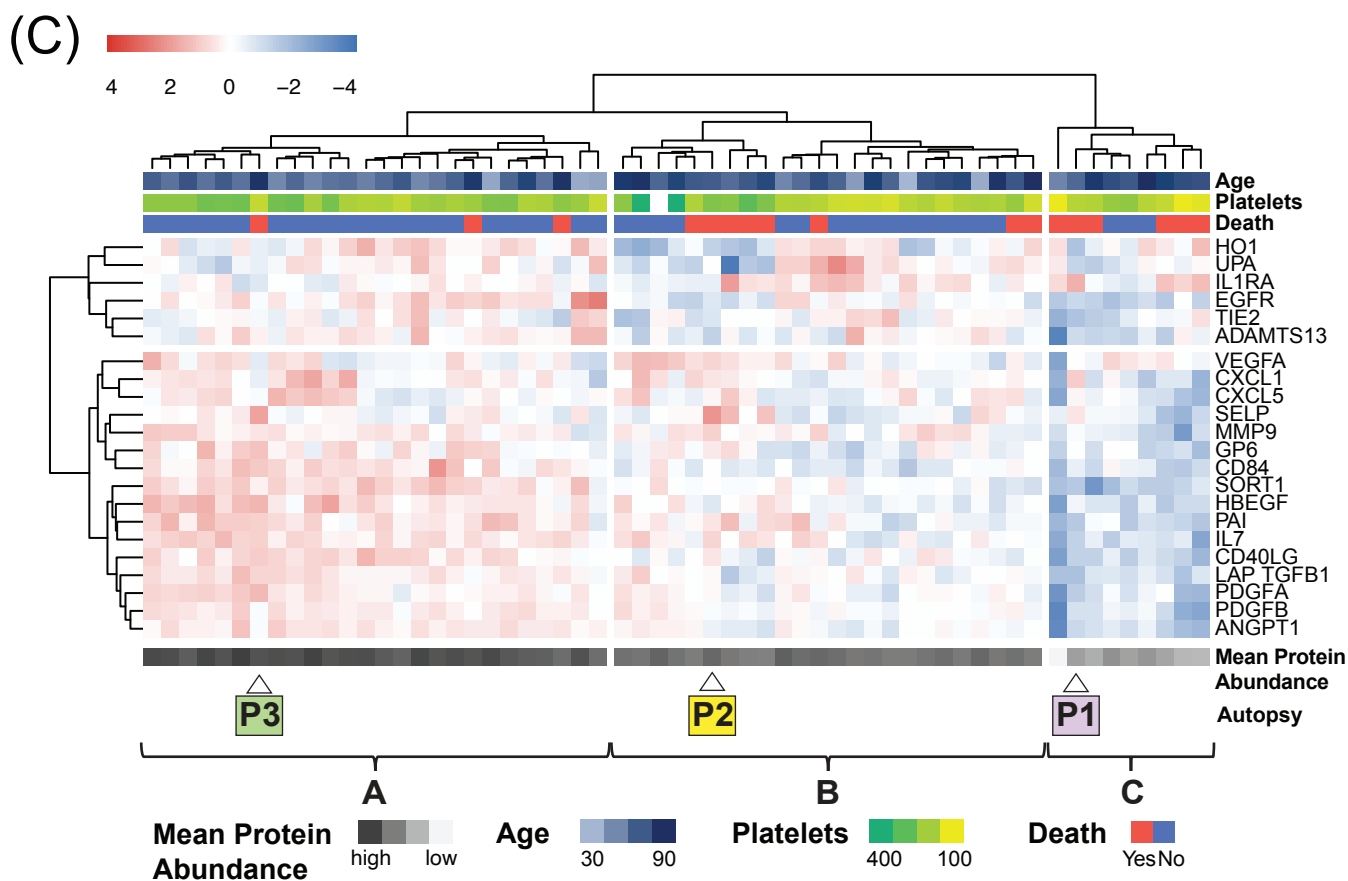
Figure 3: The hospitalized at risk cohort (N=59) blood proteome identifies a maladaptive vascular response preceding critical illness. (A) Overview of the associations of the protein set to death and platelets. P-values were obtained with a linear mixed effect model to account for repeated measurements and confounders and corrected for multiple comparisons (Padj). X and Y axes indicate the -\log_{10} of the adjusted p-value of the association of proteins to death and platelets, respectively. The protein labels signifies inclusion in the final protein set. (B) Box plots demonstrating the association between proteins of vascular junctional integrity, angiogenesis, platelet degranulation, and coagulopathy to mortality in the at risk cohort after adjusting for multiple comparisons. The boxes indicate the interquartile range (IQR) of the data distribution, the line in the box represents the median value and the whiskers extend for 1.5 times the value of the IQR. Dots indicate the protein level in individual patients. (C) Heatmap of protein set abundance in the at risk COVID-19 subjects. Hierarchical clustering was performed using Ward linkage and Euclidean distance. Age, platelet count and death are overlaid at the top. Mean abundance of the 22 protein set and autopsy cases identifiers (e.g. P1, P2, P3) are displayed at the bottom.
