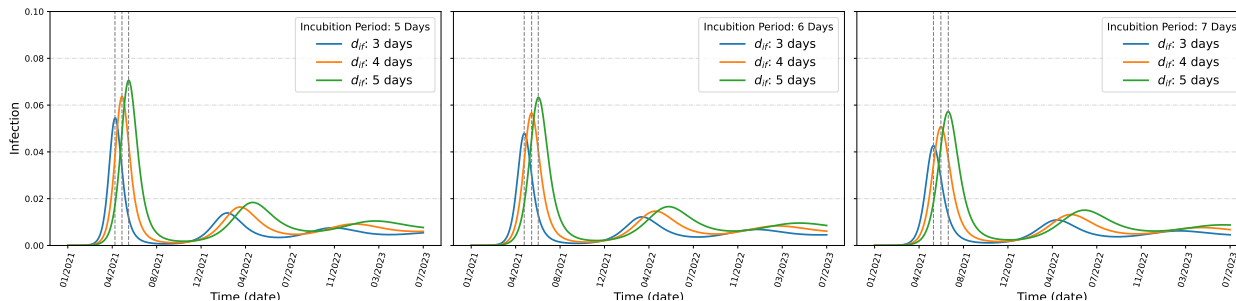
Figure 9: SVEIRD dynamics of Madhya Pradesh
