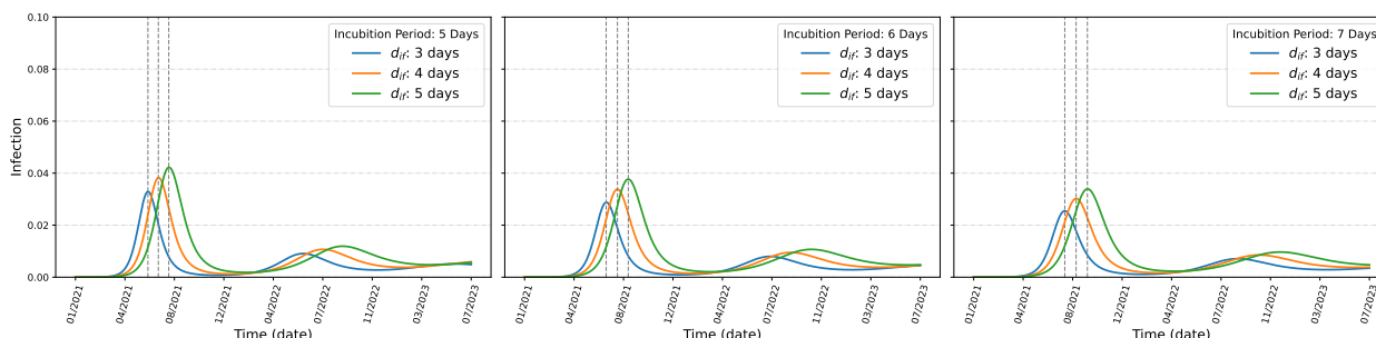
Figure 6: SVEIRD dynamics of Tamil Nadu
