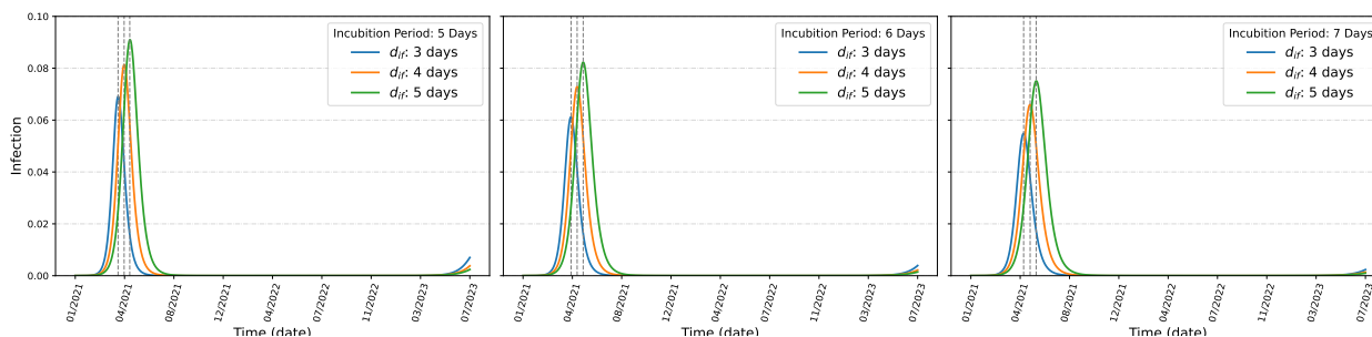
Figure 7: SVEIRD dynamics of Odisha
