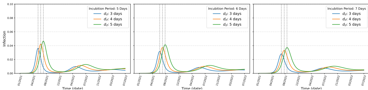
Figure 5: SVEIRD dynamics of Karnataka
