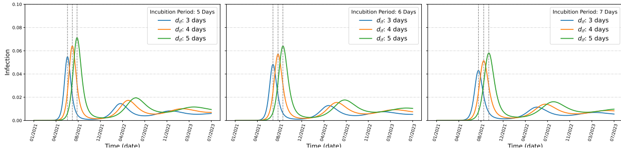
Figure 11: SVEIRD dynamics of India
