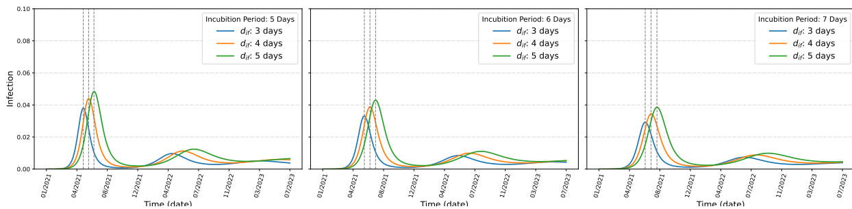
Figure 4: SVEIRD dynamics of Chhattisgarh
