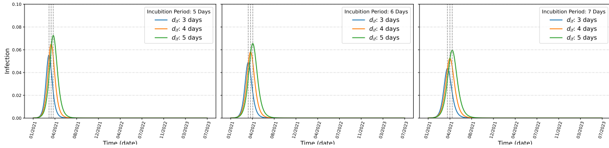
Figure 3: SVEIRD dynamics of Goa
