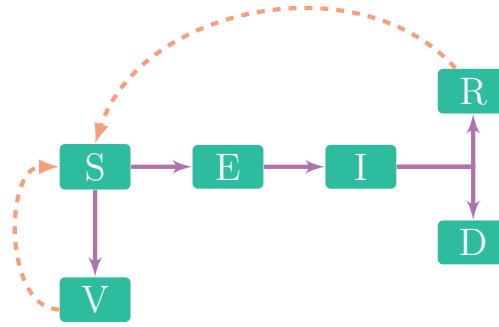
Figure 1: Dynamics of SVEIRD model
