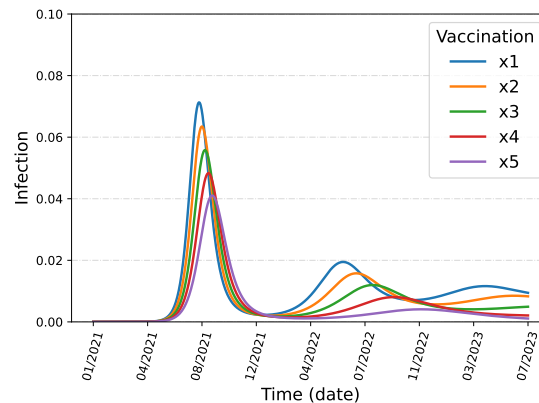
Figure 13: Change of SARS-CoV-2 infection with increase in vaccination rate in India. The line shows increase in rate of vaccination times the current rate. This is done for dynamics of India (Figure (11)) with incubation period 5 days and d_{if} 5 days.)
