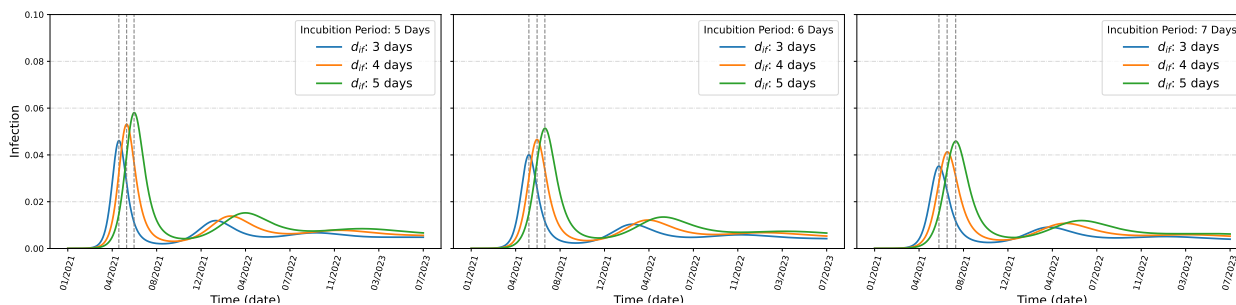
Figure 8: SVEIRD dynamics of Gujarat
