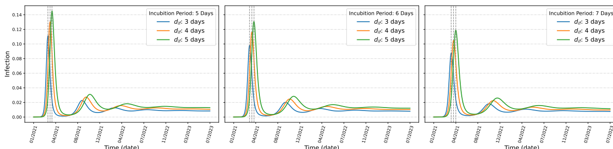
Figure 10: SVEIRD dynamics of Uttar Pradesh (Note the change of scale in y -axis)
