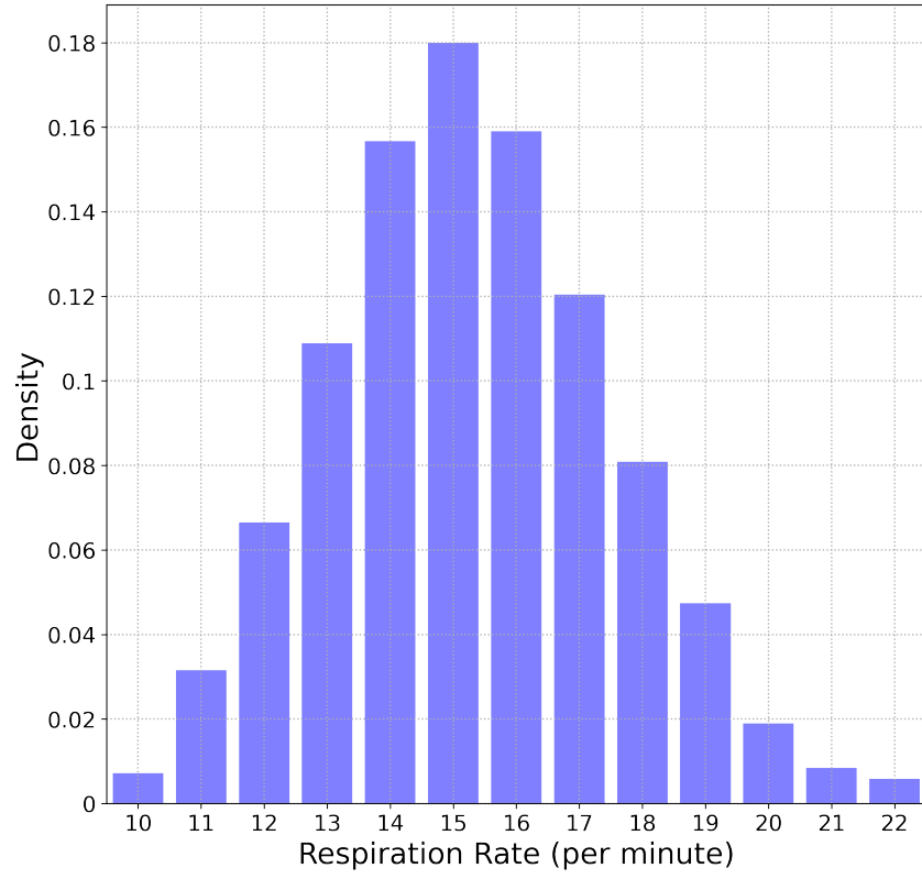
FIG. 3. Distribution of respiratory rates. 90% of values are between 11.8 - 19.2 min -1 .
