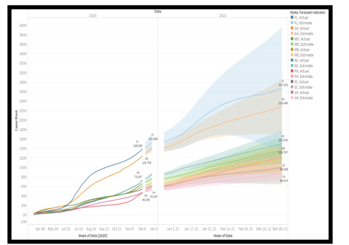
Figure 8. Holt-Winter exponential forecast of Black COVID 19 Cases in FL, GA, MD, NC, SC, MS, PA and VA
