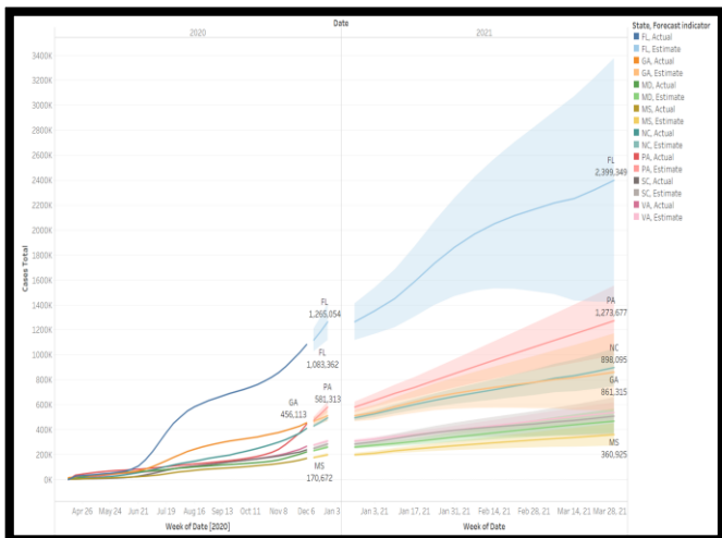
Figure 6. Holt-Winter exponential forecast of total COVID 19 Cases in FL, GA, MD, NC, SC, MS, PA and VA
