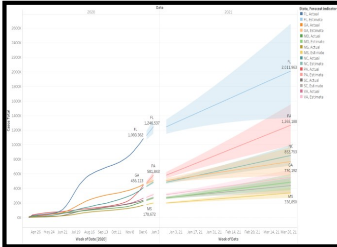
Figure 5. Holt exponential forecast of total COVID 19 Cases in FL, GA, MD, NC, SC, MS, PA and VA
