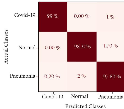
Figure 9. Confusion matrix for KL-MOB on the COVIDx test dataset.
