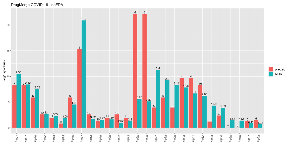
Figure 8: DrugMerge performance on COVID-19 data without FDA approval restriction. The bars represent the -\log_{10}(pvalue) with respect to the precision@20 (red), and the RHR (light blue). On the x-axis, different algorithms or combinations of them are indexed with aliases, since the complete algorithm names are too long. The mapping between them is on Table S5.1. The numbers on the top of the bars show the absolute values of precision@20 or RHR. The dotted red line represents the limit of significance ( -\log_{10}(0.05) ). All the bars above the dotted line show a significant p-value.
