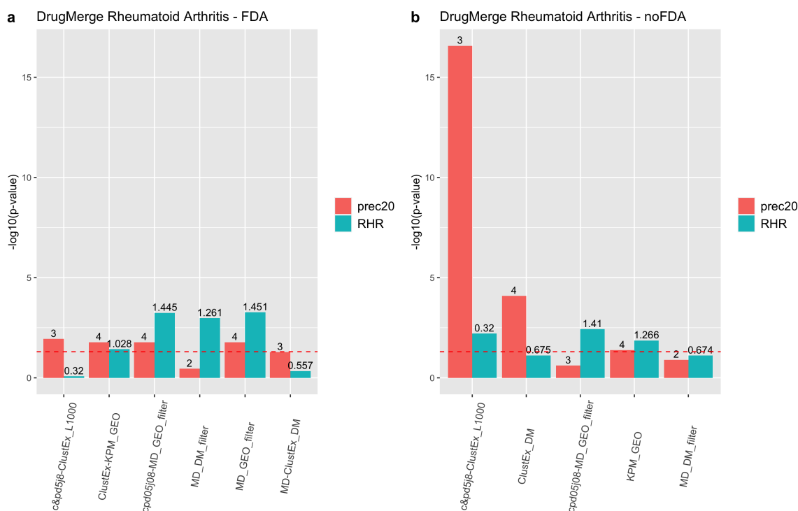
Figure 3: DrugMerge performance on Rheumatoid Arthritis data. The bars represent the -\log_{10}(pvalue) with respect to the precision@20 (red), and the RHR (light blu). On the x-axis, different algorithms or combinations of them are shown. The numbers on the top of the bars show the absolute values of precision@20 or RHR. The dotted red line represents the limit of significance ( -\log_{10}(0.05) ). All the bars above the dotted line show a significant p-value. The a) panel represents the DrugMerge performance when only FDA-approved drugs are considered; b) when all drugs (without any FDA filtering) are considered. The plot has been generated by the ggplot2 [Wickham et al., 2016] R package.
