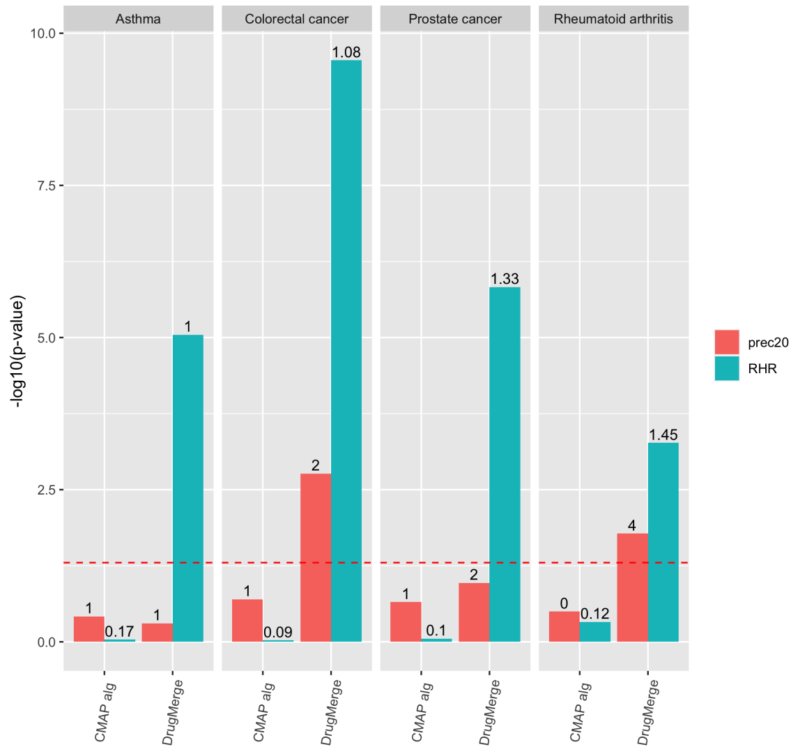
Figure 6: Comparison of performance of DrugMerge and the CMAP algorithm across the four benchmark diseases. For Colorectal Cancer and Prostate Cancer both methods use CMAP data. For Asthma and Rheumatoid Arthritis DrugMerge uses GEO data. The bars represent the -\log_{10}(pvalue) with respect to the precision@20 (red), and the RHR (light blu). The numbers on the top of the bars show the absolute values of precision@20 or RHR. The dotted red line represents the limit of significance ( -\log_{10}(0.05) ). All the bars above the dotted line show a significant p-value. The plot has been generated by the ggplot2 [Wickham et al., 2016] R package.
