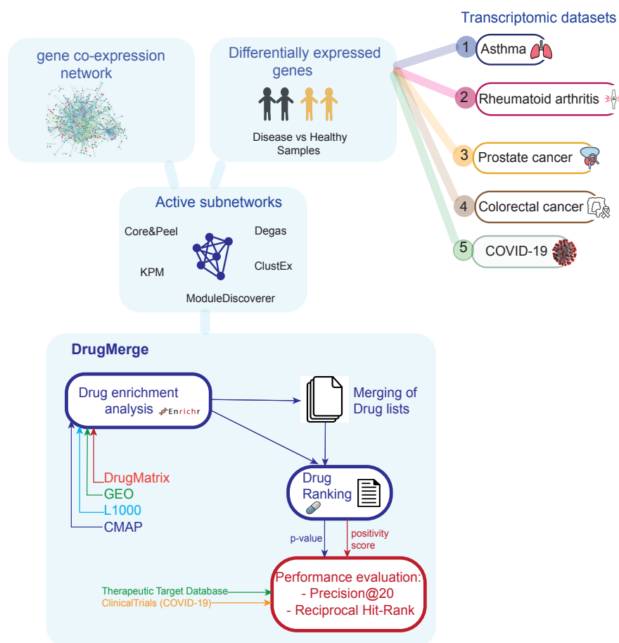
Figure 1: Overview of the workflow. The first part of the figure shows how we generated the data inputs of DrugMerge. These data have been created in [Lucchetta, 2020], and we reported them here for sake of completeness. We used several transcriptomic data to identify differentially expressed genes and the gene co-expression network to find one active subnetwork for each method used (Core&Peel, ModuleDiscoverer, Degas, ClustEx, and KeyPathwayMiner). For each of them, we performed the drug enrichment analysis on four drug perturbation databases: DrugMatrix, GEO, L1000, and CMAP. After that, we ranked the drugs according to the p-value or the positivity score. We also merged more drug lists, which come from different algorithms for the same disease and we applied the same ranking strategy. Finally, we evaluated the DrugMerge performance through the Precision@20 and the Reciprocal Hit-Rank using the golden-standard drugs, collected in the Therapeutic Target Database, and ClinicalTrials for COVID-19.
