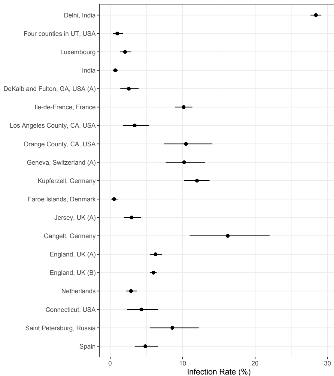
Figure 5: Analysis results from the Chen et al.-based analysis: posterior median estimates for the IR_k variables (for k = 1, \dots, 19 ) with 95% HPD CrIs. Studies are listed from top to bottom in the same order as in Figure 3.
