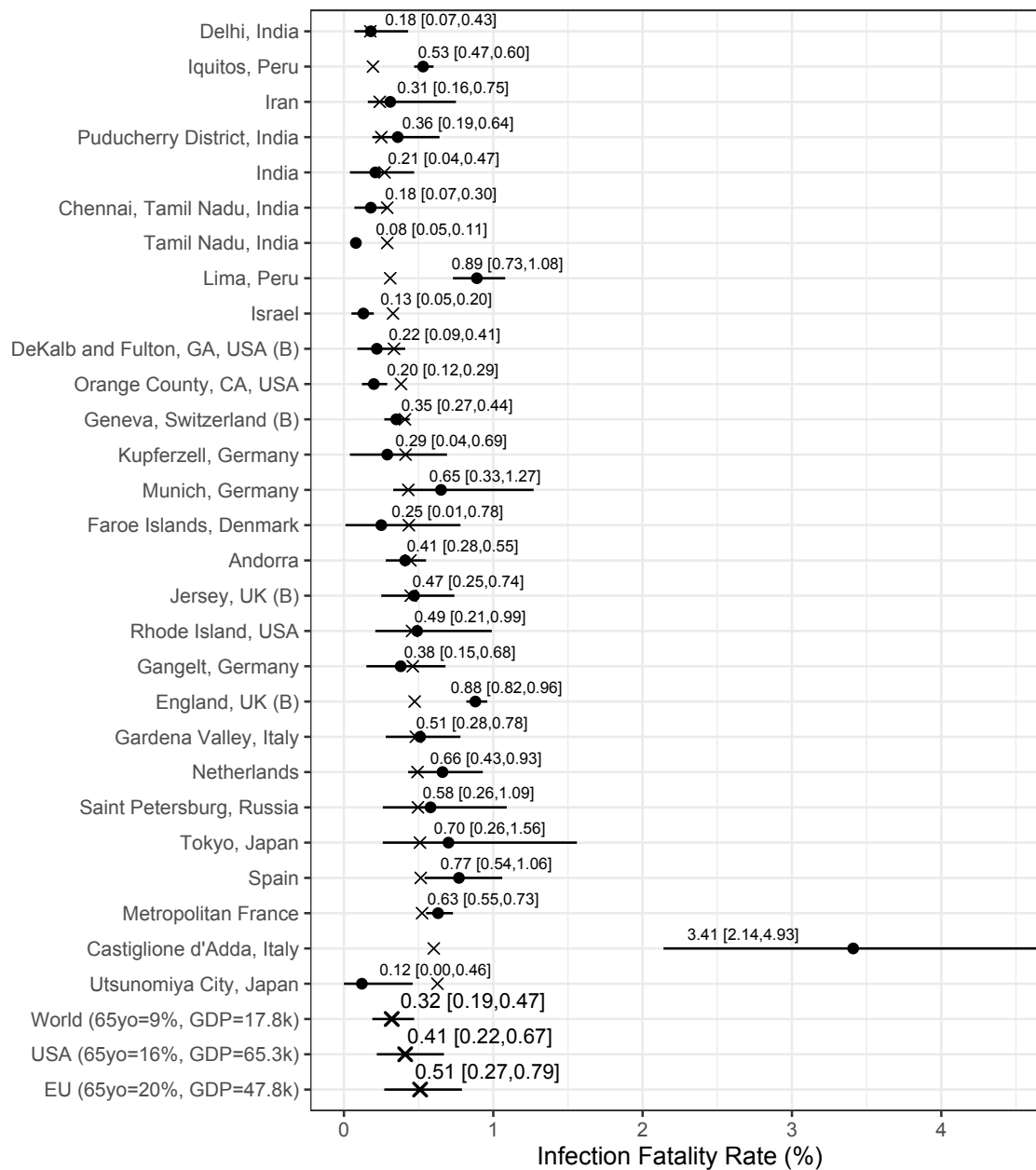
Figure 4: Results from the Serotracker-based analysis: posterior median estimates (black circles) for the IFR_k variables (for k = 1, \dots, 28 ) with 95% HPD CrIs. Studies are listed from the top to the bottom in order of increasing fitted values (these values are indicated by \times ). Also plotted, under the labels “World (65 yo=9%, GDP=17.8k)”, “USA (65 yo=16%, GDP=65.3k)”, “EU (65 yo=20%, GDP=47.8k)”, are the posterior median estimate and 95% HPD CrIs for the typical IFR corresponding to values for the proportion of the population aged 65 years and older of 9% and for GDP per capita of $17,811 (the worldwide values), of 16% and of $65,298 (the USA values), and of 20% and of $47,828 (the EU values).
