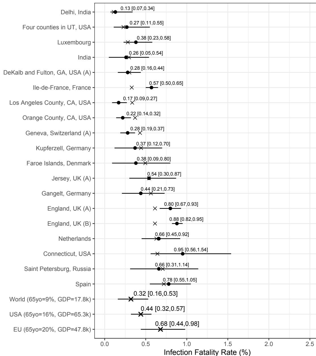
Figure 9: Analysis results from the Chen et al.-based analysis with alternative priors: posterior median estimates (black circles) for the IFR_k variables (for k = 1, \dots, 19 ) with 95% HPD CrIs. Studies are listed from top to bottom according to increasing fitted values (these values are indicated by \times ). Also plotted, under the labels “World (65 yo=9%, GDP=17.8K)”, “USA (65 yo=16%, GDP=65.3K)”, “EU (65 yo=20%, GDP=47.8K)”, are the posterior median estimate and 95% HPD CrIs for the typical IFR corresponding to values for the proportion of the population aged 65 years and older of 9% and for GDP per capita of $17,811 (the worldwide values), of 16% and of $65,297 (the USA values), and of 20% and of $47,828 (the EU values).
