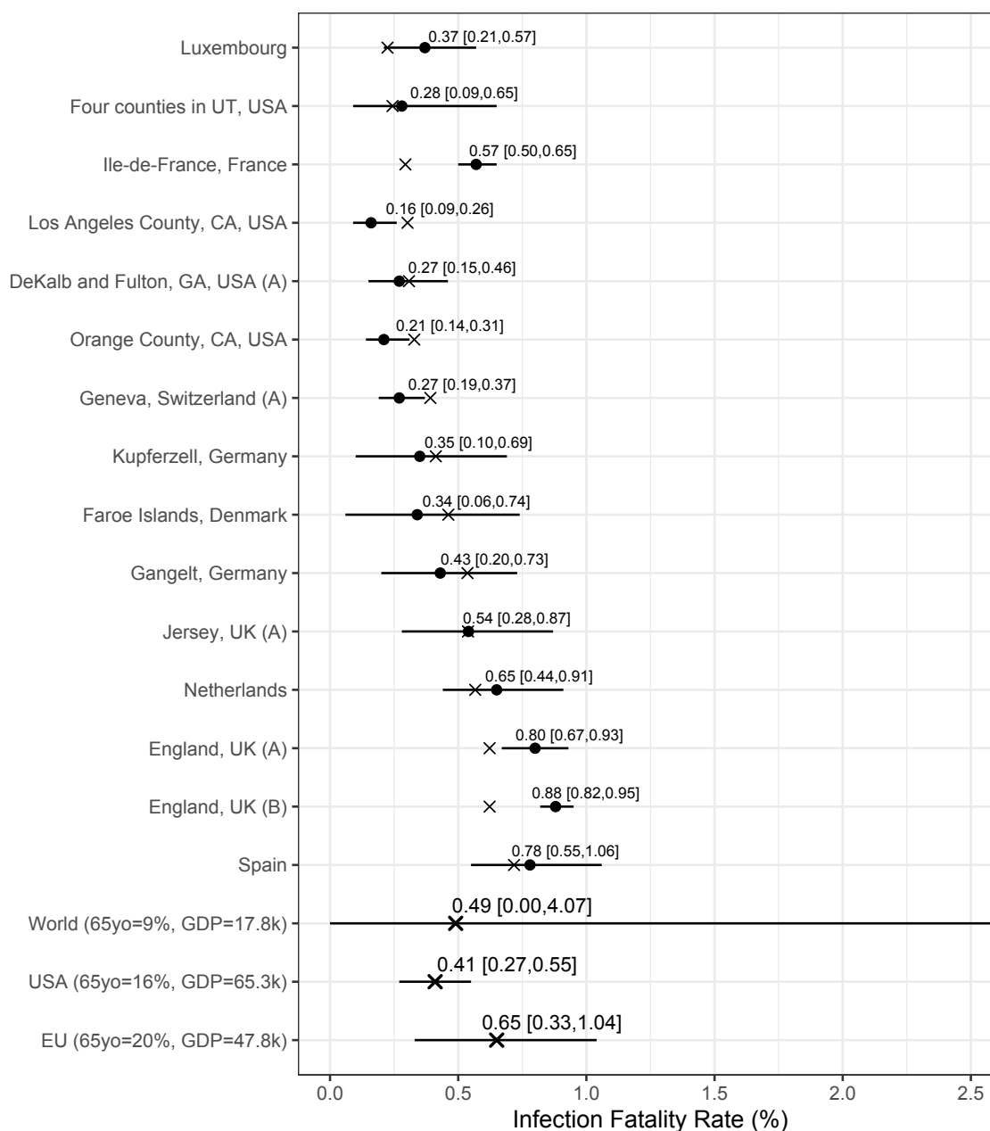
Figure 7: Chen et al.-based analysis results with only those studies for which mortality data was obtained from official sources known to be reliable: posterior median estimates (black circles) for the IFR_k variables (for k = 1, \dots, 15 ) with 95% HPD CrIs. Studies are listed from top to bottom in order of increasing fitted values (these values are indicated by \times ). Also plotted, under the labels “World (65 yo=9%, GDP=17.8k)”, “USA (65 yo=16%, GDP=65.3k)”, “EU (65 yo=20%, GDP=47.8k)”, are the posterior median estimate and 95% HPD CrIs for the typical IFR corresponding to values for the proportion of the population aged 65 years and older of 9% and for GDP per capita of $17,811 (the worldwide values), of 16% and of $65,298 (the USA values), and of 20% and of $47,828 (the EU values).
