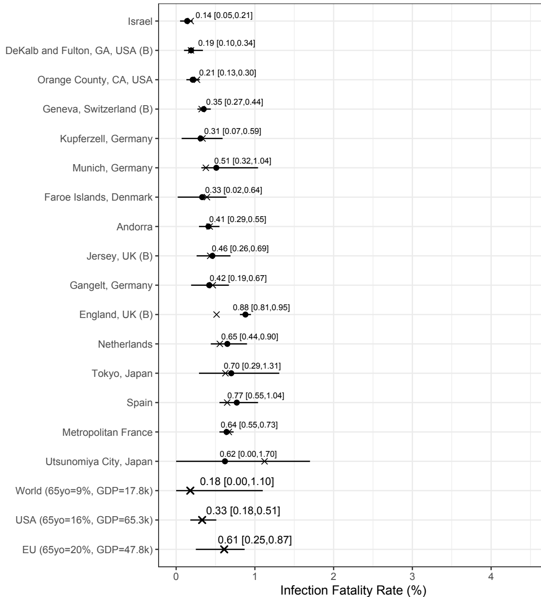
Figure 8: Serotracker-based analysis results with only those studies for which mortality data was obtained from official sources known to be reliable: posterior median estimates (black circles) for the IFR_k variables (for k = 1, \dots, 16 ) with 95% HPD CrIs. Studies are listed from top to bottom in order of increasing fitted values (these values are indicated by \times ). Also plotted, under the labels “World (65 yo=9%, GDP=17.8k)”, “USA (65 yo=16%, GDP=65.3k)”, “EU (65 yo=20%, GDP=47.8k)”, are the posterior median estimate and 95% HPD CrIs for the typical IFR corresponding to values for the proportion of the population aged 65 years and older of 9% and for GDP per capita of $17,811 (the worldwide values), of 16% and of $65,298 (the USA values), and of 20% and of $47,828 (the EU values).
