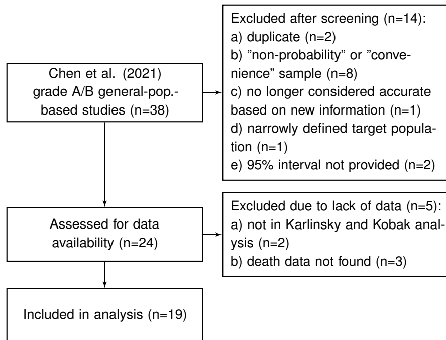
Figure 1: Flowchart of seroprevalence studies considered for Chen et al. -based analysis (based on the review of Chen et al. [29]).
