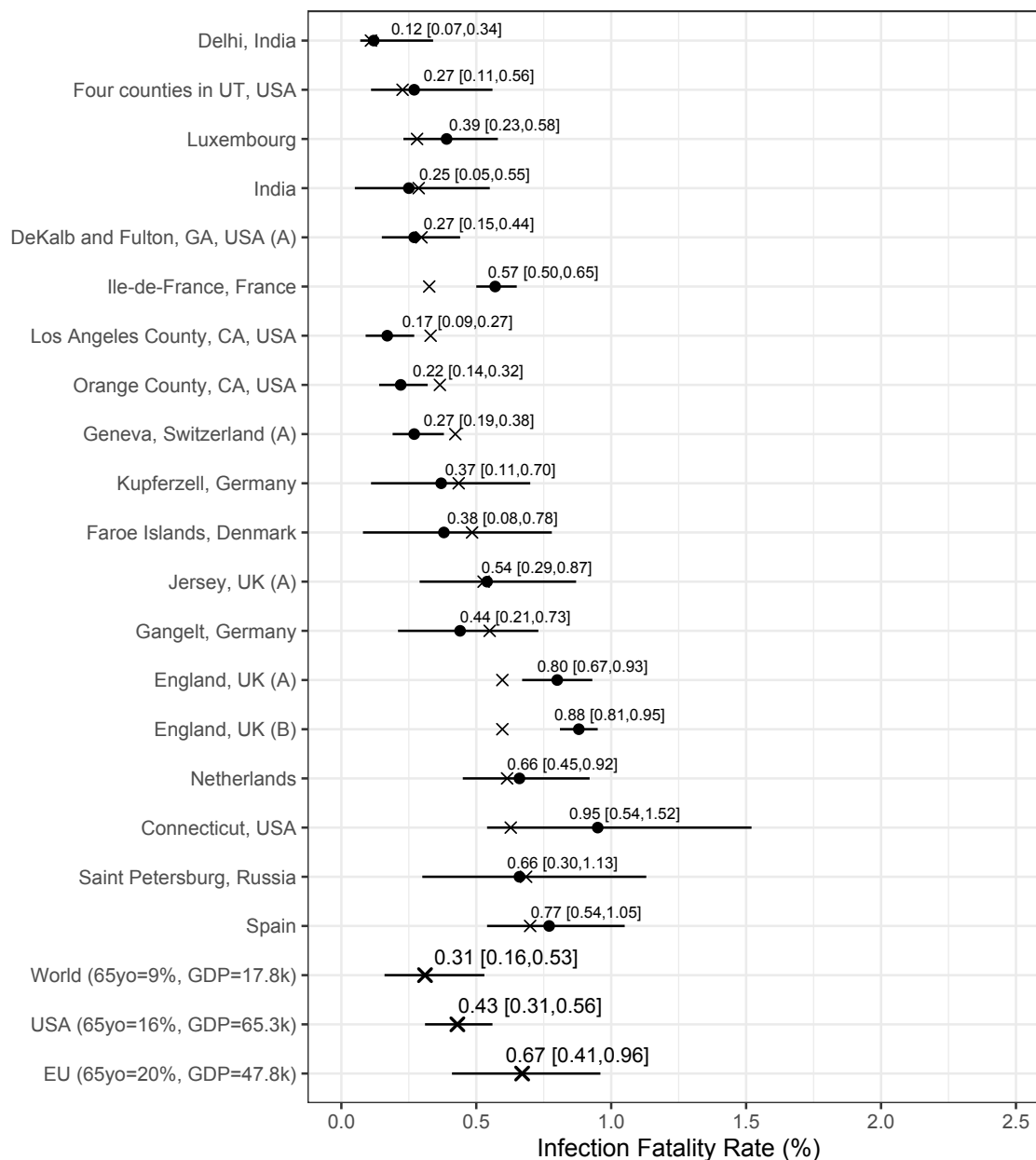
Figure 3: Results from the Chen et al.-based analysis: posterior median estimates (black circles) for the IFR_k variables (for k = 1, \dots, 19 ) with 95% HPD CrIs. Studies are listed from top to bottom in order of increasing fitted values (these values are indicated by \times ). Also plotted, under the labels “World (65 yo=9%, GDP=17.8k)”, “USA (65 yo=16%, GDP=65.3k)”, “EU (65 yo=20%, GDP=47.8k)”, are the posterior median estimate and 95% HPD CrIs for the typical IFR corresponding to values for the proportion of the population aged 65 years and older of 9% and for GDP per capita of $17,811 (the worldwide values), of 16% and of $65,298 (the USA values), and of 20% and of $47,828 (the EU values).
