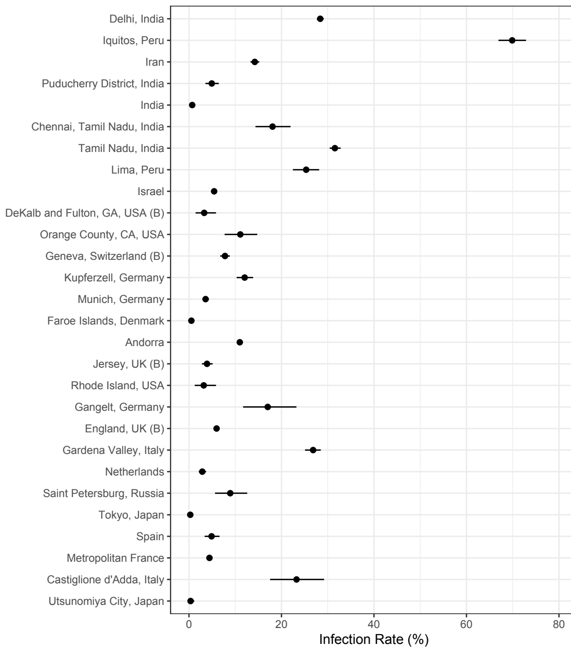
Figure 6: Analysis results from the Serotracker-based analysis: posterior median estimates for the IR_k variables (for k = 1, \dots, 28 ) with 95% HPD CrIs. Studies are listed from top to bottom in the same order as in Figure 4.
