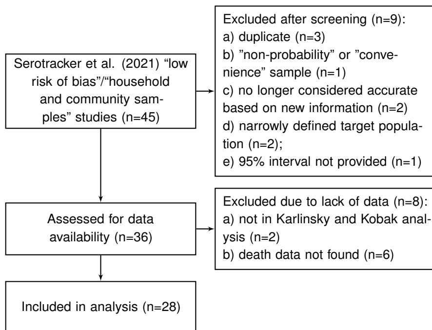
Figure 2: Flowchart of seroprevalence studies considered for Serotracker-based analysis (based on the Serotracker review Arora et al. [6]).
