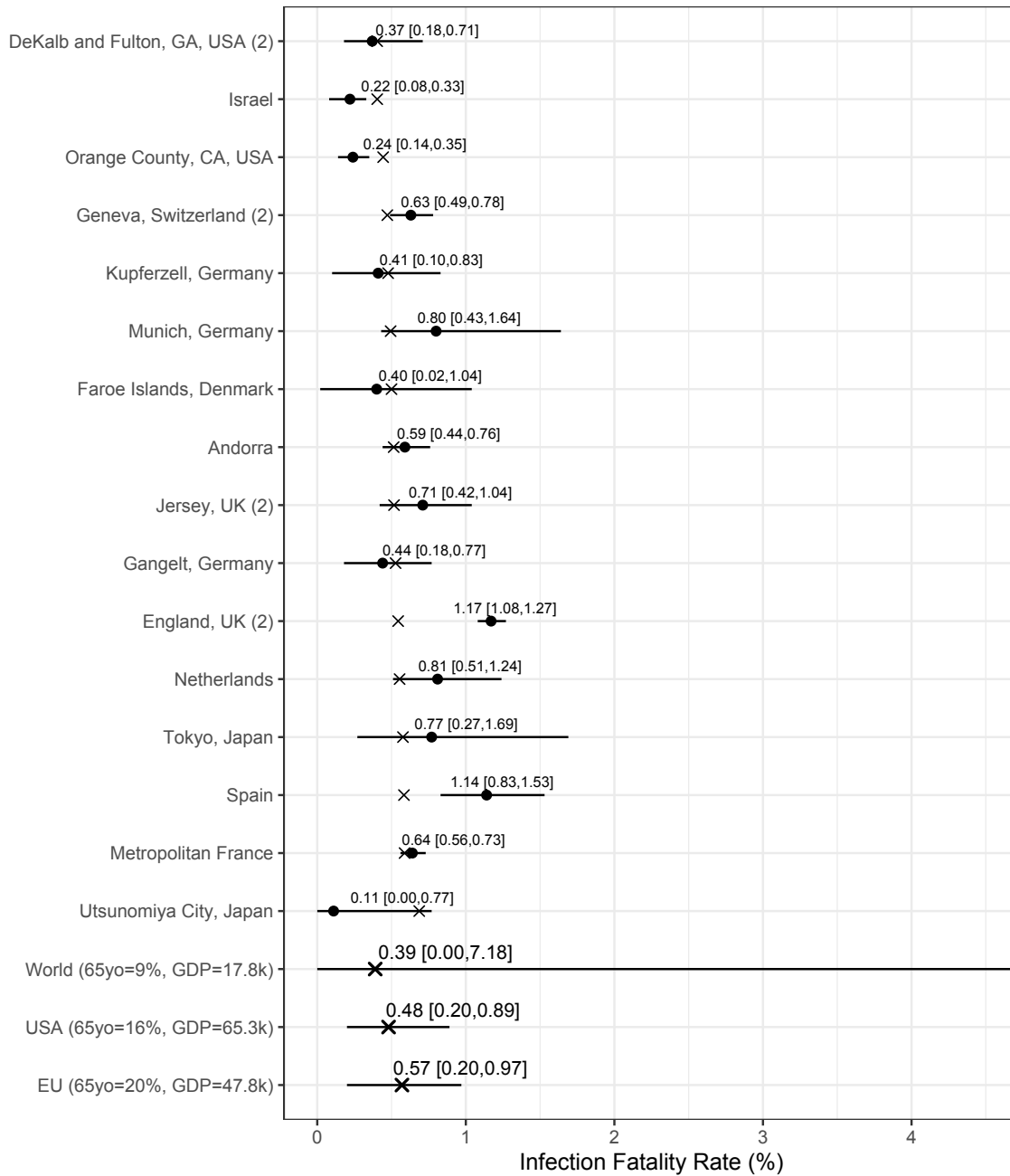
Figure 6: Serotracker-based analysis results with only those studies for which mortality data was directly (i.e., without any adjustments needed) obtained from official sources known to be reliable. Posterior median estimates for the IR_k and IFR_k variables (for k = 1, \dots, 18 ) with 95% HPD CrIs. Studies are listed from top to bottom according to increasing fitted values (these values are indicated by \times ). Also plotted, under the labels “World (65 yo=9%, GDP=17.8K)”, “USA (65 yo=16%, GDP=65.3K)”, “EU (65 yo=20%, GDP=47.8K)”, are the posterior median estimate and 95% HPD CrIs for the typical IFR corresponding to values for the proportion of the population aged 65 years and older of 9% and for GDP per capita of $17,811 (the worldwide values), of 16% and of $65,298 (the USA values), and of 20% and of $47,828 (the EU values).
