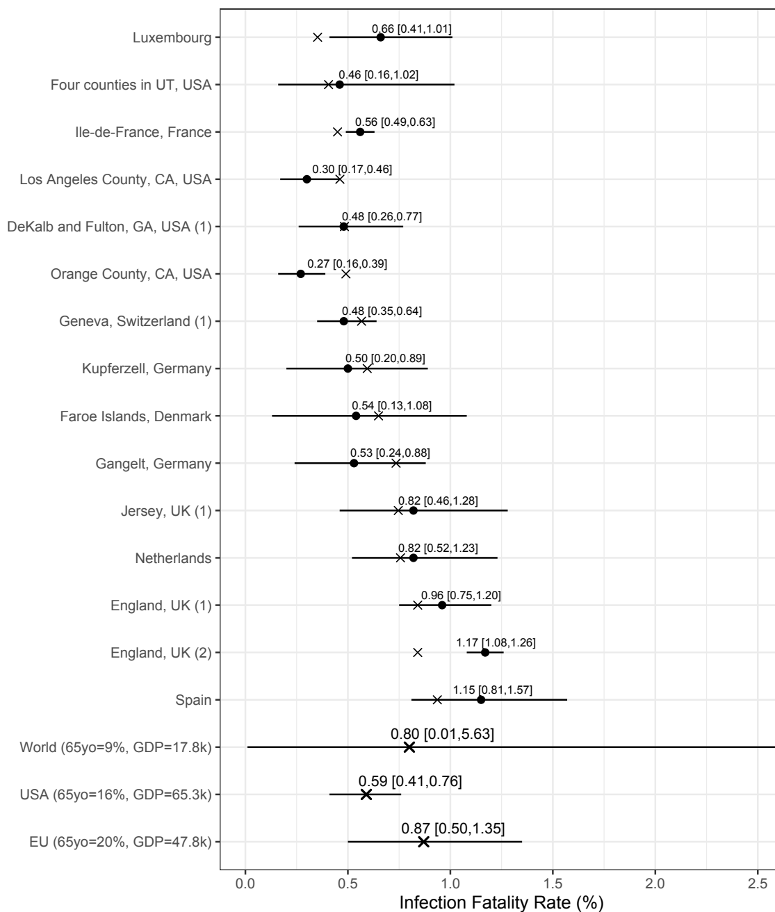
Figure 5: Chen et al.-based analysis results with only those studies for which mortality data was directly (i.e., without any adjustments needed) obtained from official sources known to be reliable. Posterior median estimates for the IR_k and IFR_k variables (for k = 1, \dots, 18 ) with 95% HPD CrIs. Studies are listed from top to bottom according to increasing fitted values (these values are indicated by \times ). Also plotted, under the labels “World (65 yo=9%, GDP=17.8K)”, “USA (65 yo=16%, GDP=65.3K)”, “EU (65 yo=20%, GDP=47.8K)”, are the posterior median estimate and 95% HPD CrIs for the typical IFR corresponding to values for the proportion of the population aged 65 years and older of 9% and for GDP per capita of $17,811 (the worldwide values), of 16% and of $65,298 (the USA values), and of 20% and of $47,828 (the EU values).
