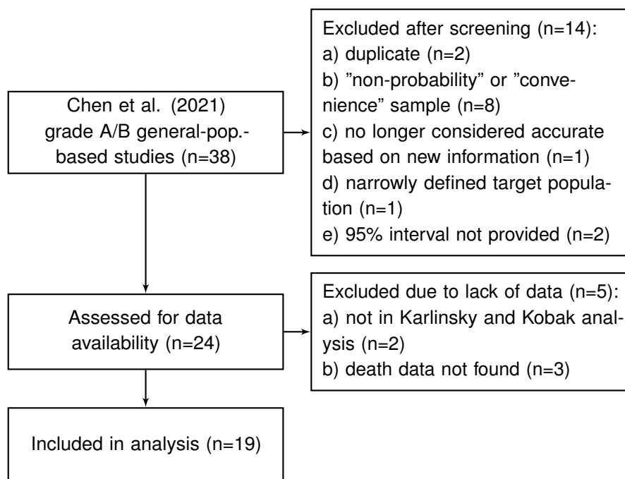
Figure 1: Flowchart of seroprevalence studies considered for Chen et al. -based analysis (based on the review of Chen et al. [28]).
