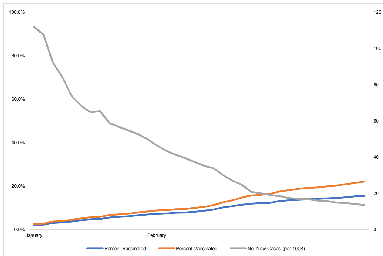
228 Figure: New SARS-CoV-2 Infections Against Percent Vaccinated in California, 229 January - March 2021 230
