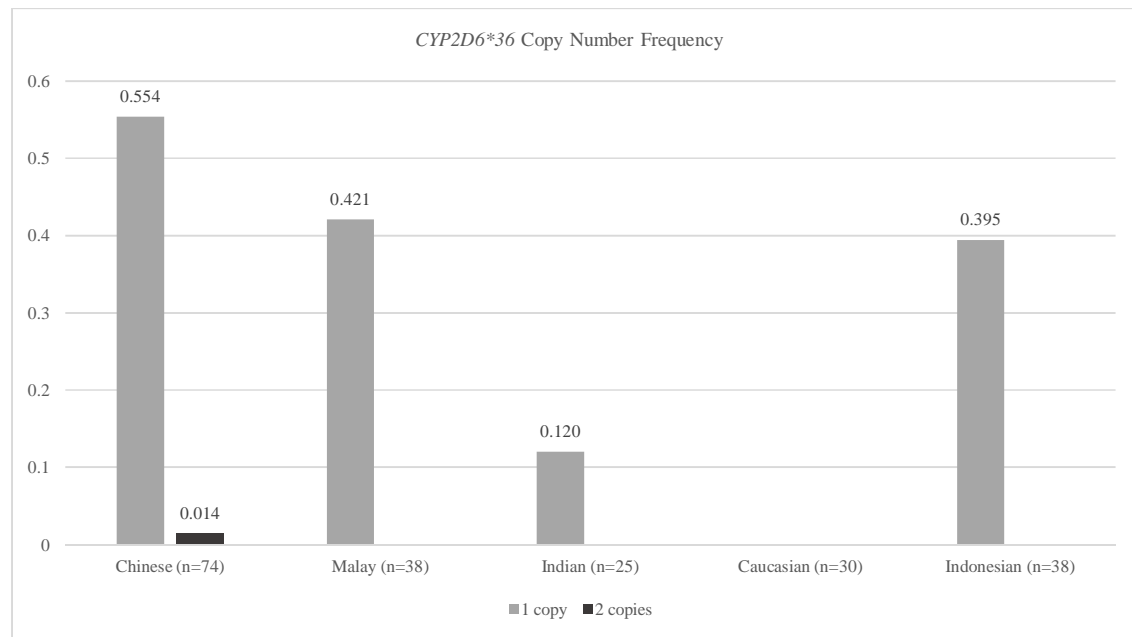
Figure 1. CYP2D6 *36 Frequency By Ethnicity. Distribution of individuals carrying one or two copies of the CYP2D6 *36 allele among the study cohort (n=205), grouped per ethnicity
