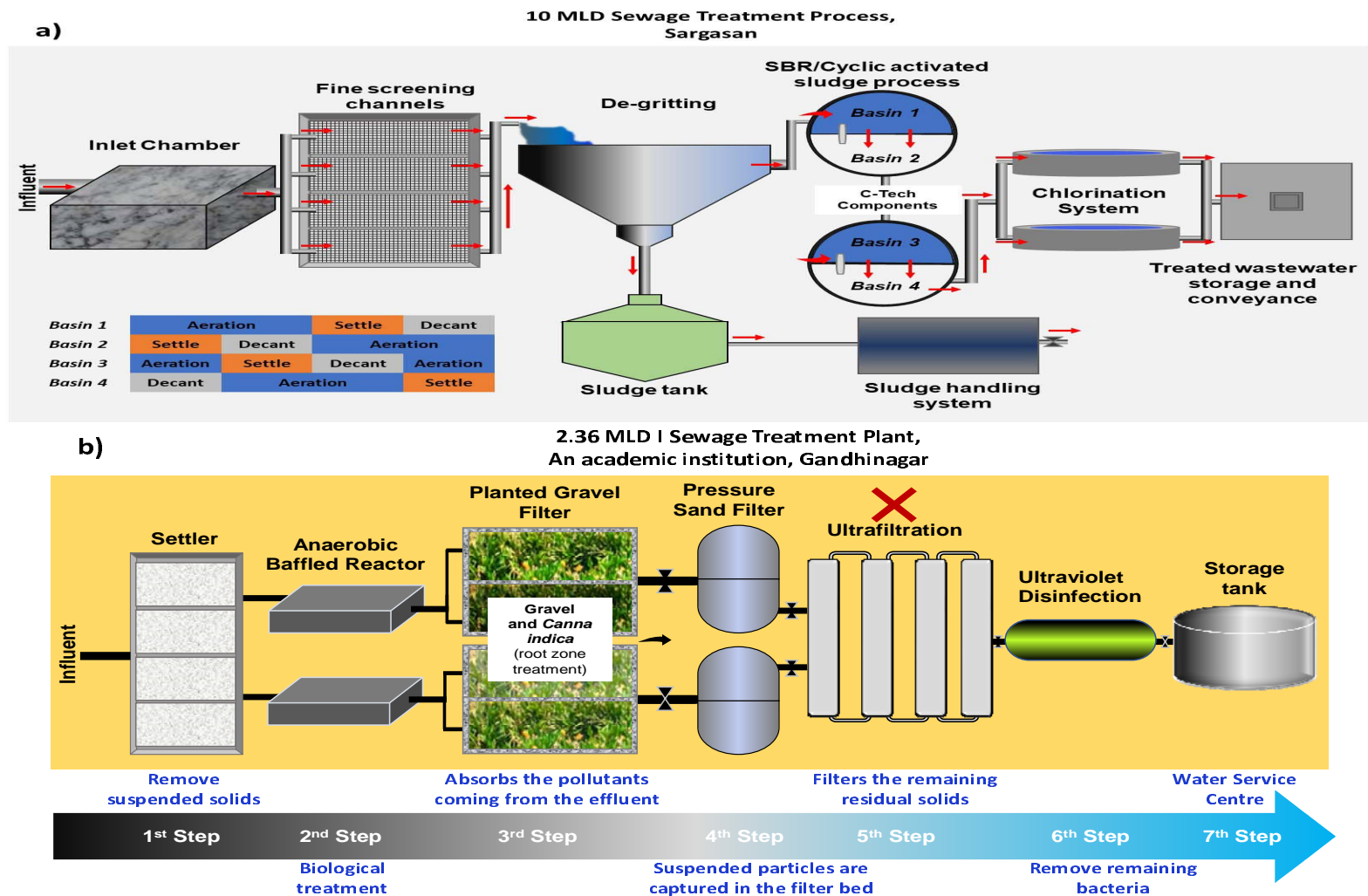
Fig.1. Simplified illustration of the layout of two wastewater treatment plants; a) Conventional Activated Sludge based WWTP in Sargasan, and b) root-zone treatment in an academic institution of Gandhinagar, India monitored during August and September, 2020.
