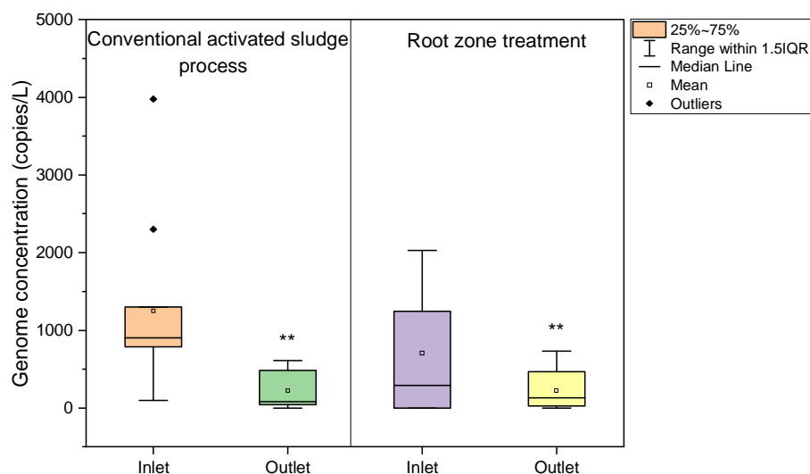
Fig. 4. Overall comparison of SARS-CoV-2 genome removal efficacy of conventional activated sludge and root-zone treatments expressed through paired T-test performed on the total effective genome concentrations obtained through out the 60 days of monitoring period. Same level of significance is used as above.
