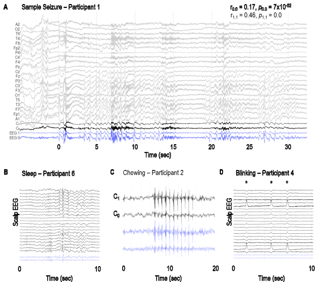
Figure 2: Sample EEG recordings. (A) Sample seizure in participant 1 and examples of (B) vertex waves and spindles during sleep, (C) chewing and (D) blinking artefacts (*) in participants 6, 2 and 4, respectively. C_0 and C_1 channels represent the bipolar recordings from the additional scalp electrodes placed over the sub-scalp electrodes. Blue traces (EEG 0 and EEG 1) represent the sub-scalp recordings. r_{0,0} and r_{1,1} represent the Pearson correlation coefficient between C_0 and EEG 0, and C_1 and EEG 1, respectively. p_{0,0} and p_{1,1} represent the respective p values.
