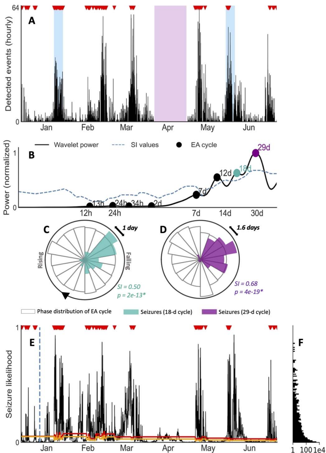
Figure 3: Seizure forecasting case study for patient 1. (A) Hourly rate of EA detected in the sub-scalp EEG device. Verified seizures (red markers) from review of sub-scalp EEG device are shown. The blue regions represent scalp video-EEG assessment periods, and the purple region represents a period where the device was turned off. (B) Cycle detection in EA using a
