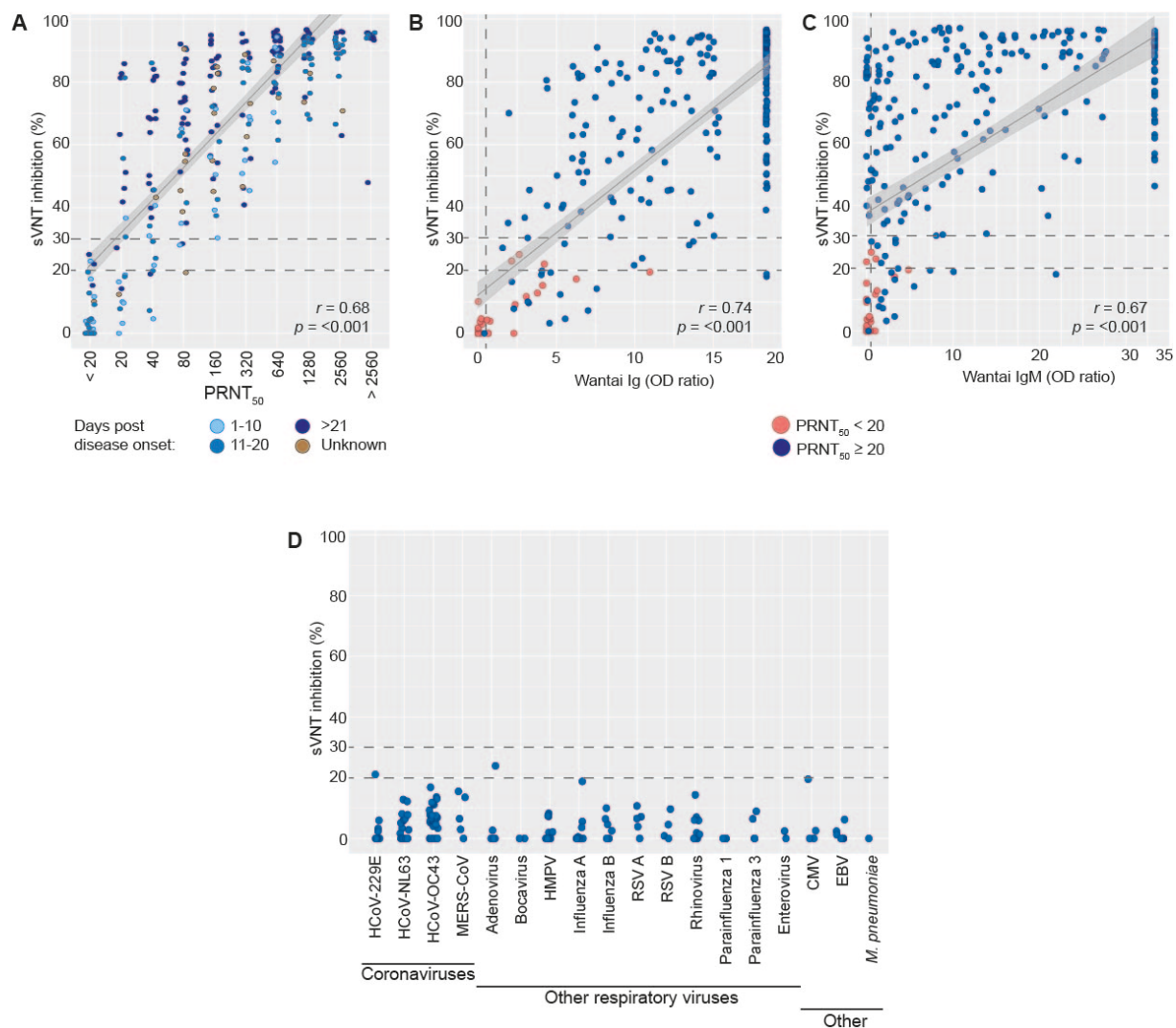
515 Fig. 1. sVNT results using the human validation panel containing confirmed COVID-19 516 patients compared to the PRNT 50 (A), the total Ig Wantai ELISA (B) or the IgM Wantai ELISA 517 (C). sVNT results using the cross-reactive human serum panel are shown in (D). Each dot 518 represents an individual serum. Dotted grey lines indicate the suggested cut-off values for the 519 presented assays. The grey lines in (A), (B) and (C) show the Spearman's correlation coefficient 520 ( r ) and its confidence interval (grey area) of the PRNT 50 / Wantai ELISAs and the sVNT. 521
