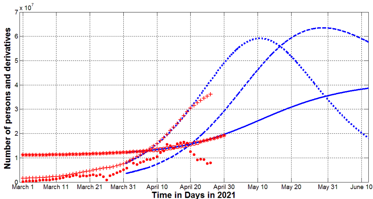
Figure. The COVID-19 epidemic dynamics in India.
