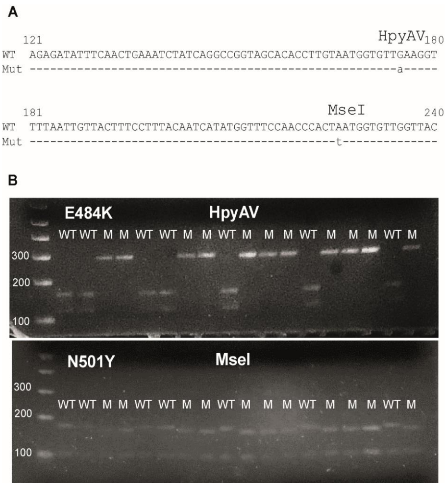
Figure 2. Restriction analysis of amplicons with E484K or N501Y mutations. A. Sequence of the amplified product showing the restriction sites which discriminate Wild-type (WT) or mutant (Mut or M) viruses. B. Agarose gel electrophoresis of digested PCR-amplified products. PCR-amplified products digested with the enzyme shown were run with molecular weight markers (1Kb plus DNA ladder): smaller bands are signaled (100, 200 and 300 bp).
