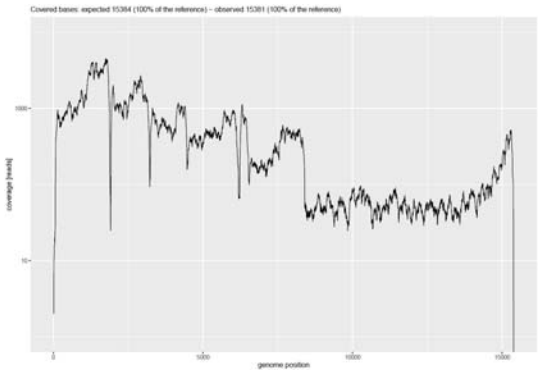
PDF coverage plot (command line)
