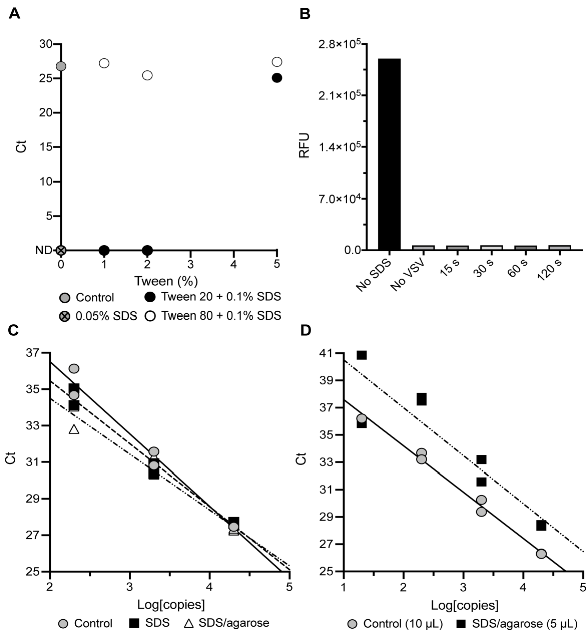
Figure 2: Denaturation of live viruses and nucleic acid amplification reactions using soap/surfactant combinations. (A) Determination of the minimal Tween 20 and Tween 80 concentration necessary for SDS sequestration to enable amplification of 20,000 copies/ \mu L of RNase P DNA. ND: not detected. (B) Fluorescence assay of eGFP-expressing recombinant VSV-SARS-CoV-2 ( 10^7 pfu/mL) infecting Vero-E6 cells after incubation with 0.1% (w/v) SDS for 15–120 seconds. Only a sample that was not exposed to SDS showed infectivity. 15 sec exposure to 0.1 % SDS proved sufficient to completely inactivate the virus, likely due to dissolution of its membrane and denaturation of the sample proteins. (C) Comparison of 10 \mu L qPCR reactions for SARS-CoV-2 N1 gene DNA amplification, containing 3% (v/v) of Tween 80 with and without 0.01% SDS (w/v, final) and 1% (w/v) agarose. (D) Comparison of a 10 \mu L qPCR reaction for SARS-CoV-2 N1 gene DNA containing 3% (v/v) Tween 80 with a 5 \mu L qPCR reaction for SARS-CoV-2 N1 DNA detection, containing 3% (v/v) Tween 80, 0.01% SDS (w/v, final) and 1% (w/v) agarose. In all conditions containing SDS, the DNA samples were initially incubated with 0.1% SDS (w/v) in Tris/EDTA buffer to simulate denaturing conditions for clinical samples. The samples were then centrifuged to mix with the Tween-containing PCR reactions.
