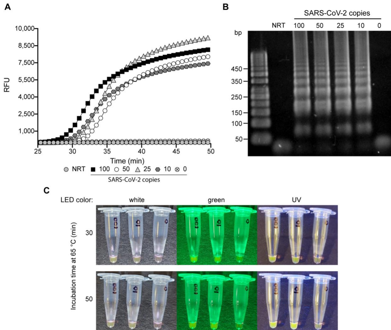
Figure 4: RT-LAMP amplification with SDS and Tween 80. (A) Real-time fluorescence of SARS-CoV-2 N gene amplification by RT-LAMP was performed at 65 °C for 50 minutes. Indicated concentrations (copies) of SARS-CoV-2 viral particles were assessed including a no-reverse-transcriptase (NRT) and no-template control (NTC; 0 copies), with all SARS-CoV-2 samples providing a positive result after ~30 minutes. (B) Amplification products (1 \mu L) from the real-time fluorescence RT-LAMP reaction were fractionated using agarose gel electrophoresis. The expected laddering pattern of LAMP amplification products was observed at all SARS-CoV-2 viral particle concentrations and not observed in NRT and NTC controls. (C) Fluorescence of RT-LAMP reactions of SARS-CoV-2 viral particles containing 20 \mu M SYTO 82 observed after 30 and 50 minutes of incubation at 65 °C. Reactions were analyzed with white, green, and UV (365 nm) handheld LED flashlights at each time point, with readily observable fluorescence of amplification reactions starting from 100 copies and 10 copies (labeled) after 30 minutes with each illumination. After 50 minutes, fluorescence in the 100-copy and 10-copy tubes increased with no observable amplification in the 0-copy control.
