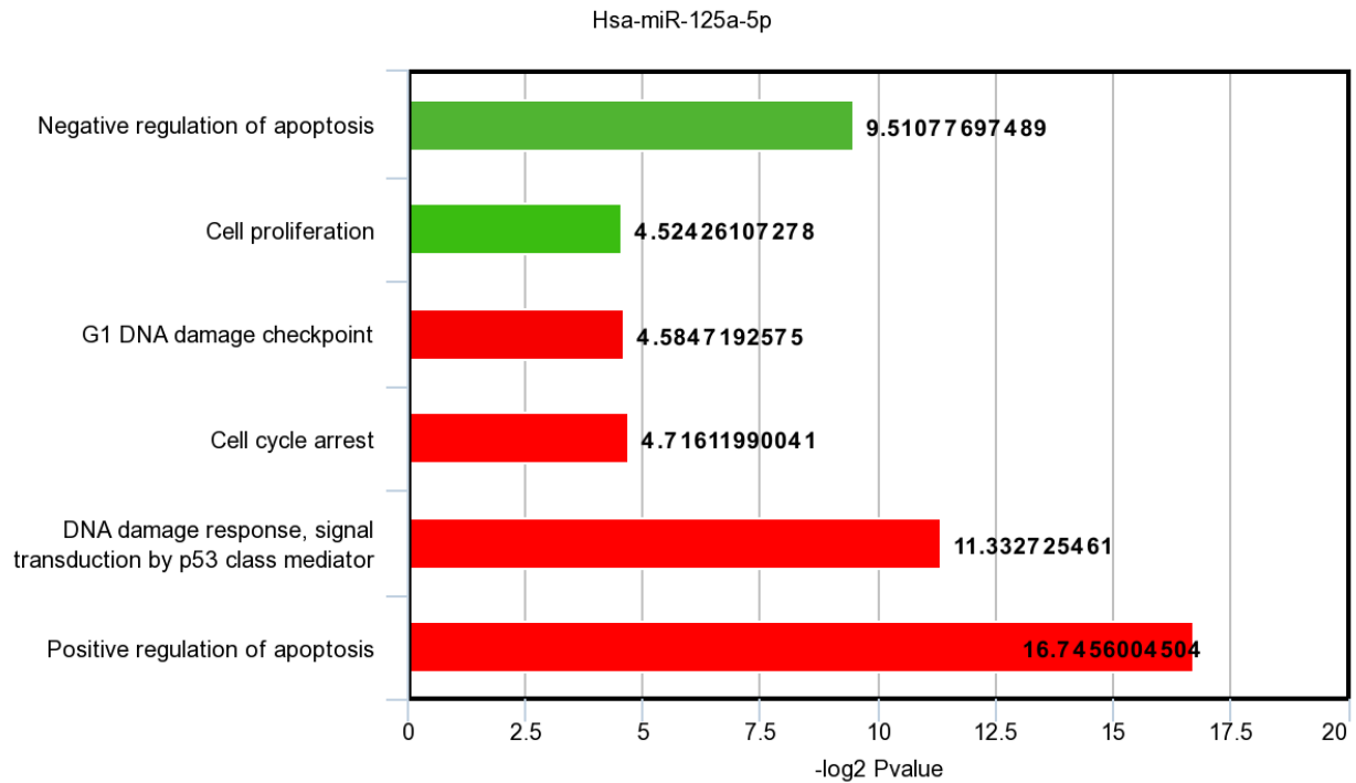
222 223 Figure5: BP of target genes of down expressed miRs in HCC. Green bars show the tumor 224 suppressor activity of miRs. Red bars show their oncogenic activity.
