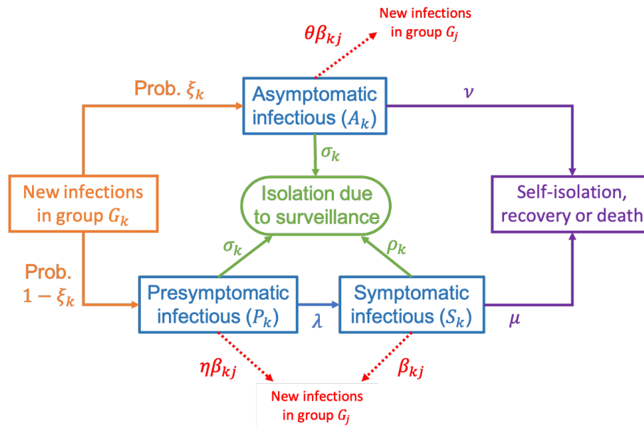
175 Fig 1. The branching process model used in our analyses. Schematic showing the different possible 176 events in the branching process model and the rates at which they occur. The parameters of the model 177 are described in the text and in Tables 1, 2 and 3.
