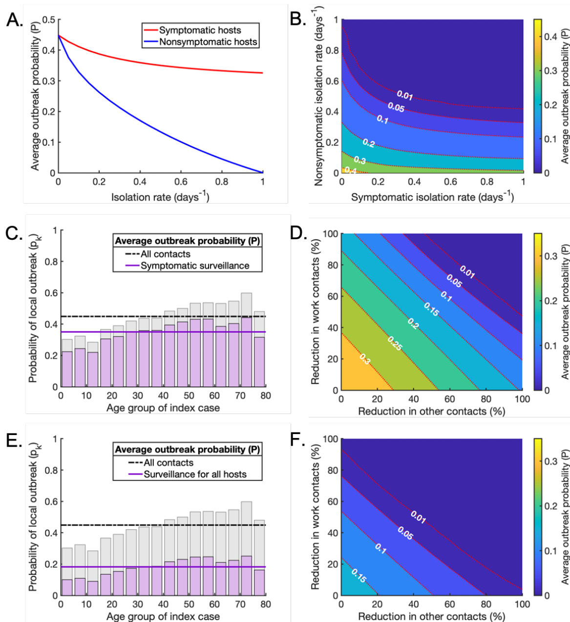
521 522 Fig 6. Surveillance as part of a mixed strategy to reduce the local outbreak probability. A. The 523 effect of increasing the isolation rate of symptomatic (red line) or nonsymptomatic infected hosts (blue 524 line) on the average probability of a local outbreak ( P ), in the absence of contact-reducing NPIs. The 525 isolation rates \rho_k and \sigma_k are varied in turn between 0 days -1 and 1 days -1 . B. The effect of 526 simultaneously varying the isolation rate of symptomatic and nonsymptomatic hosts on the average 527 probability of a local outbreak ( P ), again without contact-reducing NPIs. C. The age-dependent
