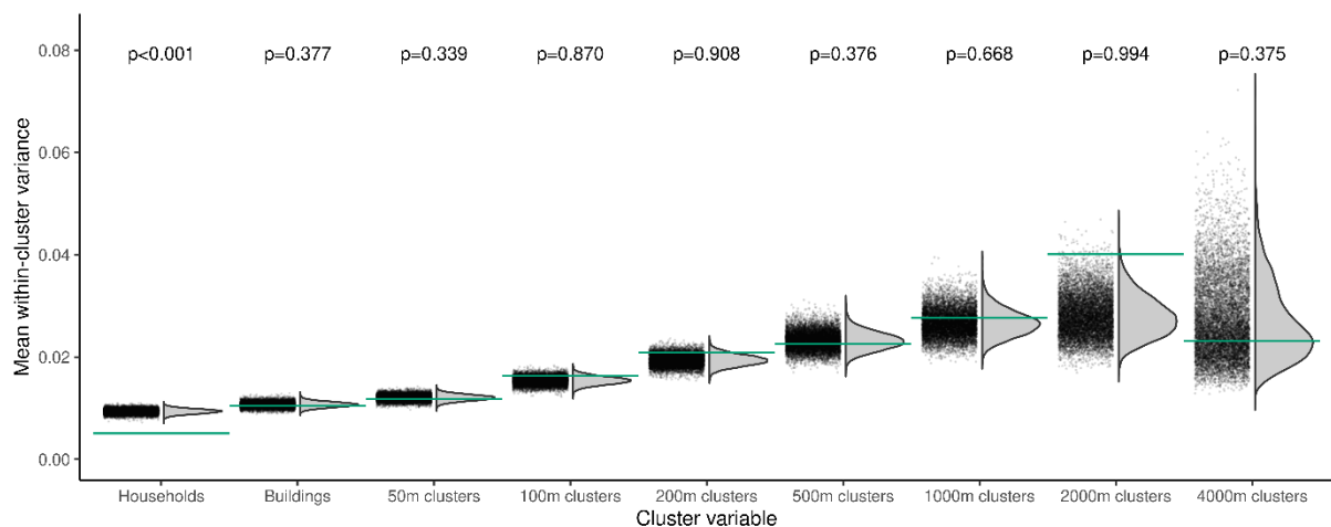
Figure 7: Proximity clustering of test outcomes at 2 nd sampling. The grey points and curves show the distribution of mean within-cluster variances for 10,000 random permutations of cluster assignments, the horizontal lines show the observed values. Cluster variables are households, buildings, and geospatial clusters of different sizes. Household membership was left invariant when considering buildings and geospatial clusters. P-values indicate the one-sided probability of observing smaller than observed values under random cluster assignments.
