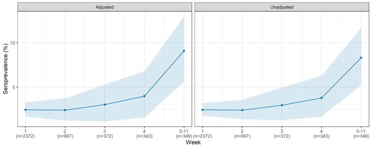
Figure 4: For sensitivity and specificity adjusted (left) and unadjusted (right) SARS-CoV-2 seroprevalence over the follow-up period. The 95% confidence intervals for the weekly seroprevalence were based on the 2.5 and 97.5 percentiles from 5,000 repetitions of a cluster bootstrap that accounts for within household clustering. The estimates do not account for sample weights. The estimation without accounting for within-household clustering but considering sample weights produced similar trends (Appendix Figure S1).
