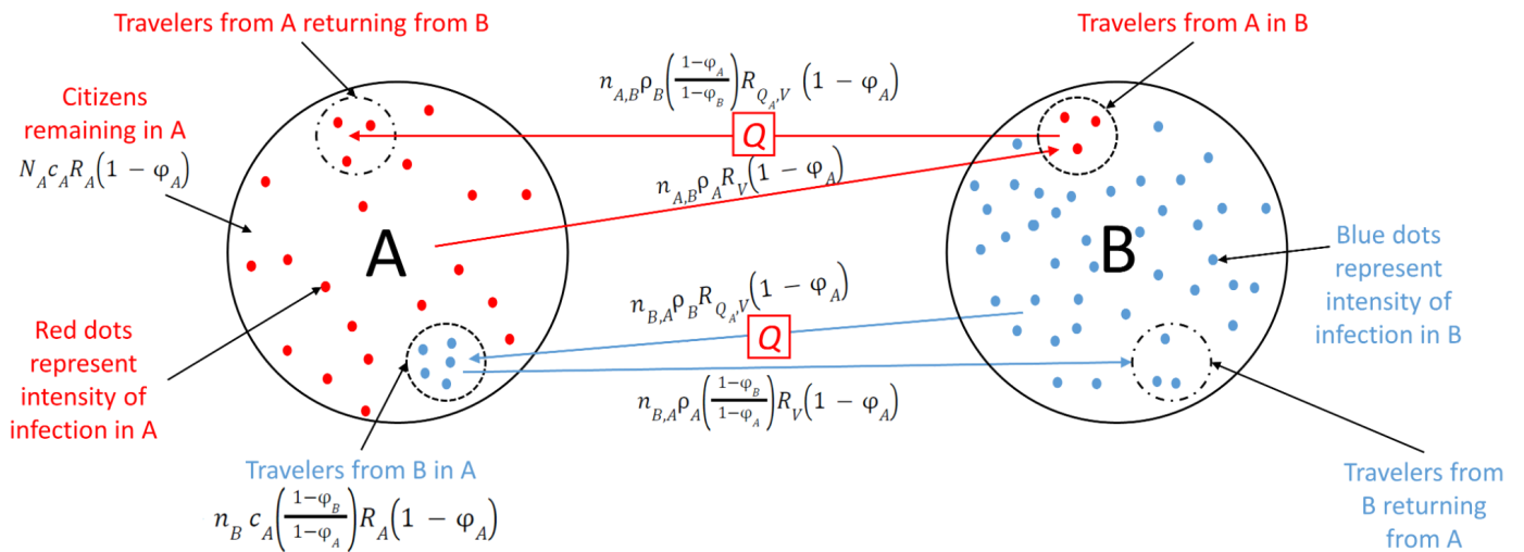
Figure 1. Model schematic diagram for imminent infections and travel quarantine. With travel between country A (red) and country B (blue), the travel quarantine specified by country A is dependent on the intensity of infection in both country A and B, the number of residents leaving country A for country B, the number of travellers entering country A from country B, the number of residents returning to country A, and the number of travellers from country B returning to country B. In the most general instantiation of our model, the minimum duration of travel quarantine is dependent on the number of daily travellers from country A to country B, n_{AB} , the number of daily travellers from country B to country A, n_{BA} , the country-specific prevalence of non-isolated infections \rho , country-specific immunity \varphi , the number of travellers from country B abroad in country A, n_B , the number of citizens of A who are non-travellers and not quarantined, N_A , daily fractional incidence, c . The amount of remaining transmission ( R_A , R_V , R_{Q,V} ) is calculable based on virus- or variant-specific properties and the temporal infectivity and test sensitivity [7].
