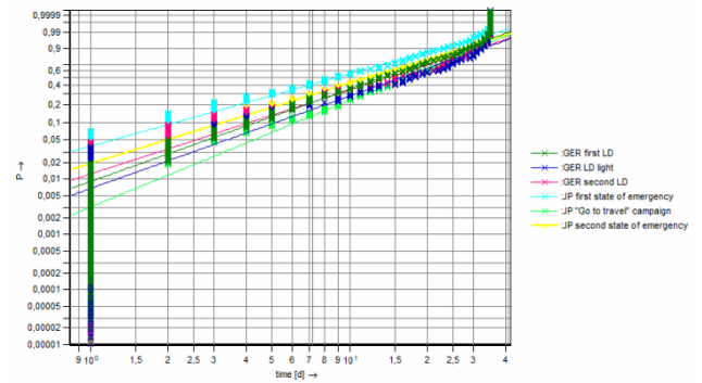
Fig. 7. Weibull distribution models COVID-19 in Germany (GER) and Japan (JP), comparison of different pandemic measures/lockdown (LD), confirmed cases, time span 35 days.
