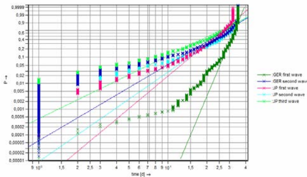
Fig. 6. Weibull distribution models COVID-19 in Germany (GER) and Japan (JP), comparison of different pandemic waves, confirmed cases, time span 35 days.
