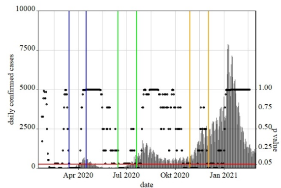
Fig. 3. Detection of waves of COVID-19 in Japan with Cox-Stuart trend test, p values (black points), \alpha=0.05 (red line), daily confirmed cases (grey lines), first wave (blue lines), second wave (green line) and third wave (yellow line).
