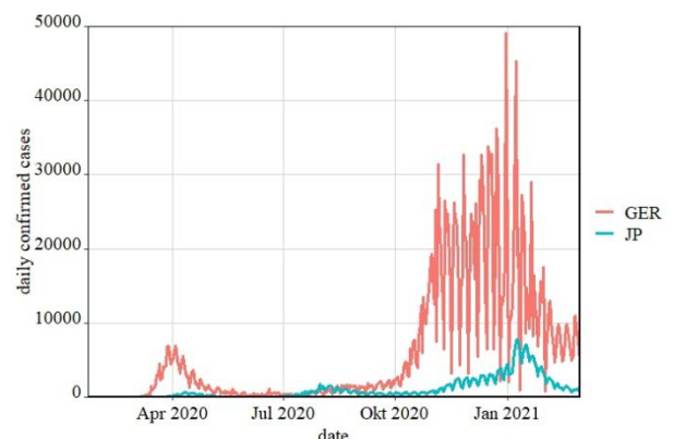
Fig. 5. Daily confirmed cases in Germany (GER) and Japan (JP) January 2020 until March 2021.
