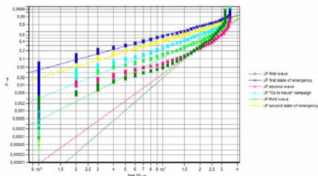
Fig. 4. Weibull distribution models COVID-19 in Japan (JP), comparison of different pandemic phases with different measures, confirmed cases, time span 35 days.
