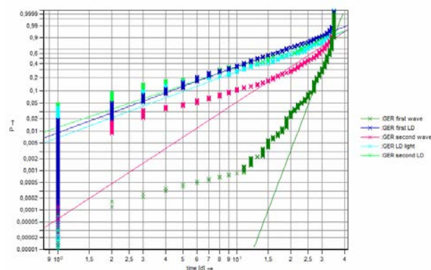
Fig. 2. Weibull distribution models COVID-19 in Germany (GER), comparison of different pandemic phases with lockdown (LD) measures, confirmed cases, time span 35 days.
