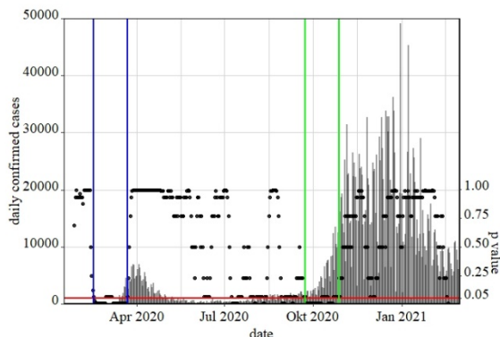
Fig. 1. Detection of waves of COVID-19 in Germany with Cox-Stuart trend test, p values (black points), \alpha=0.05 (red line), daily confirmed cases (grey lines), first wave (blue lines) and second wave (green line).
