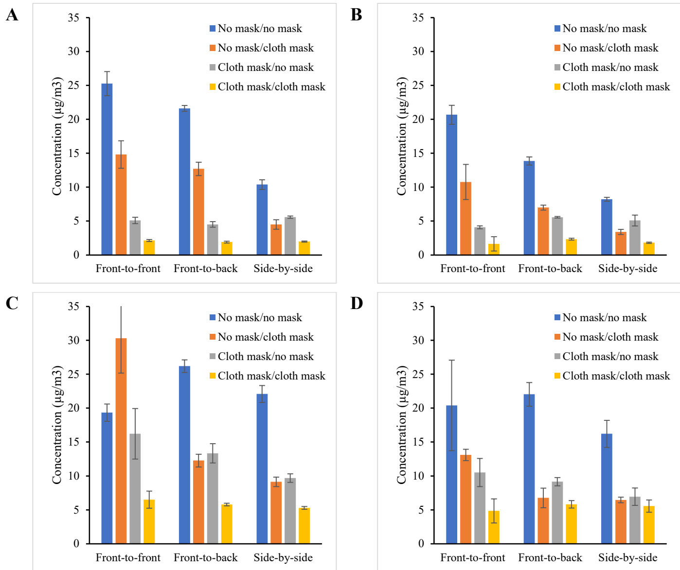
Figure 4: Mean aerosol concentration over 15 minutes measured at the mouth of the recipient simulator with and without masks and with simulators in different orientations. (A) Source is coughing, simulators are 0.9 m (36") apart. (B) Source is coughing, simulators are 1.8 m (72") apart. (C) Source is breathing, simulators are 0.9 m apart. (D) Source is breathing, simulators are 1.8 m apart. Each bar is the mean of three experiments. Error bars show the standard deviation.
