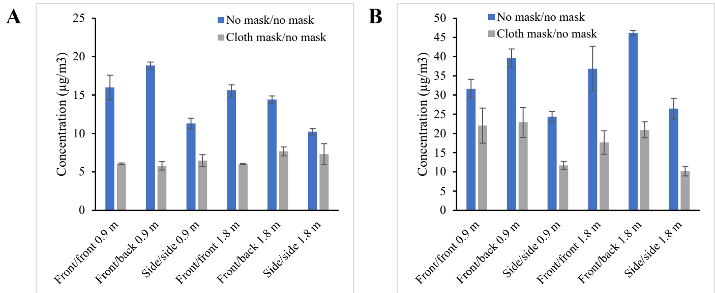
Figure 6: Aerosol concentration in the environmental chamber with and without a mask on the source simulator during (A) coughing experiments and (B) breathing experiments. The recipient simulator was unmasked during these experiments. The simulators were 0.9 or 1.8 m apart and oriented front-to-front, front-to-back, or side-by-side. For each experiment, the 15-minute mean concentrations at five locations (excluding the location at the mouth of the recipient) were averaged to determine the chamber concentration. Each bar shows the average and standard deviation of the chamber concentrations from three experiments. Note that the source simulator expels a larger mass of aerosol during breathing experiments than during coughing experiments.
