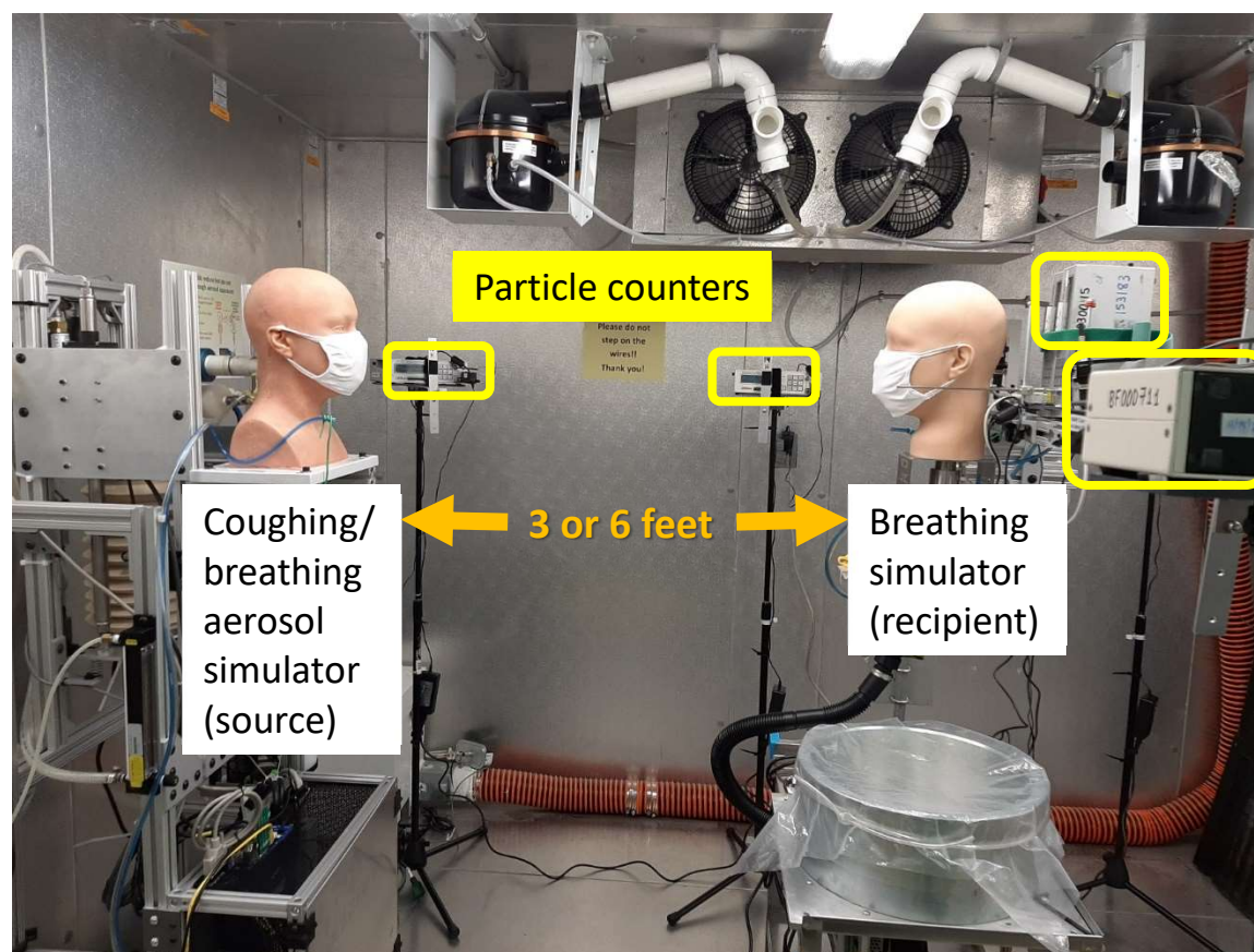
Figure S1: Photograph of experimental set-up in the environmental chamber. In this experiment, the source and recipient simulators were front-to-front 0.9 m apart.
