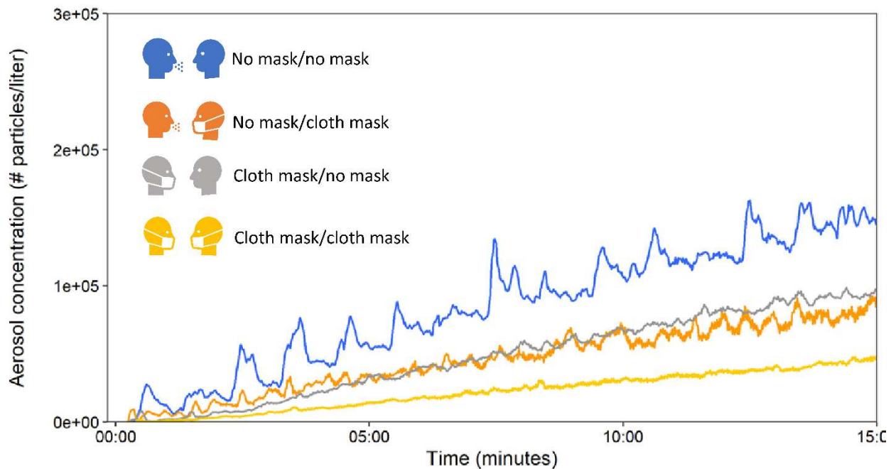
Figure 3: Aerosol concentration at mouth of recipient (breathing simulator) while source (cough & exhaled aerosol simulator) is exhaling aerosol. Source and recipient were 1.8 m (72") apart and facing each other. Each line shows data from single experiment. The plots were smoothed with a 7-point running average for clarity.
