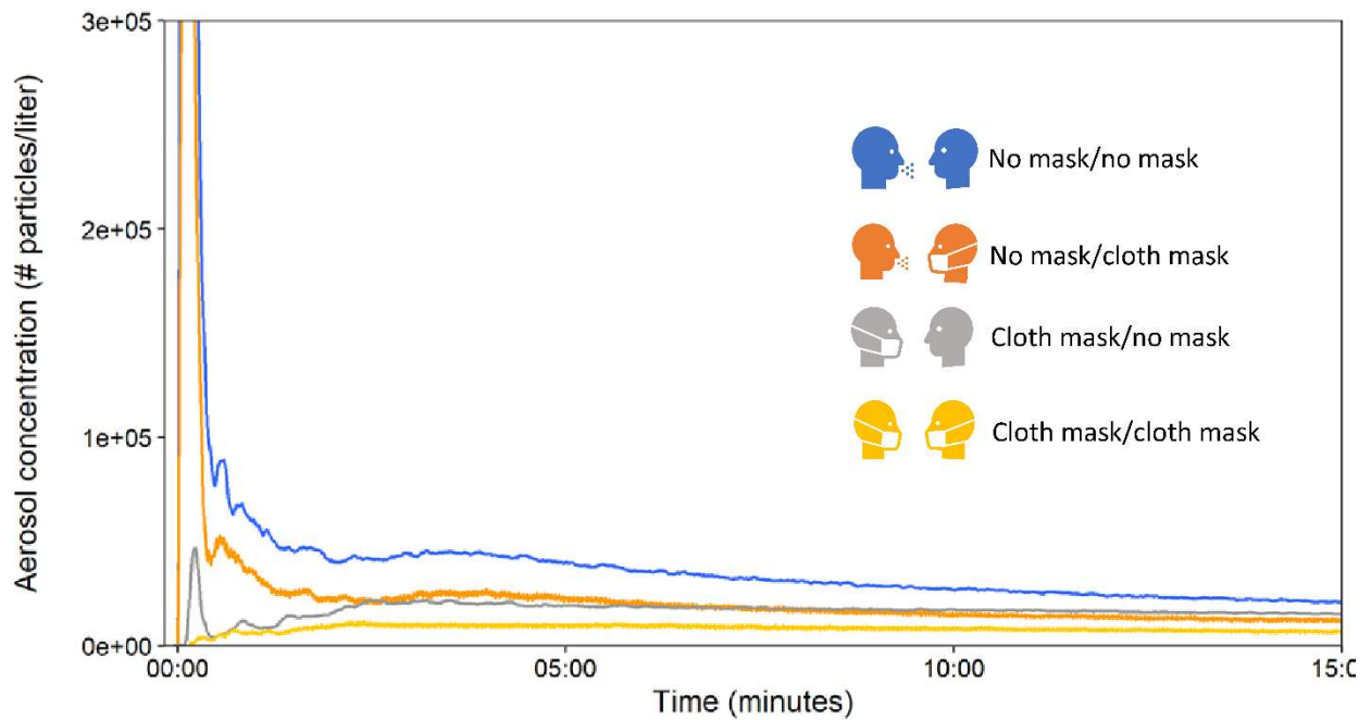
Figure 2: Aerosol concentration at mouth of recipient (breathing simulator) after single cough from source (cough & exhaled aerosol simulator). The concentration is shown as total particles/liter for 0.3 to 3 \mu\text{m} aerosol particles, which is the format reported by the aerosol particle counter. Source and recipient were 1.8 m (72") apart and facing each other. Each line shows data from a single experiment. The plots were smoothed with a 7-point running average for clarity.
