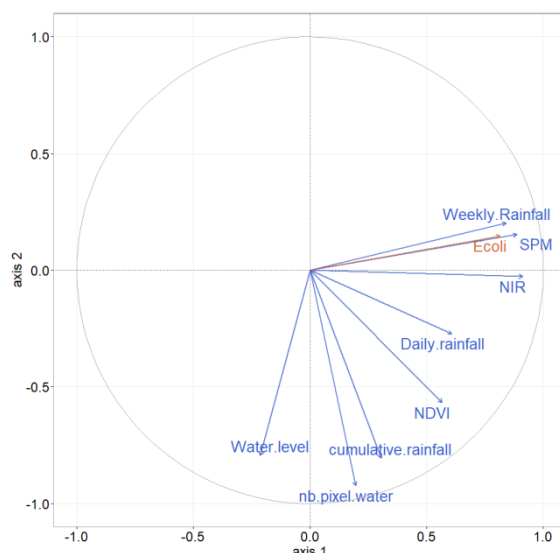
525 526 Fig 7. Correlation circle of partial least squares (PLS) regression, illustrating relationships between 527 predictor variables (blue), E. coli (orange) and the two first PLS components (first component on the x- 528 axis, second one on the y-axis ). 529
