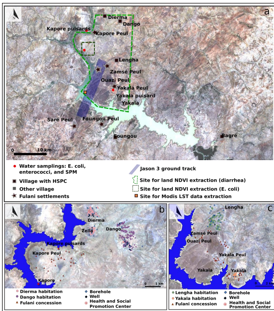
237 238 Fig 1. (a) Study Area (Sentinel-2 image 22/04/2018); (b) Zoom on the area of Dango, Dierma and Kapore; 239 (c) Zoom on the area of Lengha, Lengha Peul, Yakala and Yakala Peul
