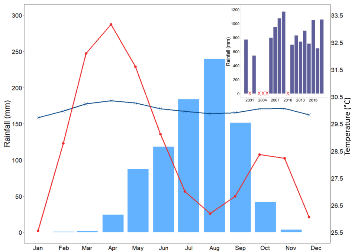
261 262 Fig 2. Average monthly rainfall for the period 2000-2018 (bar chart in blue, Tenkodogo station), air 263 temperatures for the period 2000-2018 (red line with dots, Fada N’Gourma station) and satellite_derived 264 surface water temperatures for the period 2000-2018 (blue line with crosses). Annual rainfall from 2000 to 265 2018 is shown in the inset (no data is available for 2001, 2003-2005 and 2010) 266
