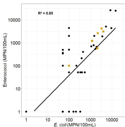
466 467 Fig 5. Enterococci vs E. coli for the Kapore routine point (N=38), and for “puisards” (N=6, yellow 468 squares).
