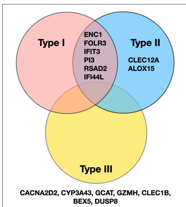
Figure 3. Venn diagram of differentially expressed genes in seropositive individuals with prior asymptomatic or clinical SARS-CoV-2 infection with respect to interferon activity.
