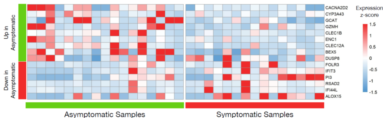
Figure 2. Differential gene expression analysis in seropositive individuals with prior asymptomatic or clinical SARS-CoV-2 infection.
