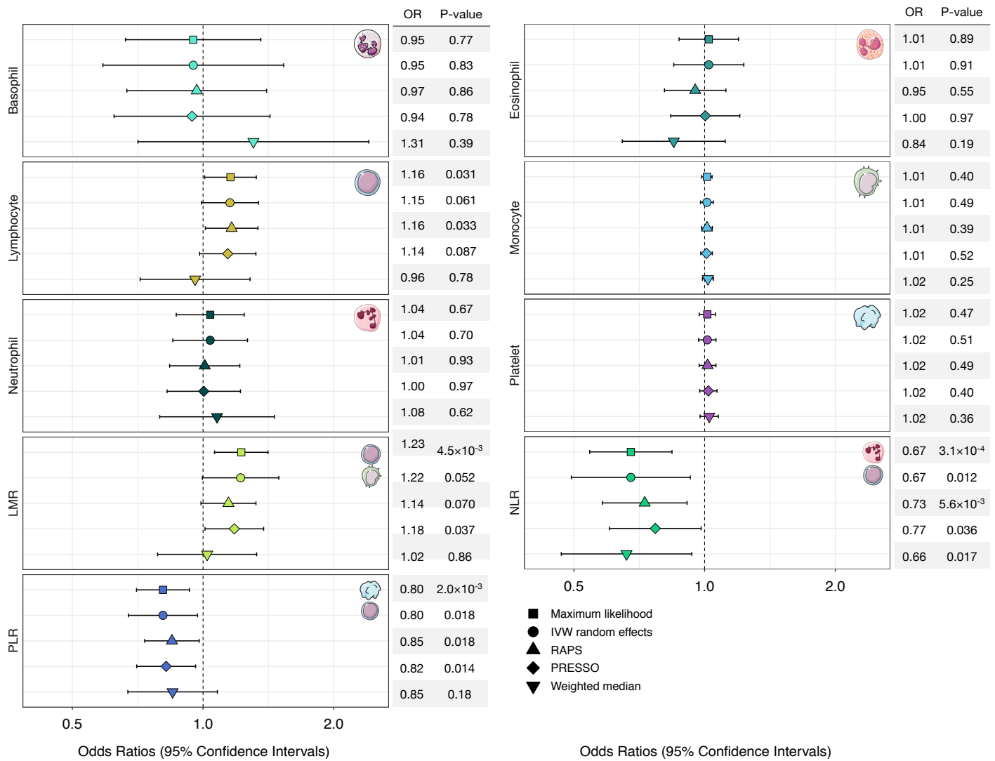
Figure 5: Odds ratios (OR) and 95% confidence intervals (CI) for the effect of increasing blood cell counts or cell type ratios on the risk of acute lymphoblastic leukemia (ALL), estimated using Mendelian Randomization (MR). Association results based on five different MR estimators are shown.
