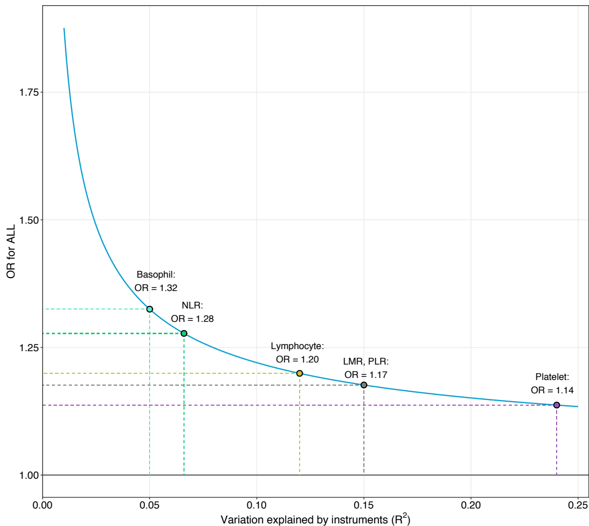
Supplementary Figure 5: Minimum detectable odds ratio at 80% power for each blood cell trait based on the observed instrument strength and available sample size for the outcome
