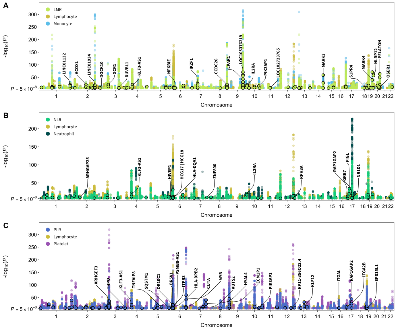
Figure 3: Genome-wide significant ( P < 5 \times 10^{-8} ) associations for cell type ratios and their component count traits. Points with black borders denote variants that were selected only as instruments for the given ratio trait and are not in linkage disequilibrium ( r^2 < 0.05 within 10Mb) with previously reported loci for its component cell type counts or proportions. Labeled genes contain variants with specific functional features (CADD score > 10 , Regulome DB rank 1-3a, missense mutations) and/or P < 1 \times 10^{-20} .
