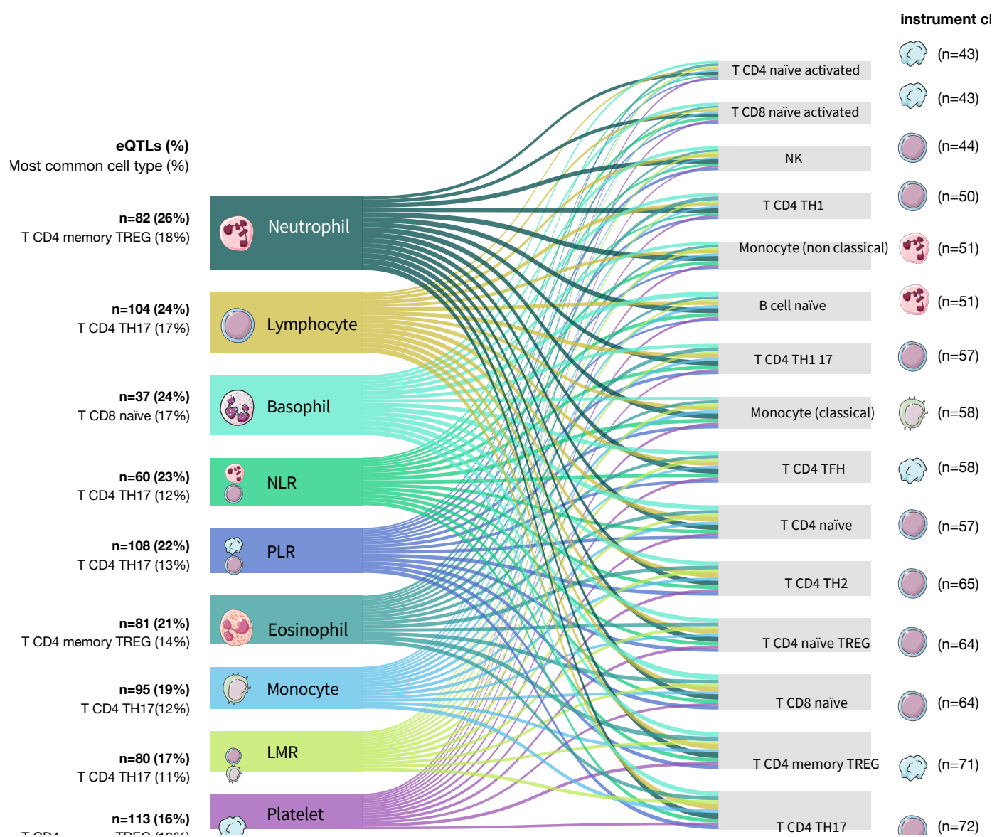
Supplementary Figure 2: Sankey style plot illustrating the pattern of cell-type specific effects on gene expression obtained from DICE (Database of Immune Cell Expression) for blood cell trait genetic instruments. Genetic instruments were considered expression quantitative trait loci (eQTL) if their associations with gene expression were significant at FDR < 0.05 . The color of each band corresponds to the blood cell type and the width of each band is scaled to reflect the proportion of all eQTL signals accounted for by a specific cell type.
