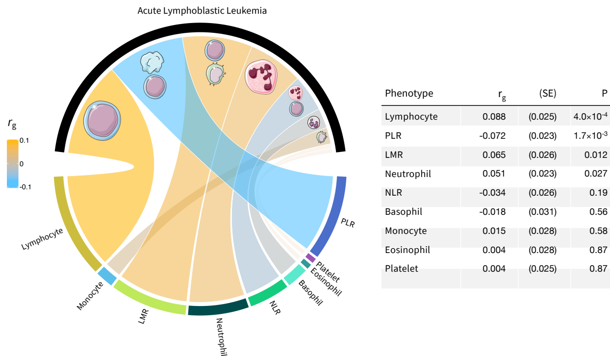
Figure 4: Genetic correlation ( r_g ) between blood cell subtypes and acute lymphoblastic leukemia (ALL) based on genome-wide summary statistics. The colors in the circos plot correspond to the direction of genetic correlation, with warm shades depicting positive correlations between increasing blood cell counts or ratios and ALL risk, cool tones corresponding to inverse associations, and faded gray shades corresponding to null correlations. The width of each band in the circos plot is proportional to the magnitude of the absolute value of the r_g estimate.
