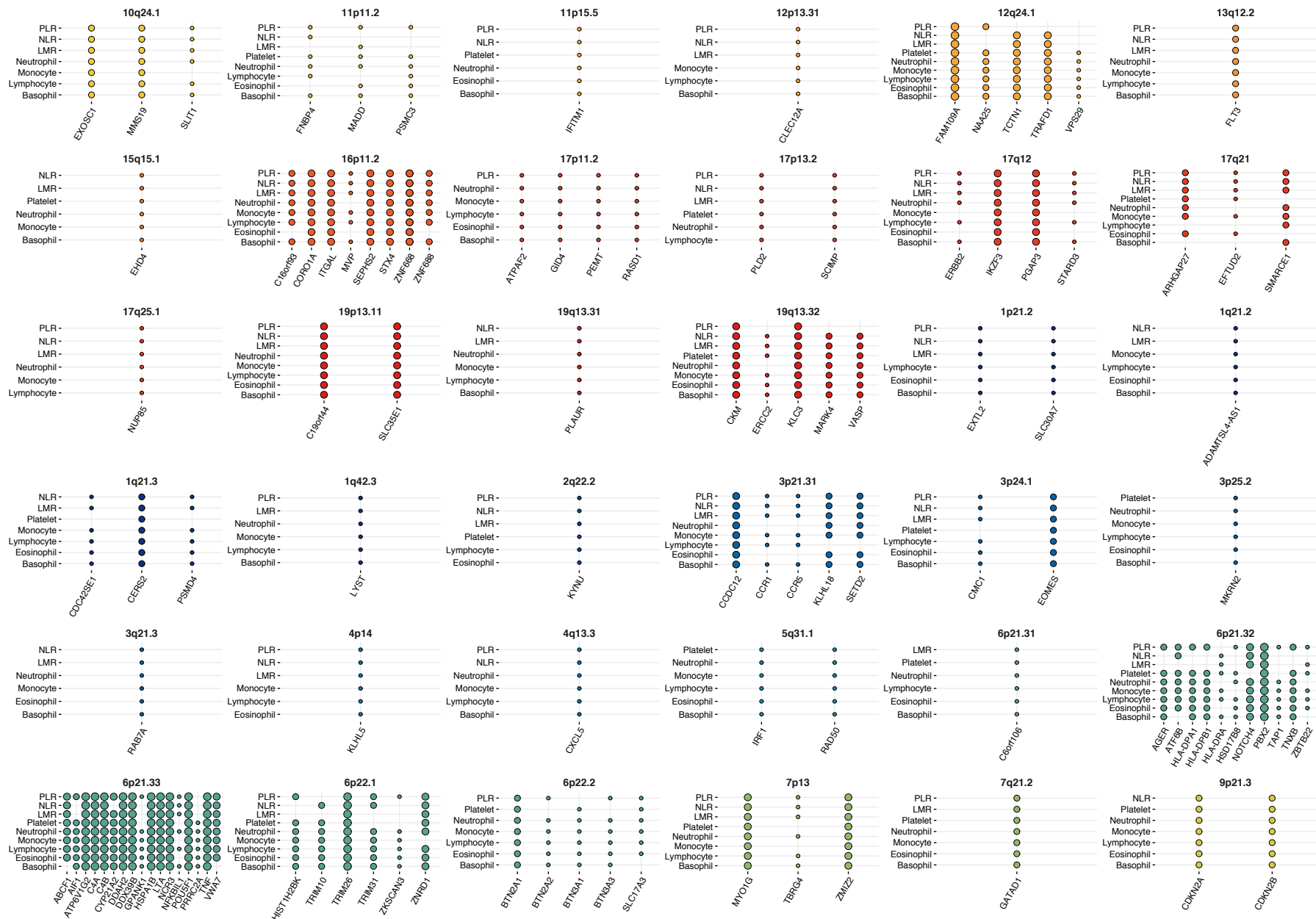
Supplementary Figure 4: Genes with expression trait loci (eQTL) in one cell type found among genetic instruments for >5 blood cell traits
