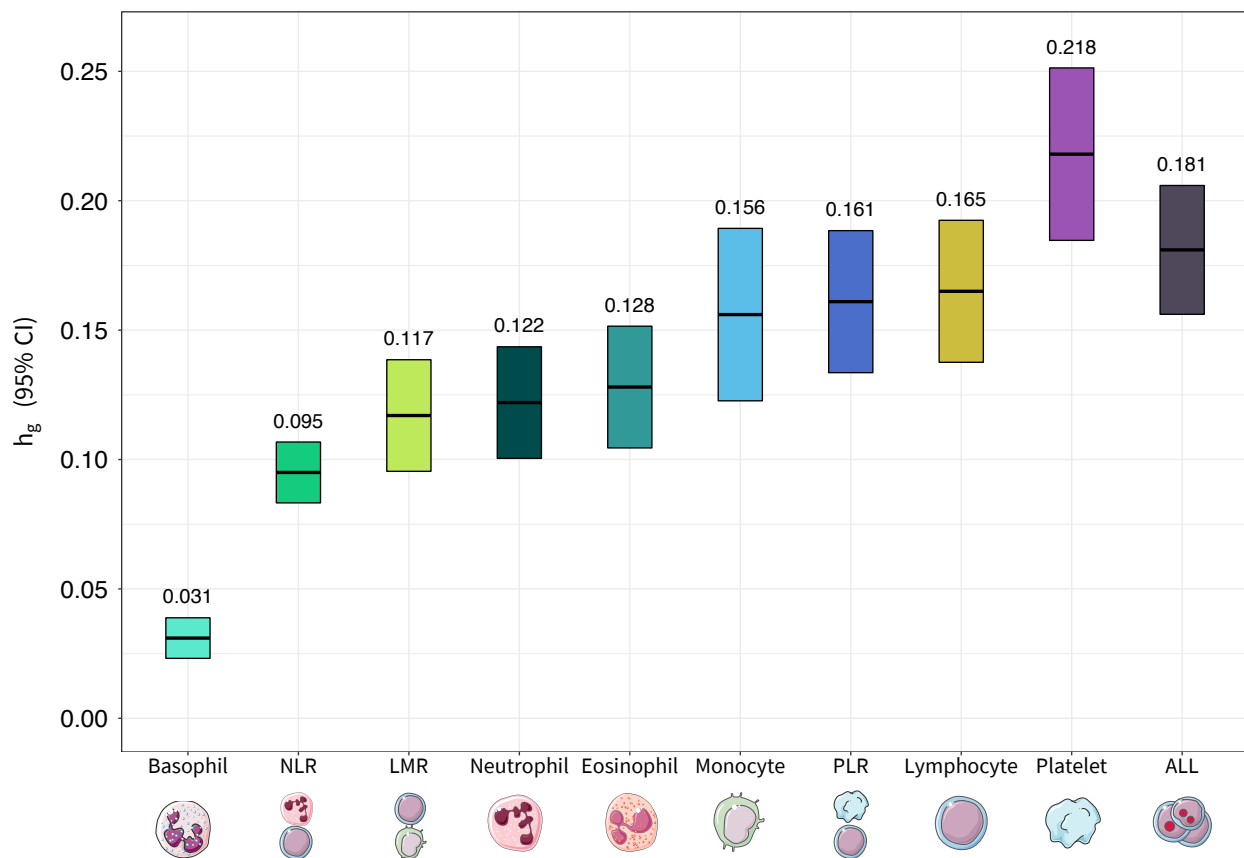
Figure 1: Array-based heritability ( h_g ) estimates for acute lymphoblastic leukemia (ALL) and blood cell subtypes: lymphocytes, monocytes, neutrophils, basophils, eosinophils, basophils, platelets, lymphocyte to monocyte ratio (LMR), neutrophil to lymphocyte ratio (NLR), and platelet to lymphocyte ratio (PLR) estimated using LD score regression.
