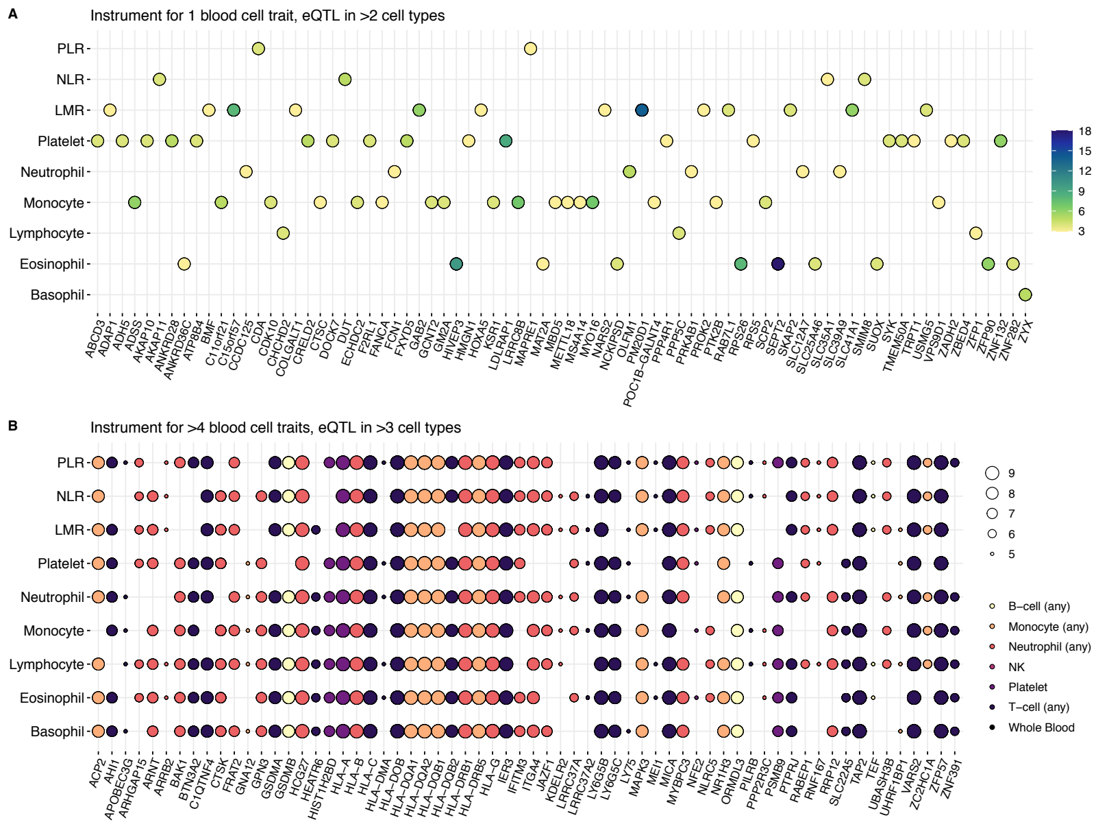
Supplementary Figure 3: Genes with expression trait loci (eQTL) in multiple cell types found among instruments for blood cell traits
