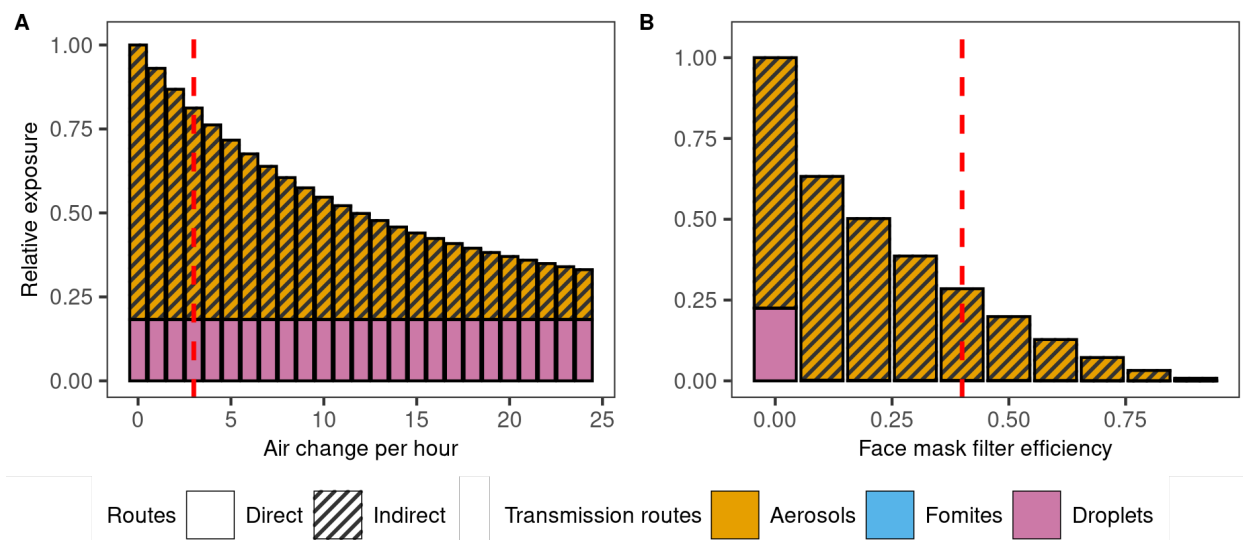
Fig 4. The impact of interventions on exposure after 15 minutes at a 1.5-metre distance.
