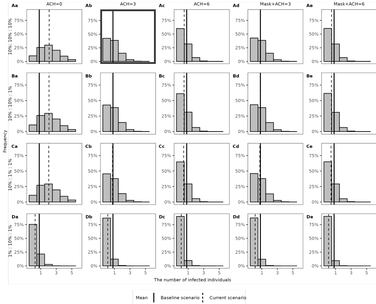
Fig 9. The density distributions of the expected number of infected individuals in the case study for varying route-specific transmission efficiency.
