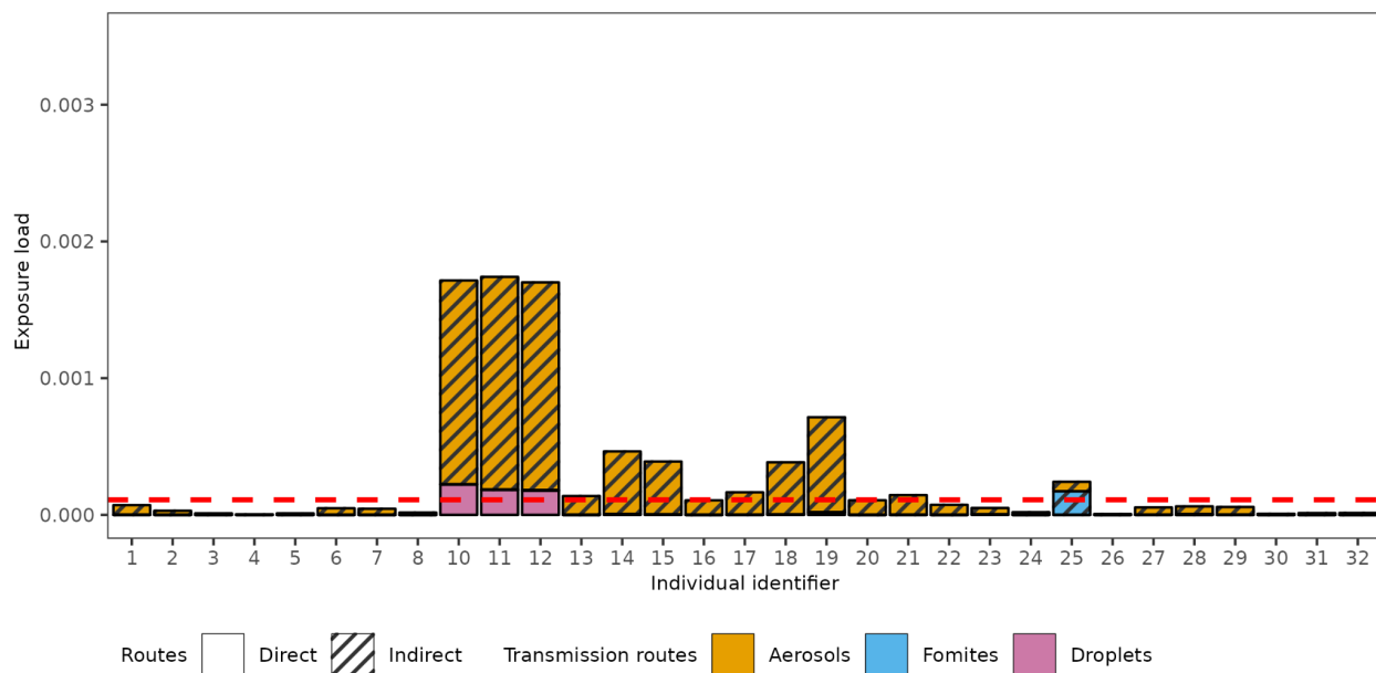
Fig 7. Susceptible individuals' exposure load.
