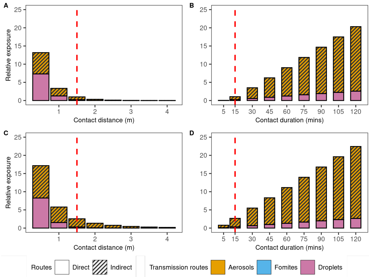
Fig 2. Effect of contact intensity on exposure and the relative contribution to exposure of transmission routes.
