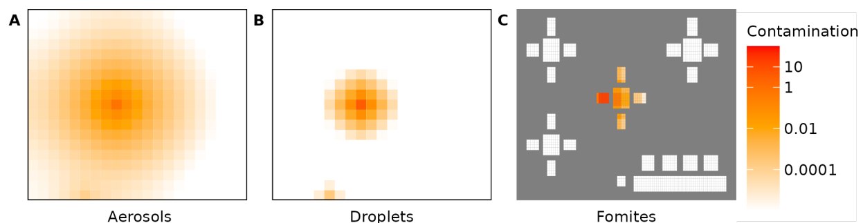
Fig 6. Cumulative virus contamination in the environment.
