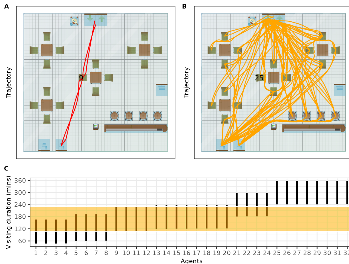
Fig 5. The trajectory, seat locations and the visiting duration of each individual in a simulation.
