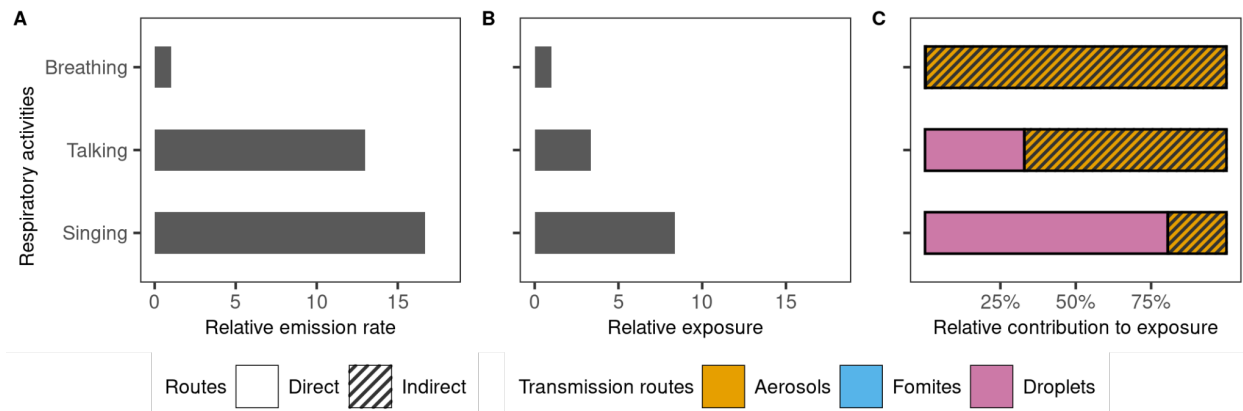
Fig 3. Effect of different respiratory activities on exposure.
