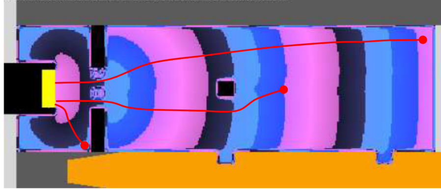
Fig 10. Illustrative floorfield Nomad with three resulting trajectories (Floorfield image from Campanella et al. (2009))
