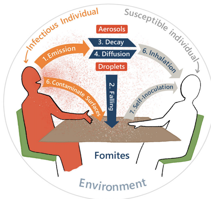
Fig 11. Schematic of processes in the epidemiological model.
