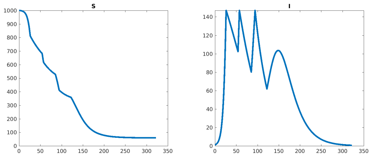
Figure 15: Plots of S(t) and I(t) (horizontal axis is time). Number of lockdowns: 3, peak I from formula: 146.957573, maximum of I on last (no lockdown) period: 103.506053. Lockdown start time(s): 26.22, 57.43, 94.30.
