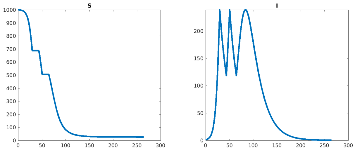
Figure 4: Plots of S(t) and I(t) (horizontal axis is time). Number of lockdowns: 2, peak I from formula: 238.740981, maximum of I on last (no lockdown) period: 238.755779. Lockdown start time(s): 29.73, 50.69.
