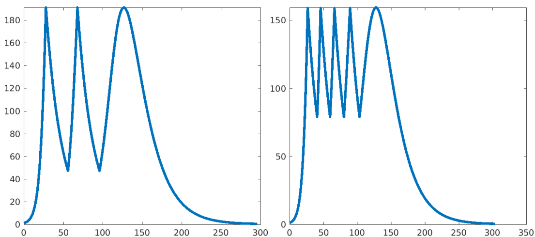
Figure 12: Left: two 28-day lockdowns. Right: four 14-day lockdowns. Parameters as earlier.
