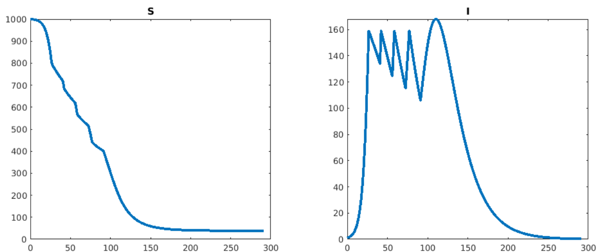
Figure 20: Plots of S(t) and I(t) (horizontal axis is time). Number of lockdowns: 4, peak I from formula: 158.980313, maximum of I on last (no lockdown) period: 167.977200. Lockdown start time(s): 26.74, 42.11, 58.60, 77.22.
