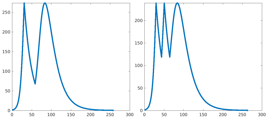
Figure 11: Left: one 28-day lockdown. Right: two 14-day lockdowns. Parameters as earlier.
