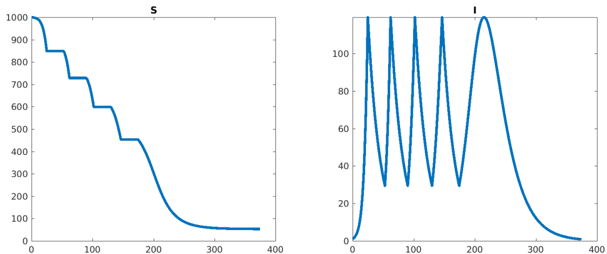
Figure 10: Plots of S(t) and I(t) (horizontal axis is time). Number of lockdowns: 4, peak I from formula: 119.371878, maximum of I on last (no lockdown) period: 119.395364. Lockdown start time(s): 24.91, 62.23, 101.98, 146.47.
