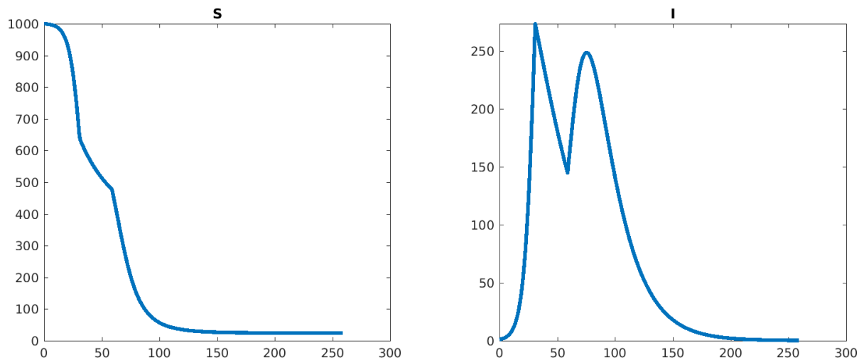
Figure 13: Plots of S(t) and I(t) (horizontal axis is time). Number of lockdowns: 1, peak I from formula: 273.247170, maximum of I on last (no lockdown) period: 248.383407. Lockdown start time(s): 30.90.
