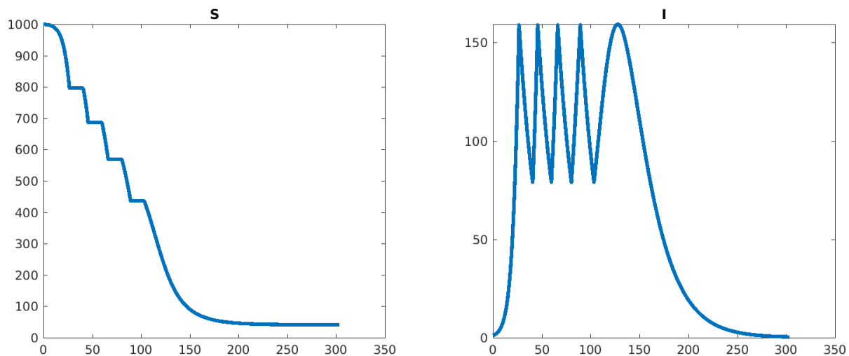
Figure 6: Plots of S(t) and I(t) (horizontal axis is time). Number of lockdowns: 4, peak I from formula: 158.980313, maximum of I on last (no lockdown) period: 159.342577. Lockdown start time(s): 26.74, 45.87, 66.33, 89.44.
