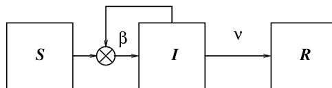
Figure 1: Diagram of standard SIR system
