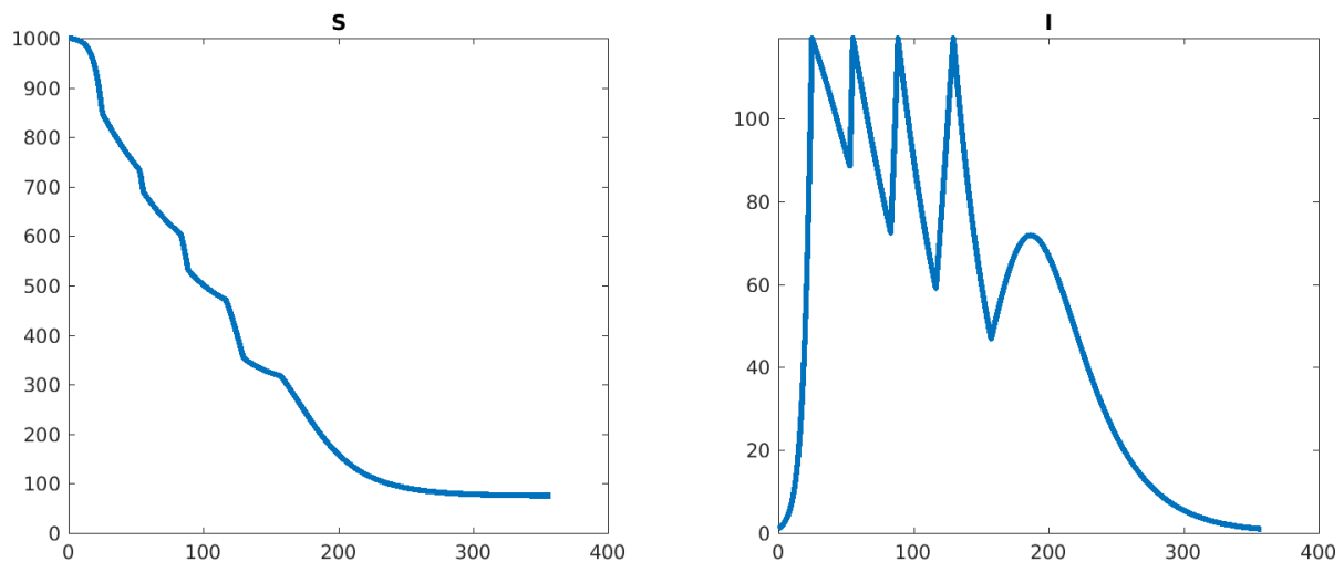
Figure 16: Plots of S(t) and I(t) (horizontal axis is time). Number of lockdowns: 4, peak I from formula: 119.371878, maximum of I on last (no lockdown) period: 71.792718. Lockdown start time(s): 24.91, 55.24, 88.63, 129.63.
