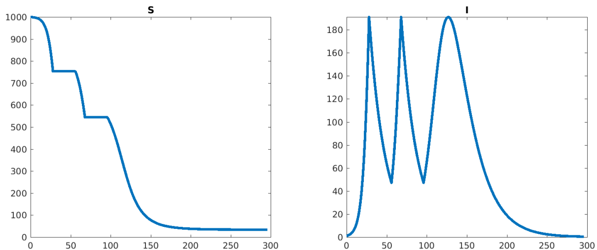
Figure 8: Plots of S(t) and I(t) (horizontal axis is time). Number of lockdowns: 2, peak I from formula: 191.124644, maximum of I on last (no lockdown) period: 191.048654. Lockdown start time(s): 28.02, 68.02.
