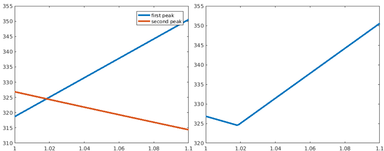
Figure 21: Left: Magnitude of first and second peak, with the lockdown time parametrized ( x axis) by the percentage of the ideal (perfect lockdown) formula. ; 14 day lockdown. Note that the second peak decreases as the first peak happens later, so the minimum of the maximum among them will occur when the curves intersect. Right: The maximum between the curves; minimum is around fraction 1.018 of the optimal for perfect lockdowns, so trigger should occur later.
