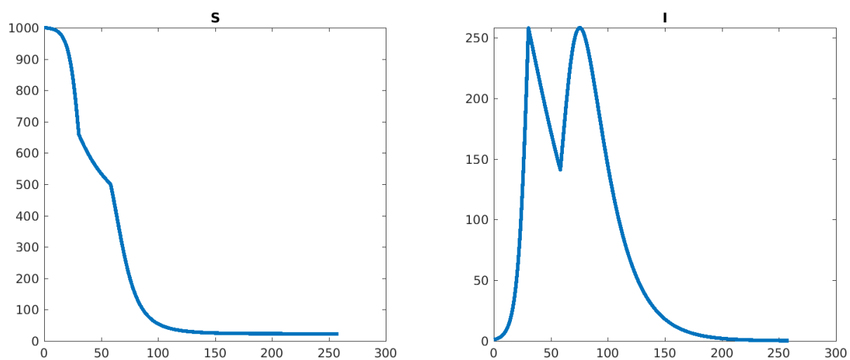
Figure 24: Simulation with an imperfect lockdown. Using now the optimal fraction 0.944 of the optimal for perfect lockdowns, obtained by minimizing the plot in Figure 23 (right). The optimal peak value is now approximately 258, which can be compared with the suboptimal plot (using the formula that assumed perfect lockdowns) shown in Figure 13, which had a peak of approximately 273. Observe how the two peaks are now balanced. The optimal result is very close to the one obtained from our formulas.
