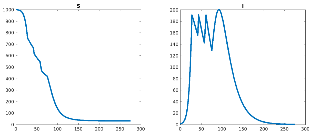
Figure 19: Plots of S(t) and I(t) (horizontal axis is time). Number of lockdowns: 3, peak I from formula: 190.862880, maximum of I on last (no lockdown) period: 200.218534. Lockdown start time(s): 28.01, 43.86, 61.6.
