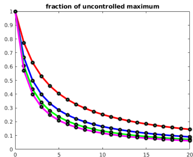
Figure 2: Percentage of virtual peak when using K lockdowns (horizontal axis) each of them 7 (red), 14 (blue), 21 (green), or 28 (magenta) days long.
