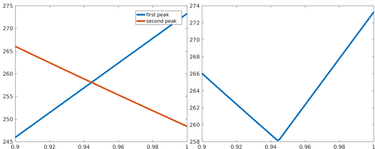
Figure 23: Left: Magnitude of first and second peak, with the lockdown time parametrized ( x axis) by the percentage of the ideal (perfect lockdown) formula; 14 day lockdown. Note that the second peak decreases as the first peak happens later, so the minimum of the maximum among them will occur when the curves intersect. Right: The maximum between the curves; minimum is around fraction 0.944 of the optimal for perfect lockdowns, so trigger should occur earlier.
