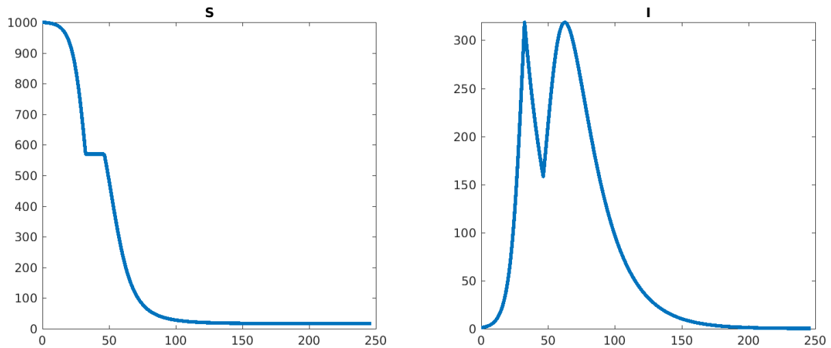
Figure 3: Plots of S(t) and I(t) (horizontal axis is time). Number of lockdowns: 1, peak I from formula: 318.682808, maximum of I on last (no lockdown) period: 318.601530. Lockdown start time(s): 32.42.
