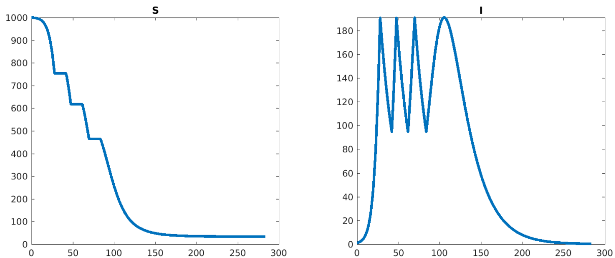
Figure 5: Plots of S(t) and I(t) (horizontal axis is time). Number of lockdowns: 3, peak I from formula: 190.862880, maximum of I on last (no lockdown) period: 191.019085. Lockdown start time(s): 28.01, 47.71, 69.80.
