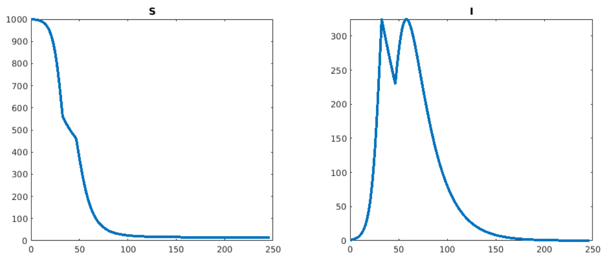
Figure 22: Simulation with an imperfect lockdown. Using now the optimal fraction 1.018 of the optimal for perfect lockdowns, obtained by minimizing the plot in Figure 21 (right). The optimal peak value is now approximately 324, which can be compared with the suboptimal plot (using the formula that assumed perfect lockdowns) shown in Figure 17, which had a peak of approximately 327. Observe how the two peaks are now balanced. The optimal result is not that different from the one obtained from our formulas, and the lockdown start is at time 30.39.
