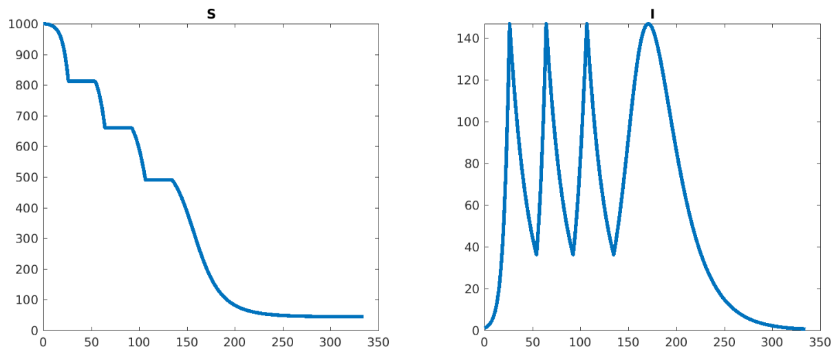
Figure 9: Plots of S(t) and I(t) (horizontal axis is time). Number of lockdowns: 3, peak I from formula: 146.957573, maximum of I on last (no lockdown) period: 146.913773. Lockdown start time(s): 26.22, 64.39, 106.74.
