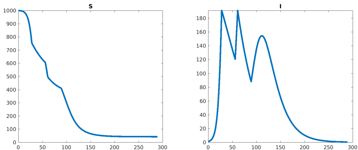
Figure 14: Plots of S(t) and I(t) (horizontal axis is time). Number of lockdowns: 2, peak I from formula: 191.124644, maximum of I on last (no lockdown) period: 154.387915. Lockdown start time(s): 28.02, 61.2.
