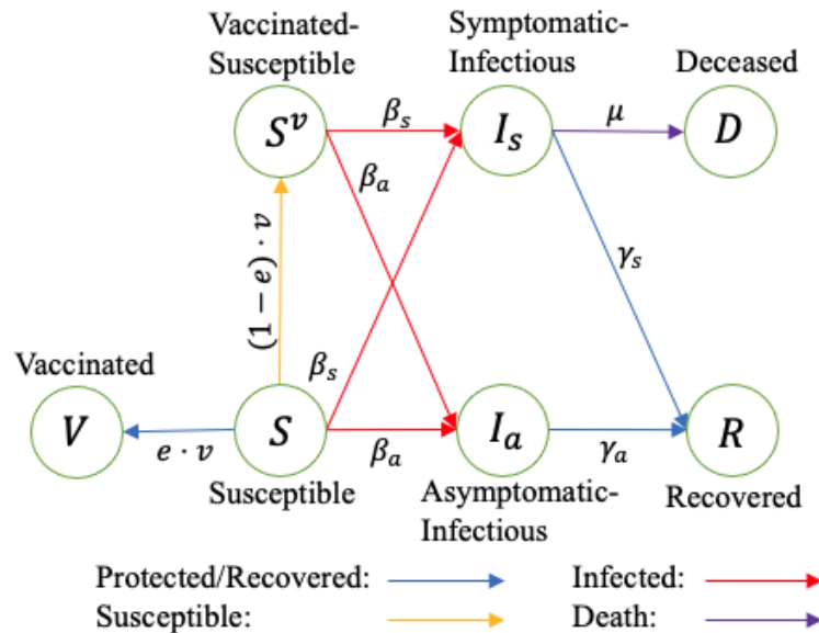
132 Figure 1: Transition diagram of the extended SIR-D model, in which each move is dependent on 133 the epidemiological and vaccine parameters; \beta_s symptomatic and asymptomatic 134 transmission rates, respectively; \beta_a : symptomatic and asymptomatic recovery rates, 135 respectively; \mu : decrease rate of a symptomatic patient; e \cdot v : efficacy of the vaccine; (1 - e) \cdot v 136 ratio of the daily vaccine capacity to the size of the unvaccinated susceptible population (i.e., 137 )
