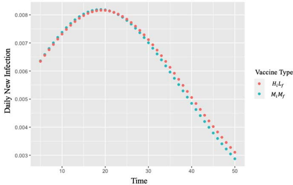
217 218 219 Figure 4: Daily new infections from day 5 to day 50 with vaccine- and vaccine- when 220 the capacity multiplier ( is 3 and the mutation time is day 5
