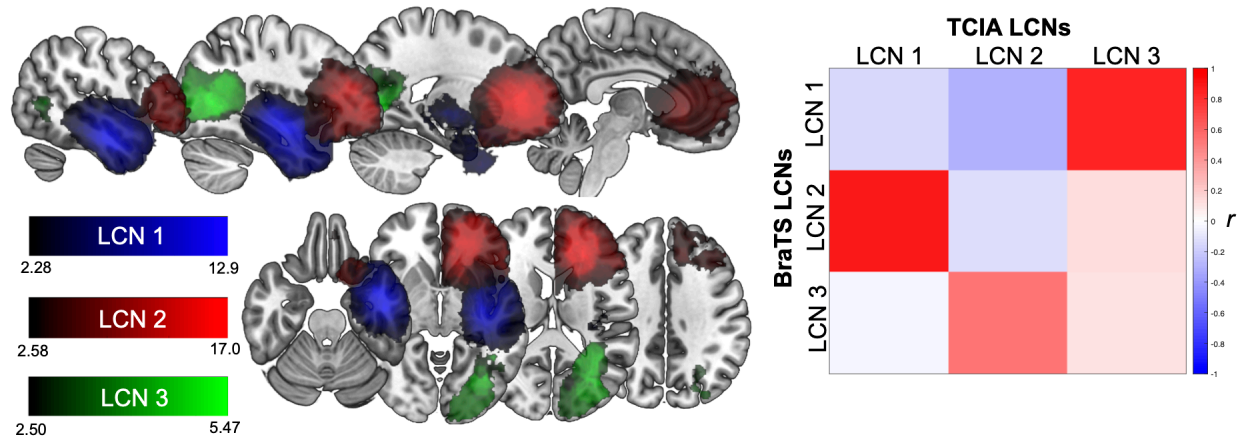
Supplementary Figure 1. Replication of lesion covariance networks in an independent cohort. (A) LCNs derived from a cohort of 168 high- and low-grade glioma patients displayed on the same slices shown in Figure 1. (B) Correlation matrix illustrating the correspondence between LCNs in the TCIA and BraTS cohorts. Abbreviations: TCIA = The Cancer Imaging Archive; BraTS = Brain Tumor Segmentation Challenge.
