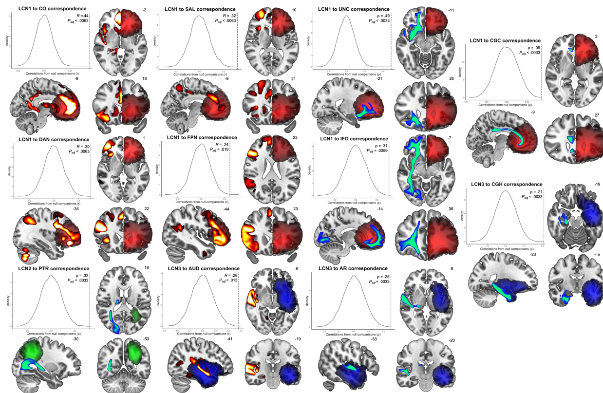
Supplementary Figure 3. Functional and structural connectivity networks significantly associated with lesion covariance networks.
