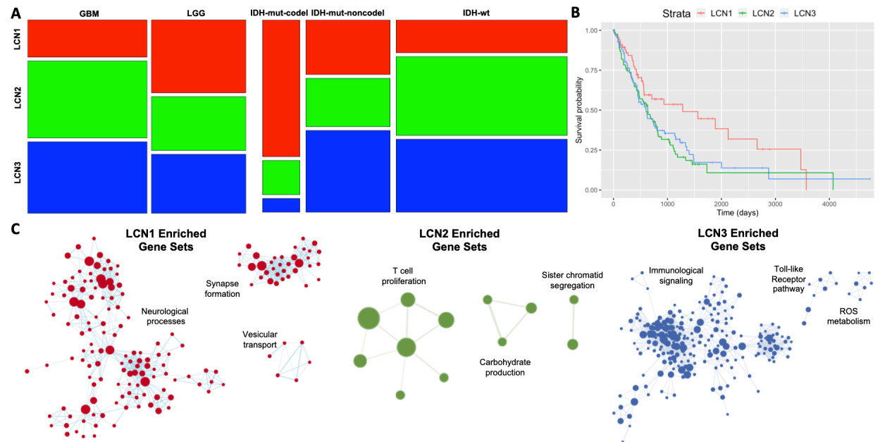
Figure 2. Clinical and genomic correlates of lesion covariance networks. (A) Mosaic plots represent the proportion of gliomas within each LCN associated with clinical variables, including tumor grade and molecular subtype. (B) Kaplan-Meier curves show overall survival outcomes stratified by LCN group. (C) Gene ontology networks associated with differentially-expressed genes for each LCN. Enriched gene sets are plotted as nodes, with gene set size proportional to node size, and the similarities between gene sets are represented as edges. Network components with the three highest numbers of nodes are displayed.
