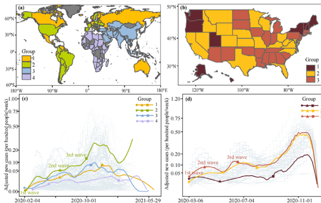
Fig. 1. Data context. The different groups in (a) and (b) were determined by pandemic parameters and geographic proximity (see SI for more information). (c) - (d) The pandemic trajectories of weekly reporting cases for each country/state (background polylines) and group (solid curves). The solid curves for each group are mean weekly cases across countries/states in that group. Starting points (represented by different marks) of different waves in each group are generally illustrated by their mean starting dates which were quantitatively defined in this study.
