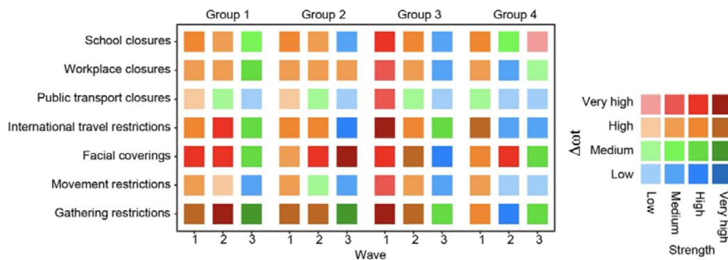
Fig. 3. The cross-wave and cross-group effects of individual NPIs. Effects of individual NPIs on reducing the transmission of COVID-19 across waves and groups are illustrated by different colours associated with their average implementation strength. The dark colour indicates higher strength, while the NPIs effects increased from low level (blue) to high level (red). A full list of countries and the corresponding time frames of different waves for each group can be found in SI Table C2 – C5.
