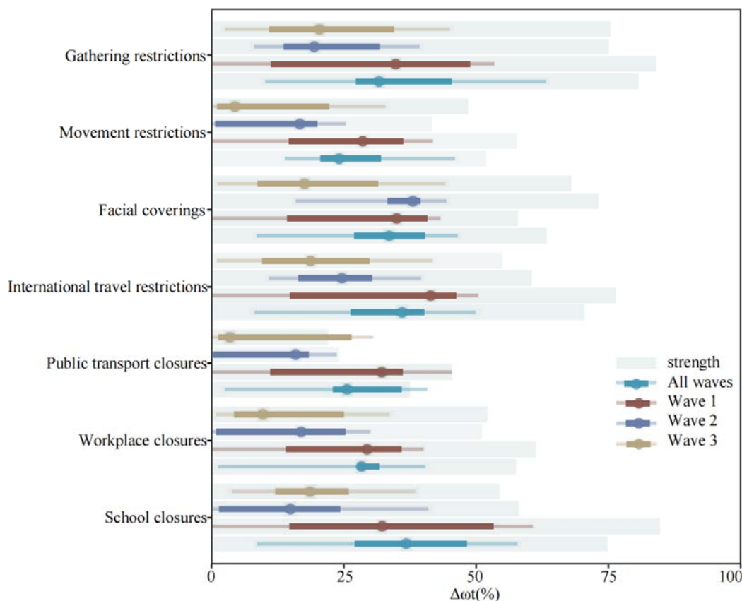
Fig. 2. Effects of individual NPIs on reducing the transmission of COVID-19 across waves within our data context. The coefficients ( \alpha_i ) of NPIs parameters in different periods were calibrated by the default model setting with corresponding data contexts. The effect estimates were calculated by the coefficients of NPIs through 1 - \exp(-\alpha_i \bar{x}_i) , where \bar{x}_i is the average strength of NPI implementation (represented by the background shadow). We rescaled the average strength by multiplying 100 to adapt the x-axis. The synergistic effectiveness of all NPIs (All waves: 92.3%, Wave 1: 95.4%, Wave 2: 79.9%, Wave 3: 56.0%) were nonlinear cumulative in terms of the individual effect by 1 - \prod_{x_i} \exp(-\alpha_i \bar{x}_i) . The effect over all waves represents the average performance of NPIs against COVID-19 in 133 countries (Fig. 1(a)) before their vaccination by 22 June 2021. Wave 1 refers to the average performance of NPIs against COVID-19 in the first wave of the 133 countries. The specific periods of the first wave in 133 countries are not fully consistent, meaning that the first wave does not refer to a particular time but a general period of the first outbreak. The second
