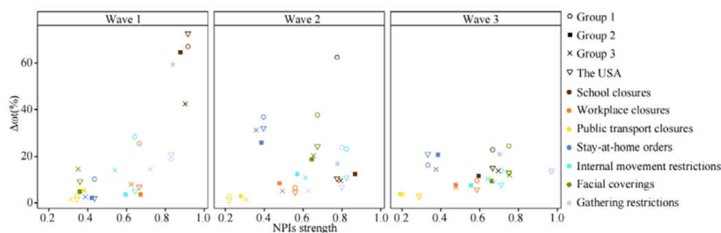
Fig. 4. The individual efficacy estimates of the seven NPIs for the USA and its subnational regions. Different NPIs are represented by different colours. The groups as well as the USA are demonstrated by different symbols. Full lists of states name in each group as well as their defined wave periods can be found in SI Table C6- C8.
