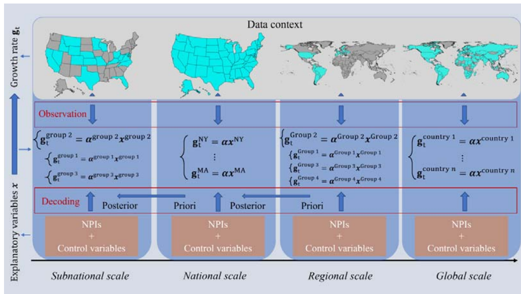
Fig. 5. The conceptual framework. We used growth rate as the outcome variable to describe the trajectory of the pandemic. The empirical changes of growth rate were decoded into the effectiveness of both NPIs as well as the control variables.
