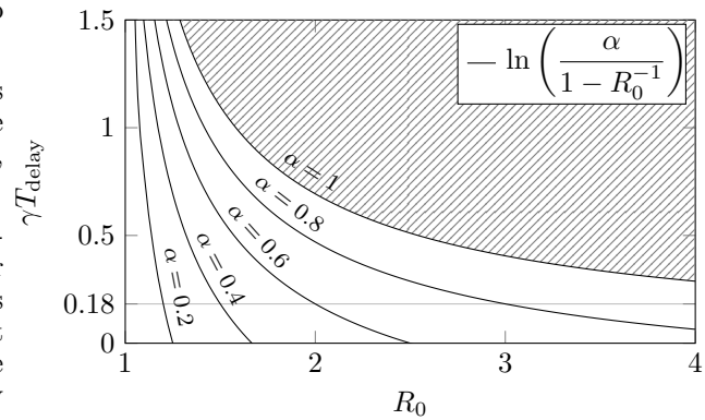
Fig. 2. Illustration of the stability boundary for the model in (1)–(2). The model is stable if and only if (R_0, \gamma T_{\text{delay}}) lies below the corresponding \alpha curve. That is, at least a proportion \alpha of persons becoming infectious on a particular day need to be isolated T_{\text{delay}} days later, given a natural recovery rate is \gamma days ^{-1} .
