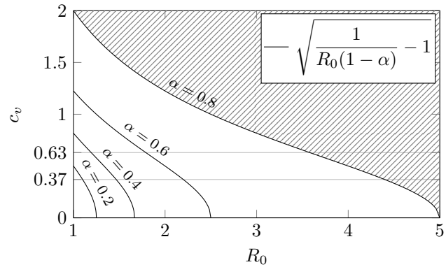
Fig. 3. Illustration of maximum admissible coefficient of variance c_v for stabilization using the case isolation scheme (2) early in an epidemic (when S \gg I ). In this example, we assume that a proportion \alpha of the infectious population are isolated without delay ( T_{\text{delay}} = 0 ). The figure illustrates, for different \alpha , the relation between the basic reproduction number R_0 of a corresponding homogeneously interacting population (in absence of case isolation), and the admissible c_v . The shaded curve shows what combinations of R_0 and c_v cannot be stabilized for \alpha = 0.8 . The horizontal lines at c_v = 0.37 and c_v = 0.67 represent bounds on c_v for human infectious disease transmission networks reported in Salathé et al. (2010).
