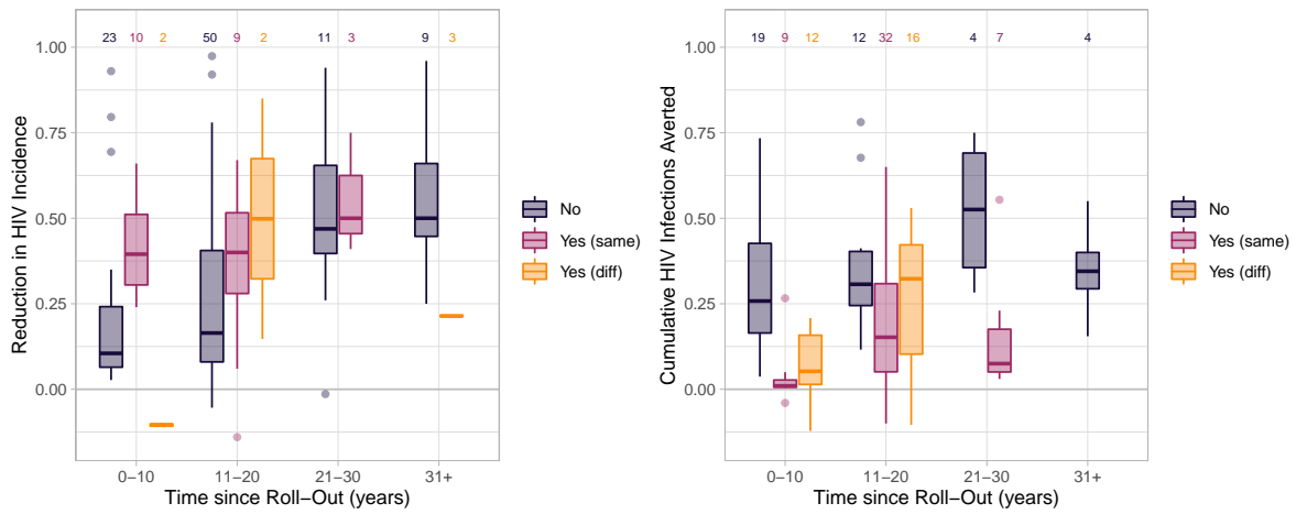
Figure C.13: Sex stratification & any ART cascade differences
