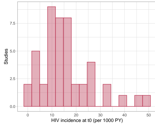
Figure C.3: HIV incidence at t_0 (per 1000 PY)
