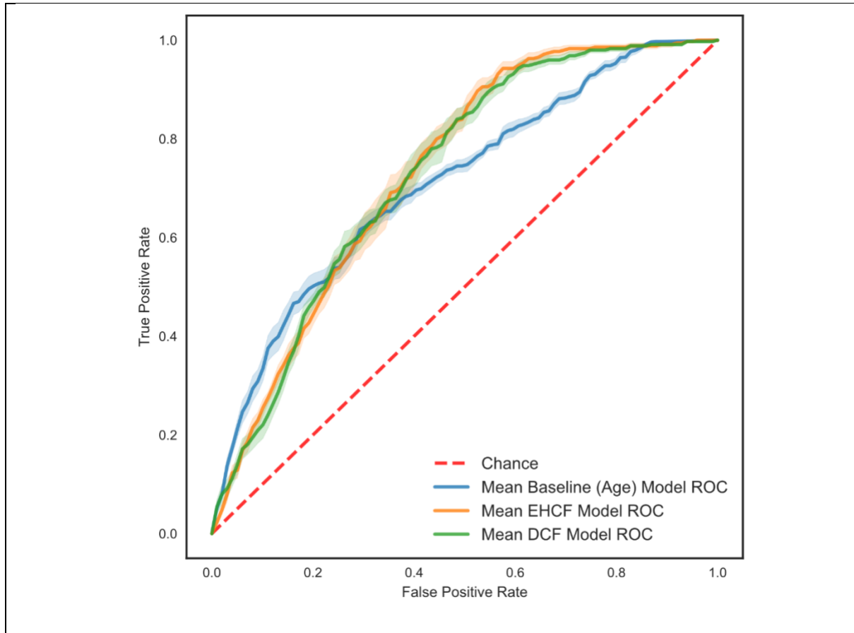
Figure 5. Mean receiver operating characteristic curves derived from predicting COVID-19-related death in the 10-Fold Cross Validation (standard error of the mean) for all models.
