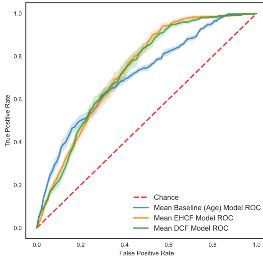
Figure 5. Mean receiver operating characteristic curves derived from predicting COVID-19-related death in the 10-Fold Cross Validation (standard error of the mean) for all models.
