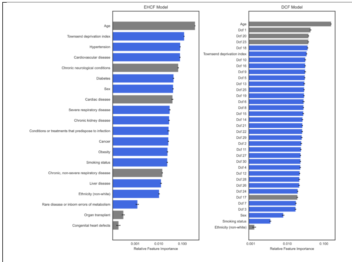
Figure 6. Comparison of relative feature importance (note logarithmic scale) showing the contribution to the predictions of the EHCF and our DCF Model. In grey the demographic and lifestyle features which were the same in both models and in blue the model specific features. Note, how in the DCF Model aside from age the co-morbidity and multi-morbidity make up the key 15 features.
