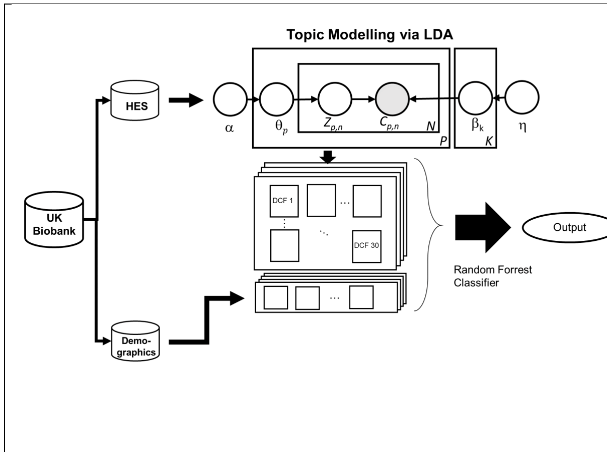
Figure 7. Illustration of the overall study design for the DCF Model. First, we separate the UK Biobank into HES and demographic data, we generate the features (using LDA) from the discrete input of the HES database. We subsequently use the distribution of each patient over these features as input to a supervised random forest classifier to predict COVID-19 fatality.
