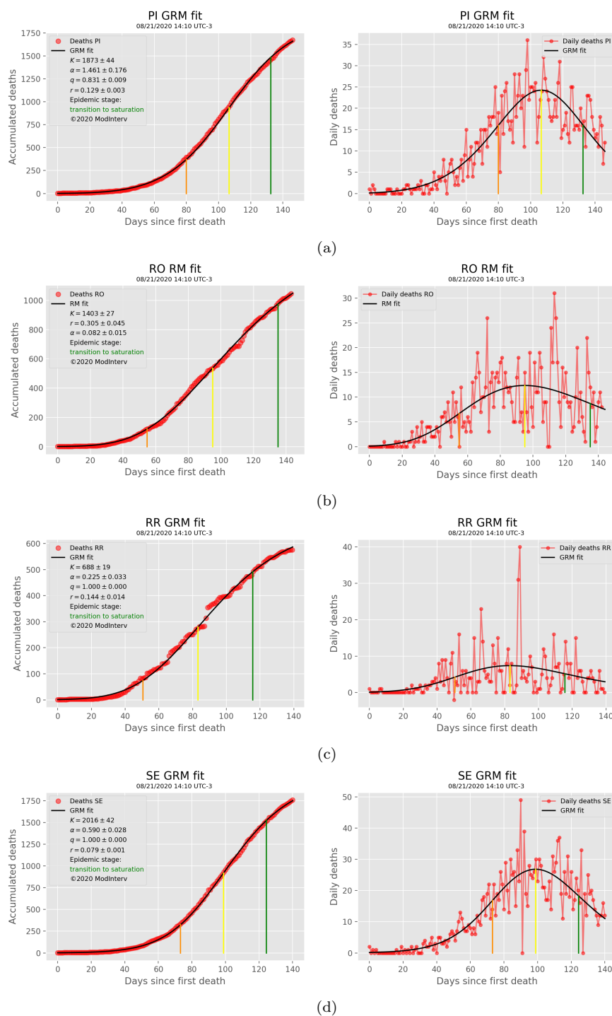
Fig. 8: States in the transition to saturation stage - II.
