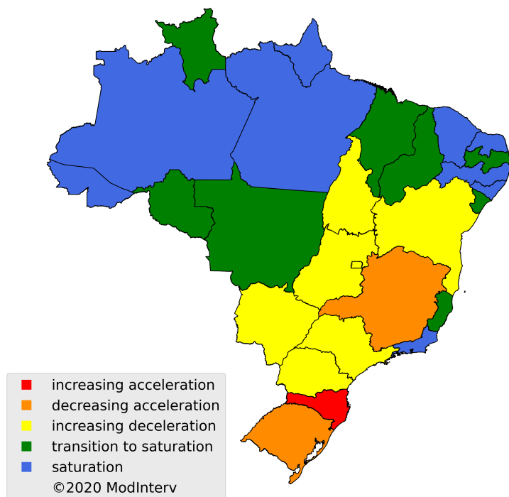
Fig. 2: Situation of the COVID-19 epidemic in the Brazilian States and Federal District, on August 21, 2020, according to the classification of the epidemic stages implemented in the ModInterv application.
