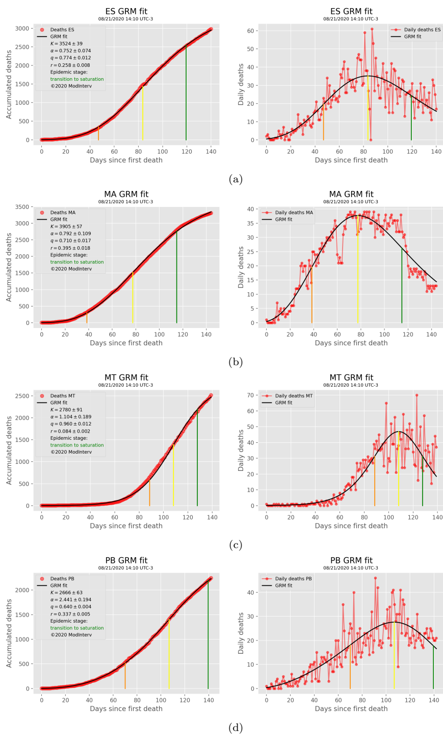
Fig. 7: States in the transition to saturation stage - I.
