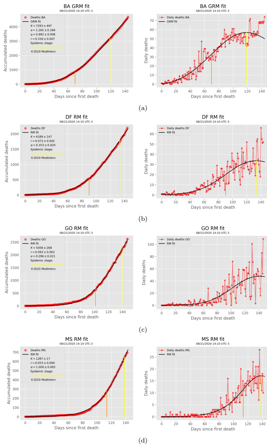
Fig. 5: States in the stage of increasing deceleration - I.
