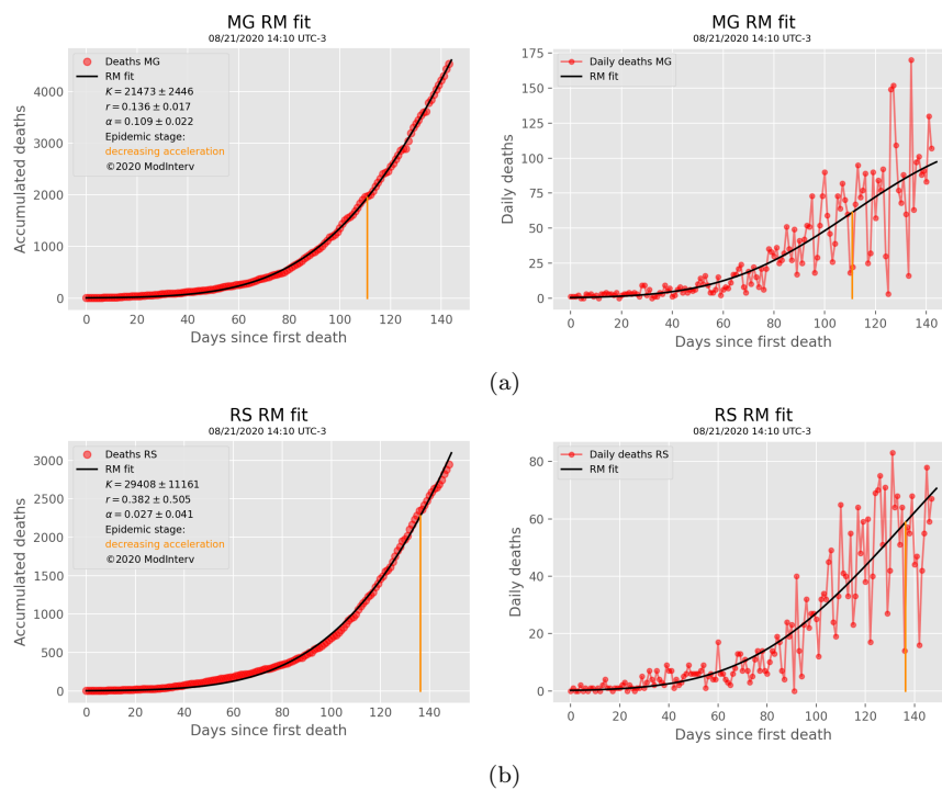
Fig. 4: States in the stage of decreasing acceleration.
