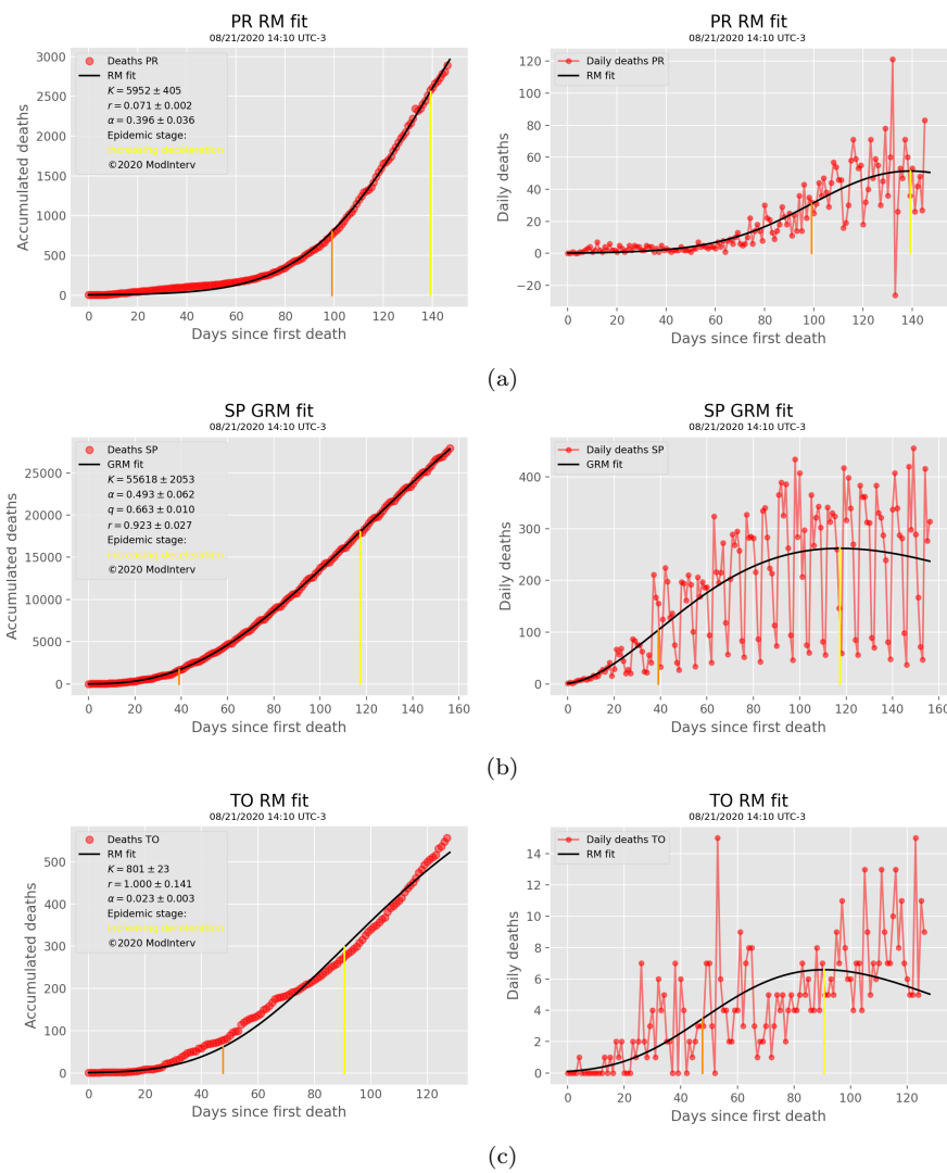
Fig. 6: States in the stage of increasing deceleration - II.
