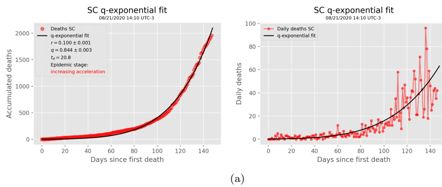
(a) Fig. 3: State in the stage of increasing acceleration.
