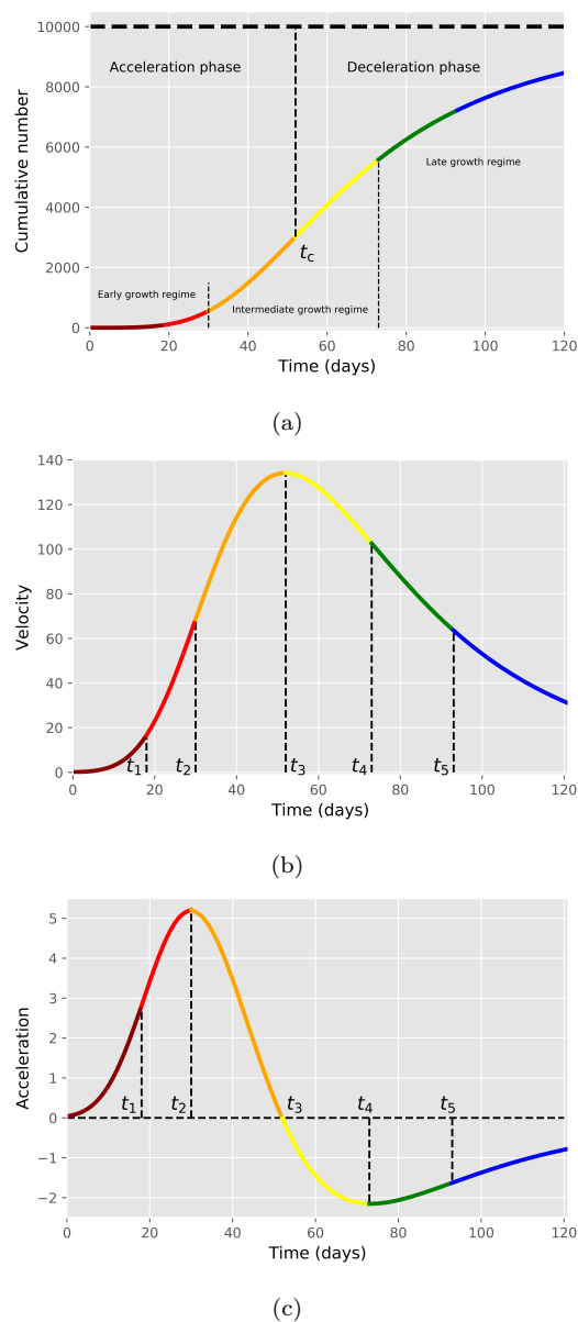
Fig. 1: (a) Schematic of an epidemic curve for the cumulative number of deaths, with an indication of its two main phases, namely, the acceleration and deceleration phases, respectively. The point t_c indicates the inflection point of the cumulative curve, where the acceleration is zero, which separates the two phases. (b) Velocity and (c) acceleration curves, corresponding to the first and second derivatives, respectively, of the cumulative curve shown in (a). The different colors in the three curves indicate the respective epidemic stages, according to the corresponding acceleration regimes; see text.
