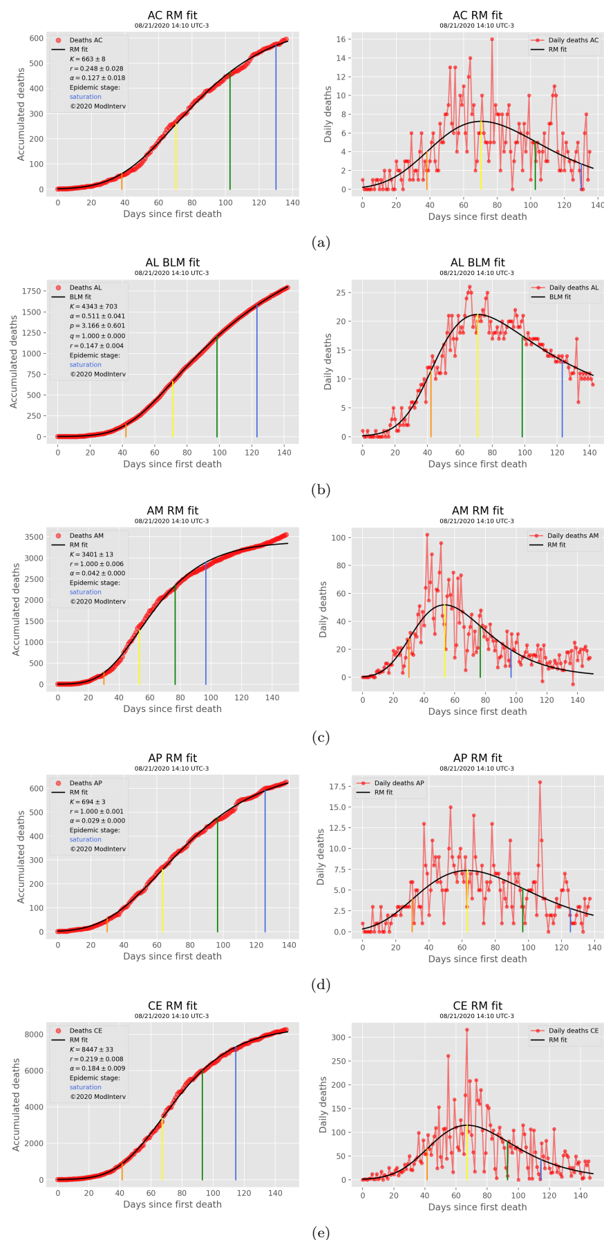
Fig. 9: States in the saturation stage - I
