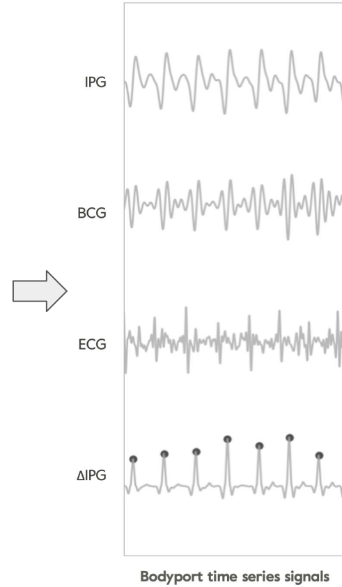
Figure 1: Left: Image of the Bodyport Cardiac Scale. Right: Example of scale-derived signals for the impedance plethysmograph (IPG), ballistocardiograph (BCG), electrocardiograph (ECG), and derivative of the IPG ( \Delta IPG).
