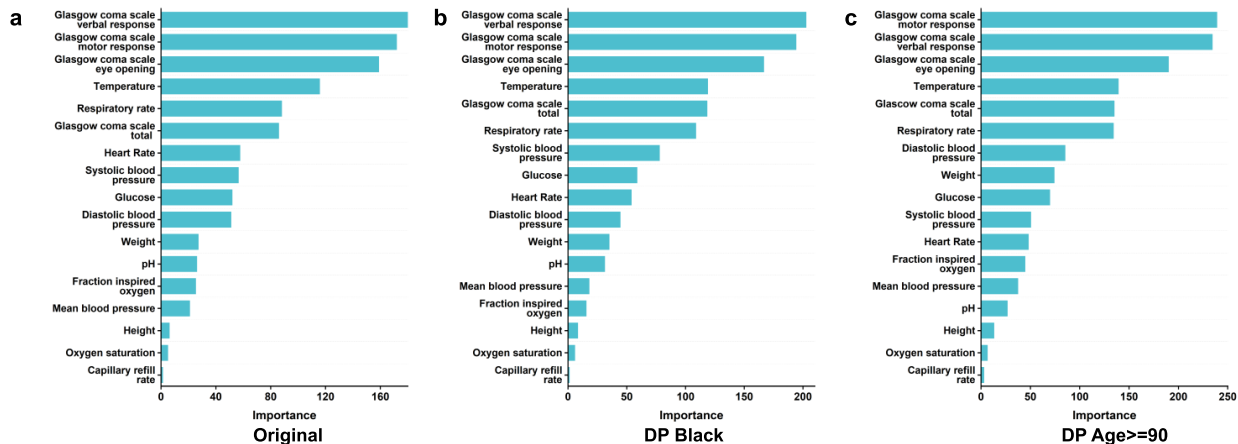
Supplementary Figure 19: SHAP-sum feature importance of different IHM experiments. Original stands for the original machine learning model without any bias correction. DP stands for our Double Prioritized sampling method. In SHAP-sum, the importance of columns representing the same variable is summed up. Feature importance for the IHM prediction in (a) original model, (b) DP model for Black patients, and (c) DP model for age>=90 patients.
