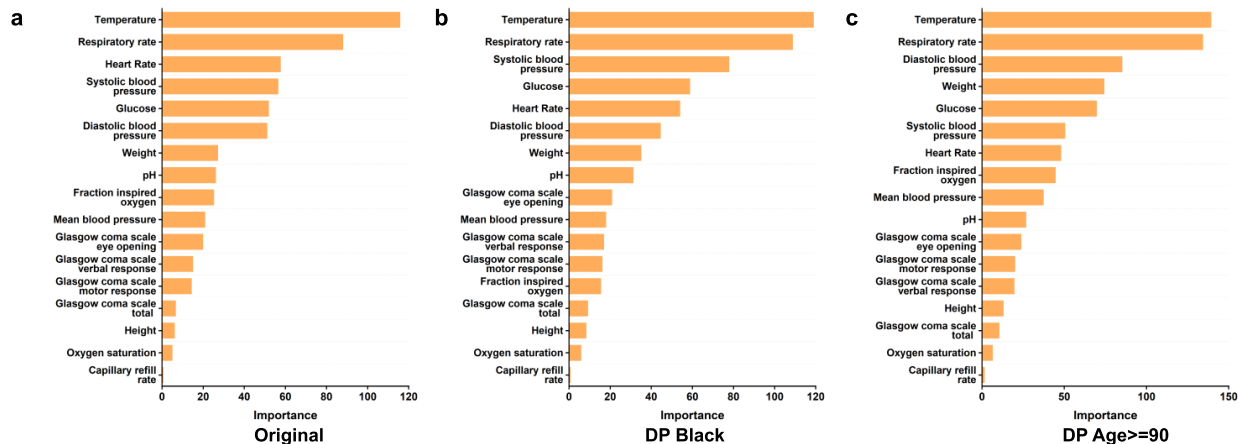
Supplementary Figure 17: SHAP-avg feature importance of different IHM experiments. Original stands for the original machine learning model without any bias correction. DP stands for our Double Prioritized sampling method. In SHAP-avg, the importance of columns representing the same variable is averaged. Feature importance for IHM prediction in (a) original model, (b) DP model for Black patients, and (c) DP model for age >=90 patients.
