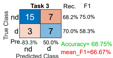
Figure 3: Task 3: Decision fusion of the best results of acoustic and linguistic features on the test set.
