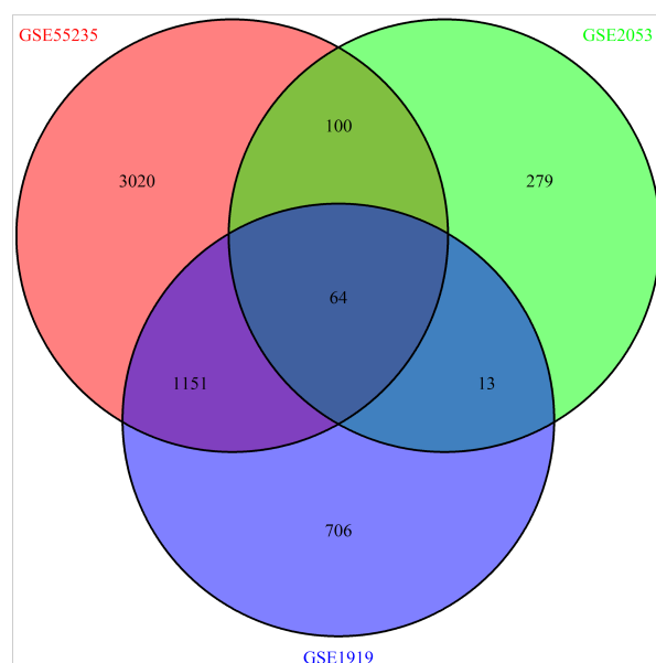
Figure 4: The Venn diagram shows the number of genes that are shared between GSE55235, GSE2053, and GSE1919. 64 genes were differentially expressed in all three sets.
