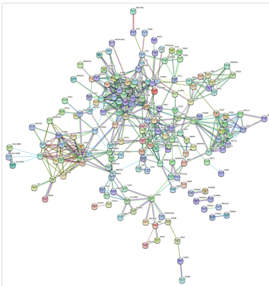
Figure 5: STRING network of protein interactions between 292 DEGs.
