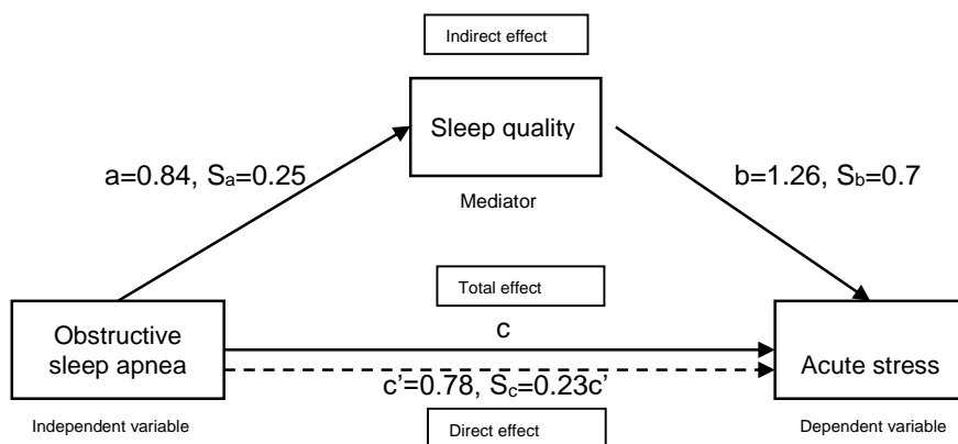
323 Figure 2 Mediation model with effect size.
