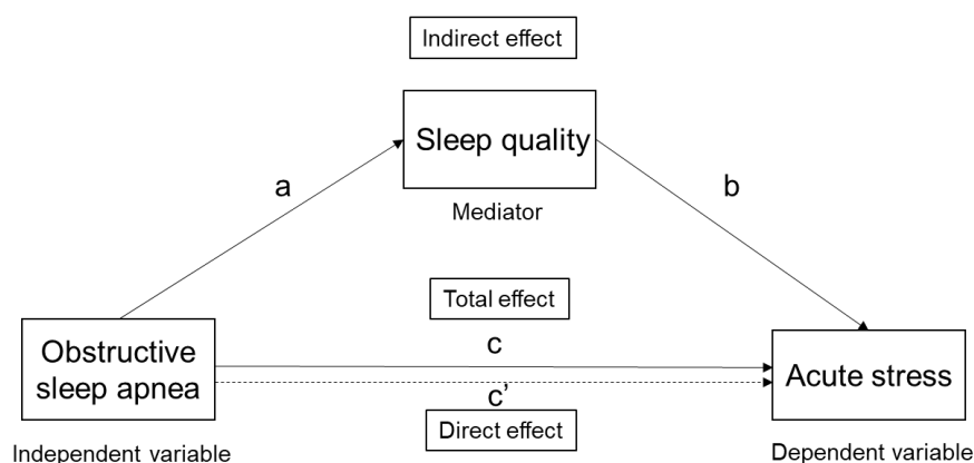
320 Figure 1 Mediation model
