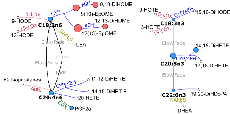
768 Figure 2. CSF differences in fatty acids-derived oxylipins and endocannabinoids, between control 769 and AD group, projected on their metabolic pathway.
