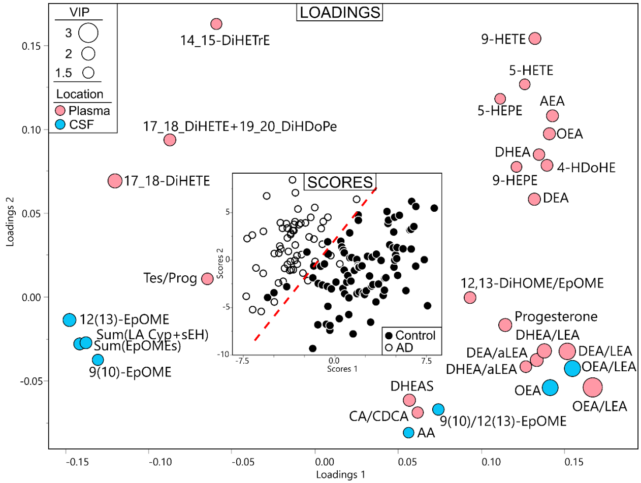
783 Figure 3. Relation between plasma and CSF predictors of AD
